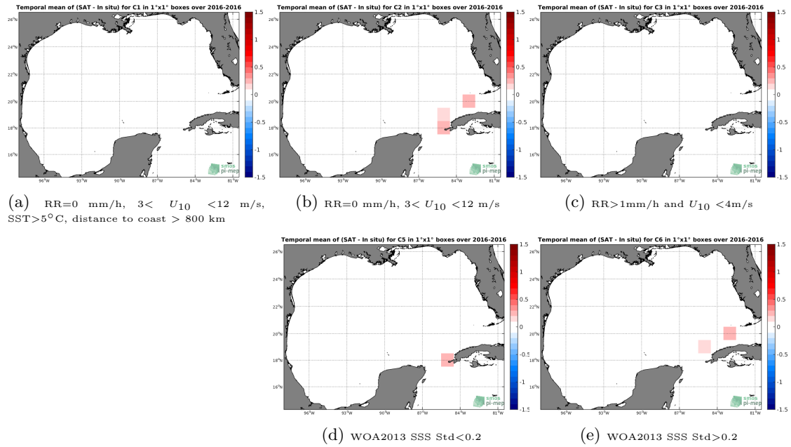
Figure 12: Temporal mean gridded over spatial boxes of size 1^\circ \times 1^\circ of \Delta SSS (SMOS-L3-CATDS-CECOS-LOCEAN-V4-9DAYS-25KM - TSG-LEGOS-DM) for 5 different subdatasets corresponding to:RR=0 mm/h, 3 < U_{10} < 12 m/s, SST >5^\circ\text{C} , distance to coast > 800 km (a), RR=0 mm/h, 3 < U_{10} < 12 m/s (b), RR >1 mm/h and U_{10} < 4 m/s (c), WOA2013 SSS Std <0.2 (d), WOA2013 SSS Std >0.2 (e).
