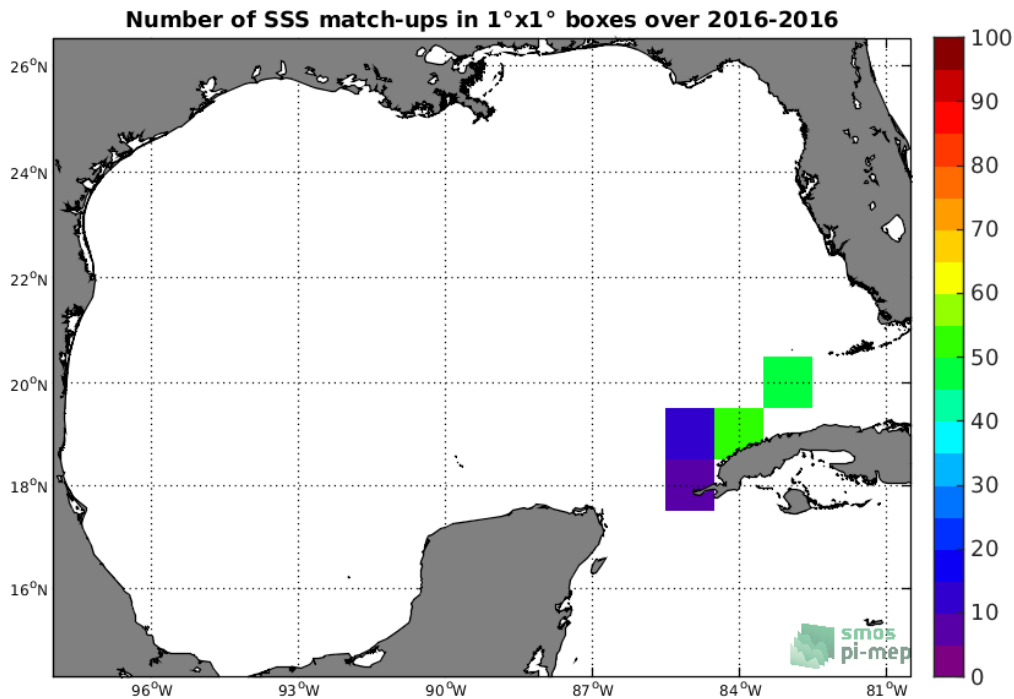
Figure 4: Number of SSS match-ups between TSG-LEGOS-DM SSS and the SMOS-L3-CATDS-CECOS-LOCEAN-V4-9DAYS-25KM SSS product for the Gulf of Mexico Pi-MEP region over 1°x1° boxes and for the full satellite product period.
