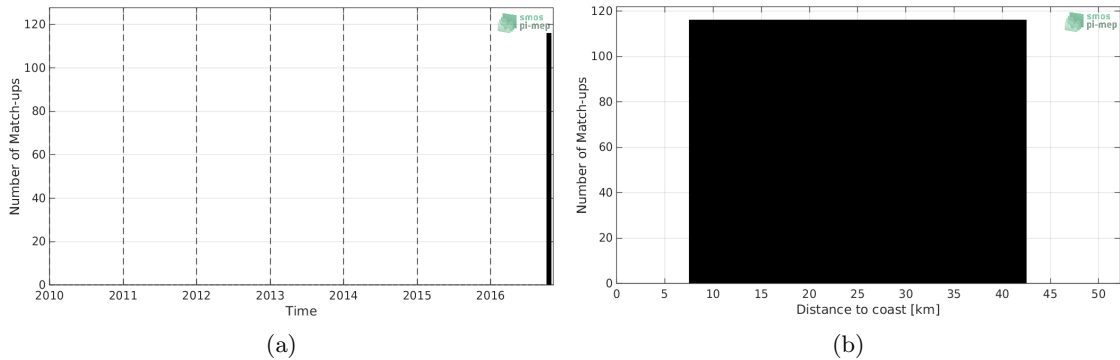
Figure 1: Number of match-ups between TSG-LEGOS-DM and SMOS-L3-CATDS-CECOS-LOCEAN-V4-9DAYS-25KM SSS as a function of time (a) and as function of the distance to coast (b) over the Gulf of Mexico Pi-MEP region and for the full satellite product period.
