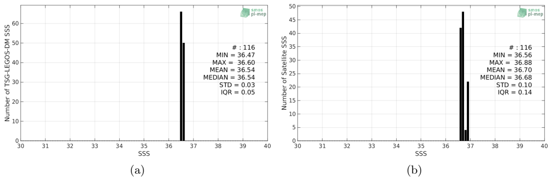
Figure 2: Histograms of SSS from TSG-LEGOS-DM (a) and SMOS-L3-CATDS-CECOS-LOCEAN-V4-9DAYS-25KM (b) considering all match-up pairs per bins of 0.1 over the Gulf of Mexico Pi-MEP region and for the full satellite product period.
