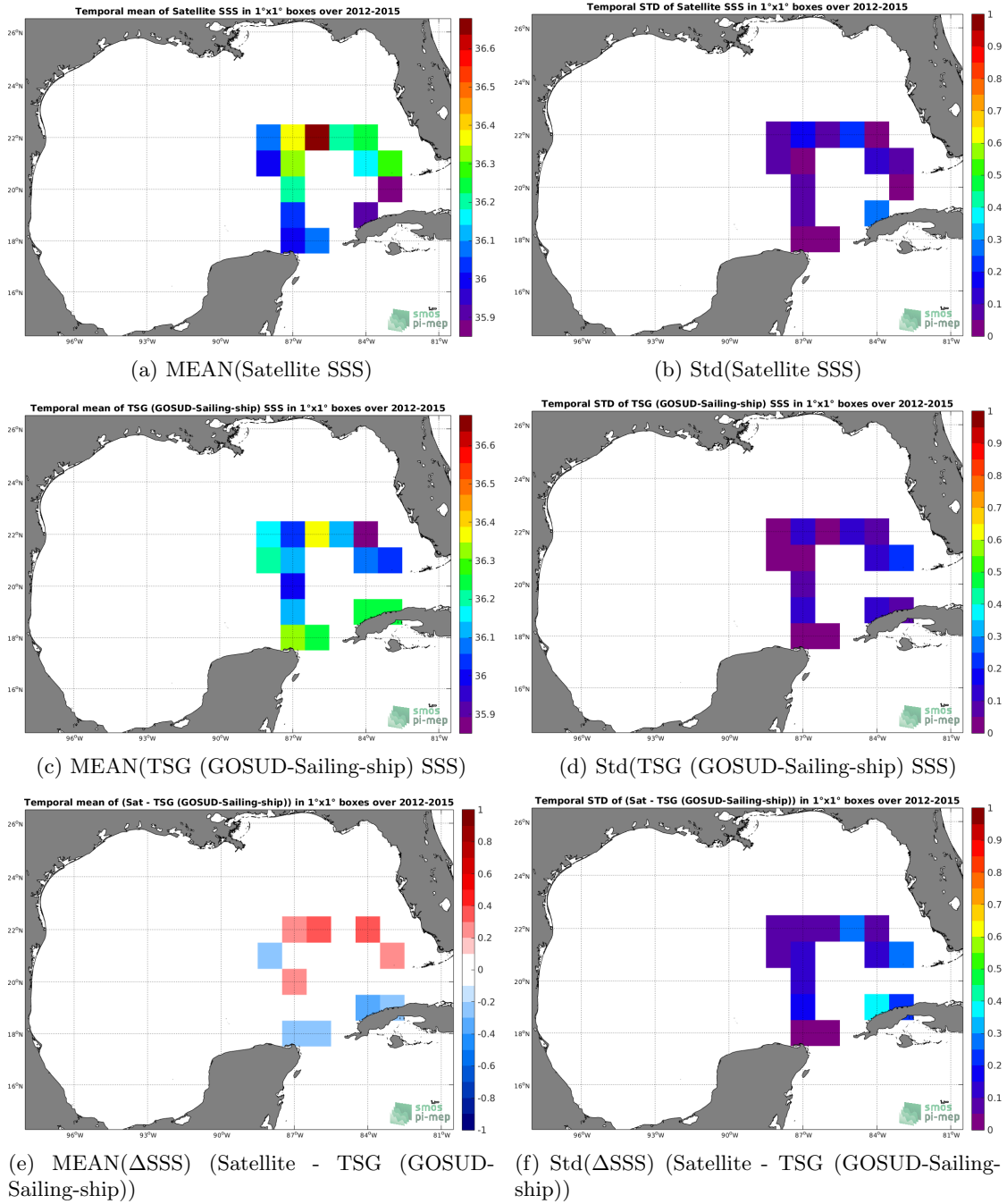
Figure 6: Temporal mean (left) and Std (right) of SSS from SMOS SSS L3 v4 - 9 Days (CATDS-CECOS-LOCEAN) (top), TSG (GOSUD-Sailing-ship) (middle), and of \Delta SSS (Satellite - TSG (GOSUD-Sailing-ship)). Only match-up pairs are used to generate these maps.
