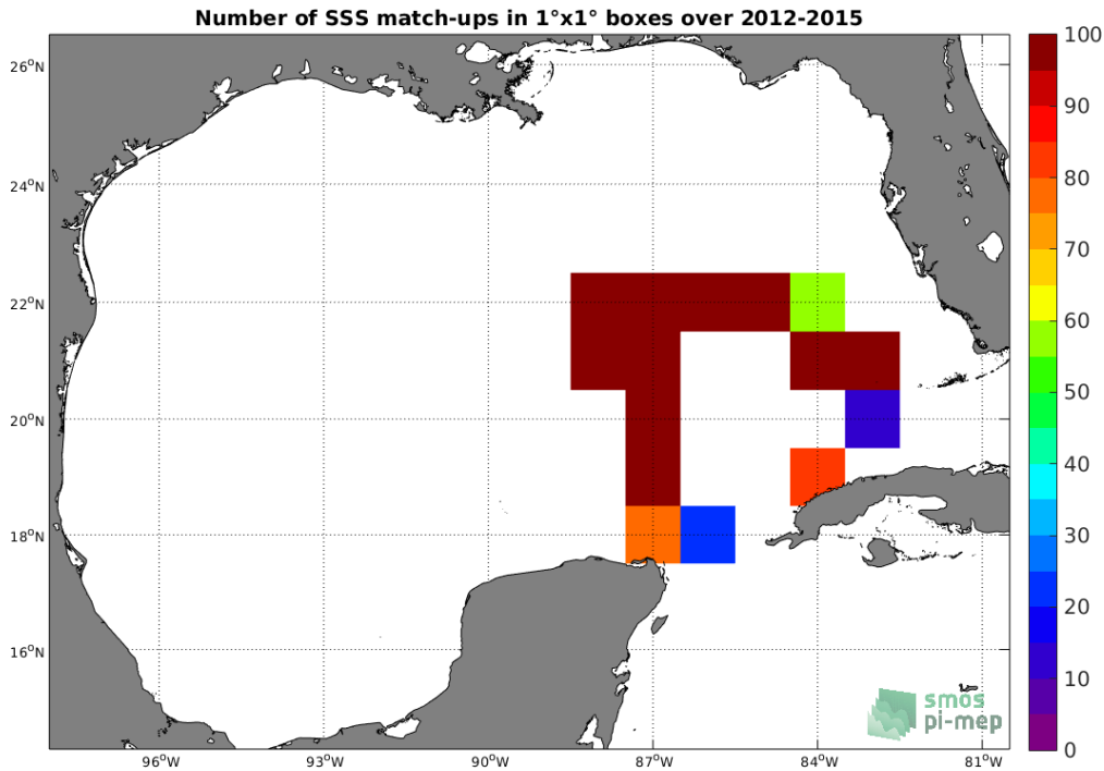
Figure 4: Number of SSS match-ups between TSG (GOSUD-Sailing-ship) SSS and the SMOS SSS L3 v4 - 9 Days (CATDS-CECOS-LOCEAN) SSS product for the Gulf of Mexico Pi-MEP region over 1°x1° boxes and for the full satellite product period.
