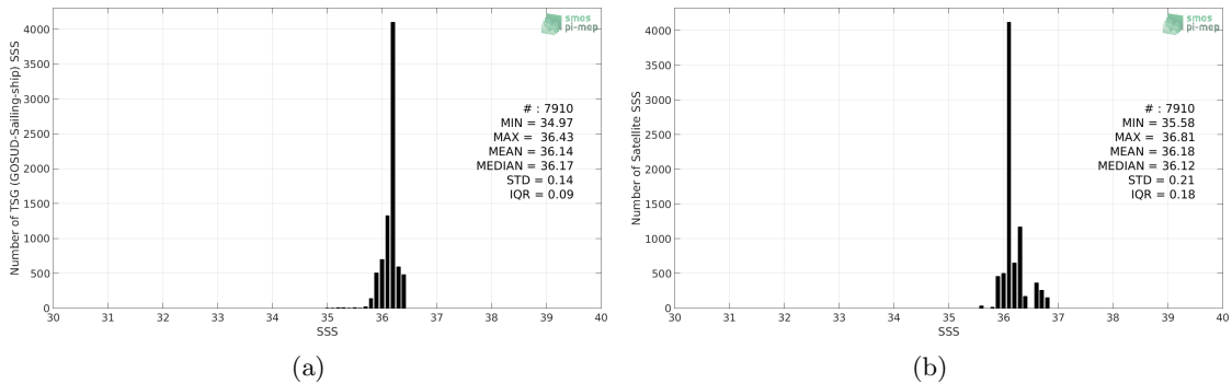
Figure 2: Histograms of SSS from TSG (GOSUD-Sailing-ship) (a) and SMOS SSS L3 v4 - 9 Days (CATDS-CECOS-LOCEAN) (b) considering all match-up pairs per bins of 0.1 over the Gulf of Mexico Pi-MEP region and for the full satellite product period.
