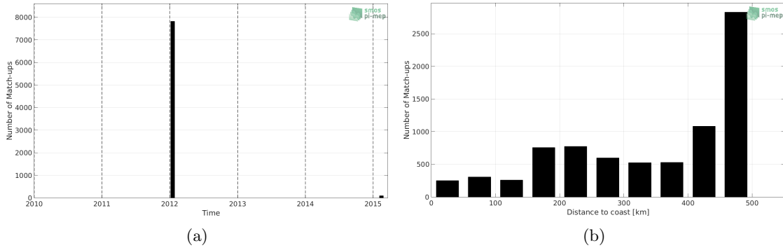
Figure 1: Number of match-ups between TSG (GOSUD-Sailing-ship) and SMOS SSS L3 v4 - 9 Days (CATDS-CECOS-LOCEAN) SSS as a function of time (a) and as function of the distance to coast (b) over the Gulf of Mexico Pi-MEP region and for the full satellite product period.
