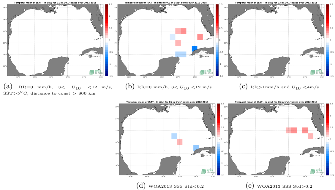
Figure 12: Temporal mean gridded over spatial boxes of size 1^\circ \times 1^\circ of \Delta SSS (SMOS SSS L3 v4 - 9 Days (CATDS-CECOS-LOCEAN) - TSG (GOSUD-Sailing-ship)) for 5 different subdatasets corresponding to:RR=0 mm/h, 3 < U_{10} < 12 m/s, SST >5^\circ\text{C} , distance to coast > 800 km (a), RR=0 mm/h, 3 < U_{10} < 12 m/s (b), RR >1 mm/h and U_{10} < 4 m/s (c), WOA2013 SSS Std <0.2 (d), WOA2013 SSS Std >0.2 (e).
