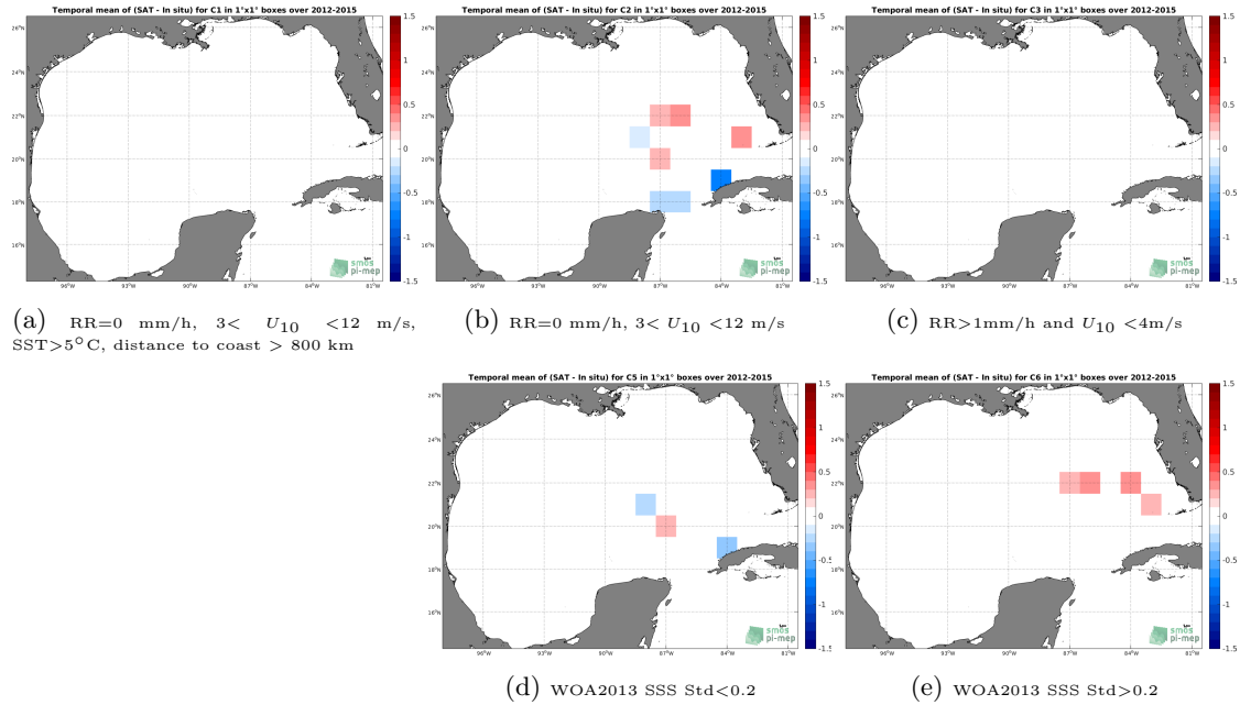
Figure 12: Temporal mean gridded over spatial boxes of size 1^{\circ}\times 1^{\circ} of \Delta SSS (SMOS-L3-CATDS-CECOS-LOCEAN-V4-9DAYS-25KM - TSG-GOSUD-Sailing-ship) for 5 different subdatasets corresponding to:RR=0 mm/h, 3 < U_{10} < 12 m/s, SST >5^{\circ}\text{C} , distance to coast > 800 km (a), RR=0 mm/h, 3 < U_{10} < 12 m/s (b), RR >1 mm/h and U_{10} < 4 m/s (c), WOA2013 SSS Std <0.2 (d), WOA2013 SSS Std >0.2 (e).
