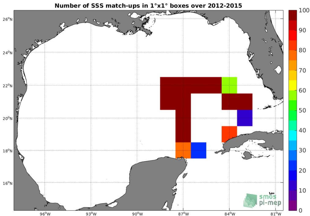
Figure 4: Number of SSS match-ups between TSG-GOSUD-Sailing-ship SSS and the SMOS-L3-CATDS-CECOS-LOCEAN-V4-9DAYS-25KM SSS product for the Gulf of Mexico Pi-MEP region over 1°x1° boxes and for the full satellite product period.
