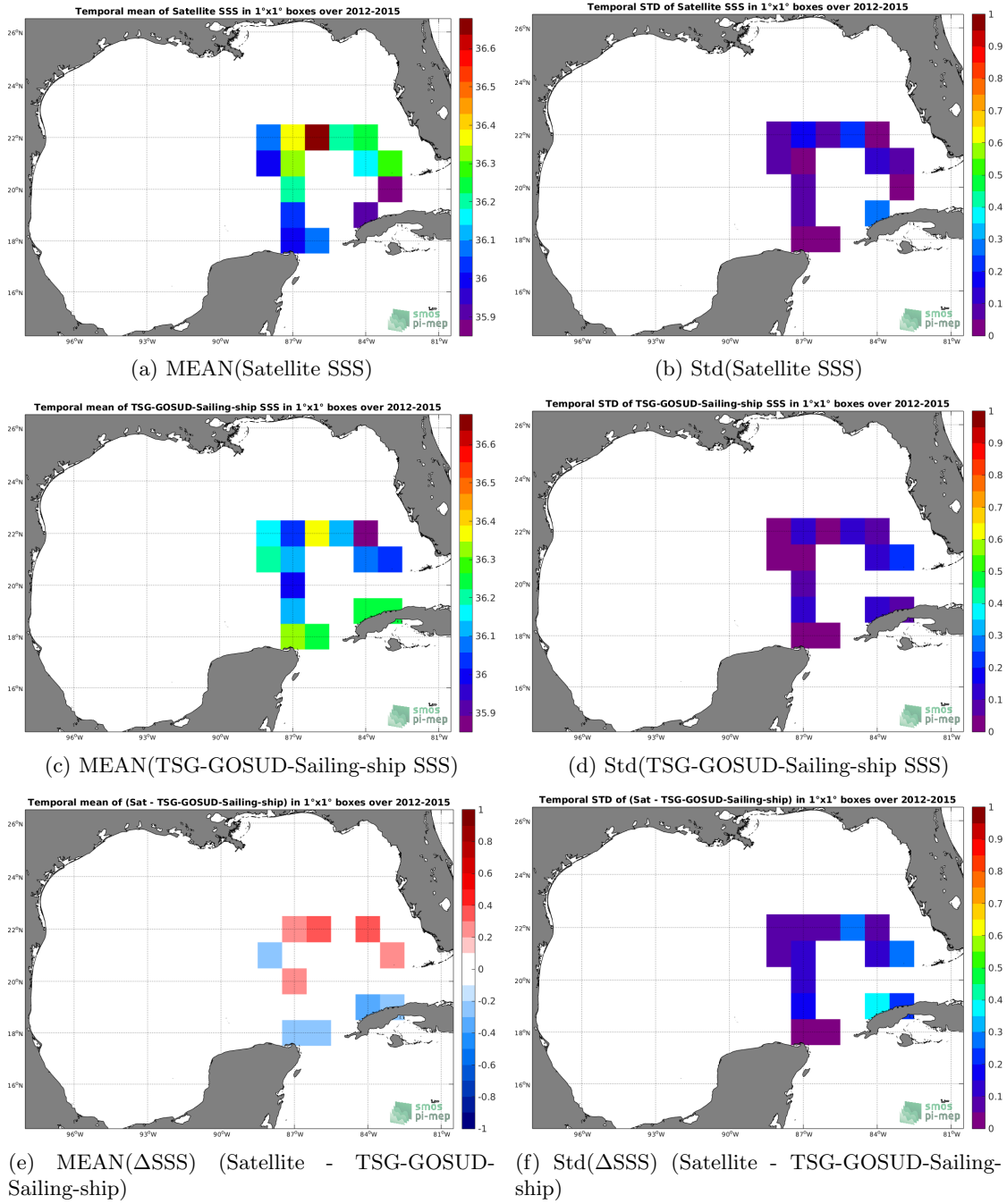
Figure 6: Temporal mean (left) and Std (right) of SSS from SMOS-L3-CATDS-CECOS-LOCEAN-V4-9DAYS-25KM (top), TSG-GOSUD-Sailing-ship (middle), and of \Delta SSS (Satellite - TSG-GOSUD-Sailing-ship). Only match-up pairs are used to generate these maps.
