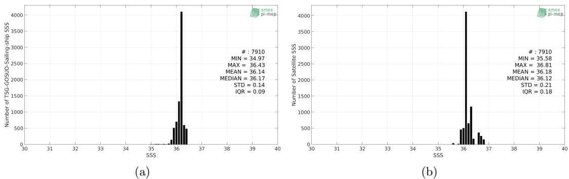
Figure 2: Histograms of SSS from TSG-GOSUD-Sailing-ship (a) and SMOS-L3-CATDS-CECOS-LOCEAN-V4-9DAYS-25KM (b) considering all match-up pairs per bins of 0.1 over the Gulf of Mexico Pi-MEP region and for the full satellite product period.
