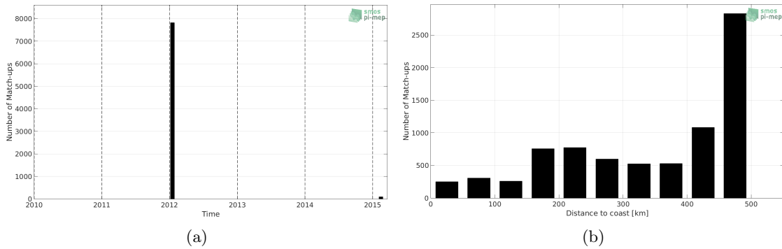
Figure 1: Number of match-ups between TSG-GOSUD-Sailing-ship and SMOS-L3-CATDS-CECOS-LOCEAN-V4-9DAYS-25KM SSS as a function of time (a) and as function of the distance to coast (b) over the Gulf of Mexico Pi-MEP region and for the full satellite product period.
