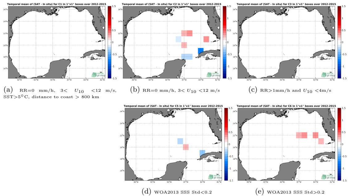
Figure 12: Temporal mean gridded over spatial boxes of size 1^\circ \times 1^\circ of \Delta SSS (SMOS-L3-CATDS-CECOS-LOCEAN-V4-9DAYS-25KM - TSG-GOSUD-Sailing-ship) for 5 different subdatasets corresponding to:RR=0 mm/h, 3 < U_{10} < 12 m/s, SST >5^\circ\text{C} , distance to coast > 800 km (a), RR=0 mm/h, 3 < U_{10} < 12 m/s (b), RR >1 mm/h and U_{10} < 4 m/s (c), WOA2013 SSS Std <0.2 (d), WOA2013 SSS Std >0.2 (e).
