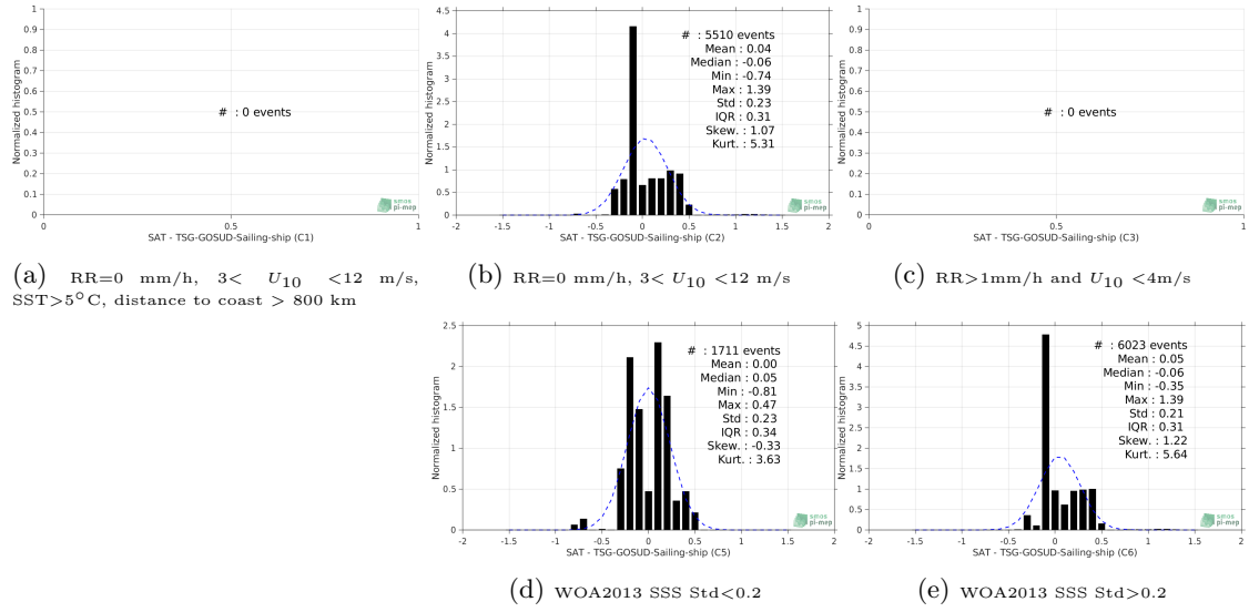
Figure 13: Normalized histogram of \Delta SSS (SMOS-L3-CATDS-CECOS-LOCEAN-V4-9DAYS-25KM - TSG-GOSUD-Sailing-ship) for 5 different subdatasets corresponding to: RR=0 mm/h, 3 < U_{10} < 12 m/s, SST > 5°C, distance to coast > 800 km (a), RR=0 mm/h, 3 < U_{10} < 12 m/s (b), RR > 1mm/h and U_{10} < 4 m/s (c), WOA2013 SSS Std < 0.2 (d), WOA2013 SSS Std > 0.2 (e).
