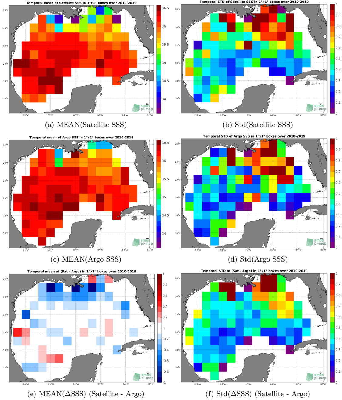
Figure 6: Temporal mean (left) and Std (right) of SSS from SMOS SSS L3 v4 - 9 Days (CATDS-CECOS-LOCEAN) (top), Argo (middle), and of \Delta SSS (Satellite - Argo). Only match-up pairs are used to generate these maps.
