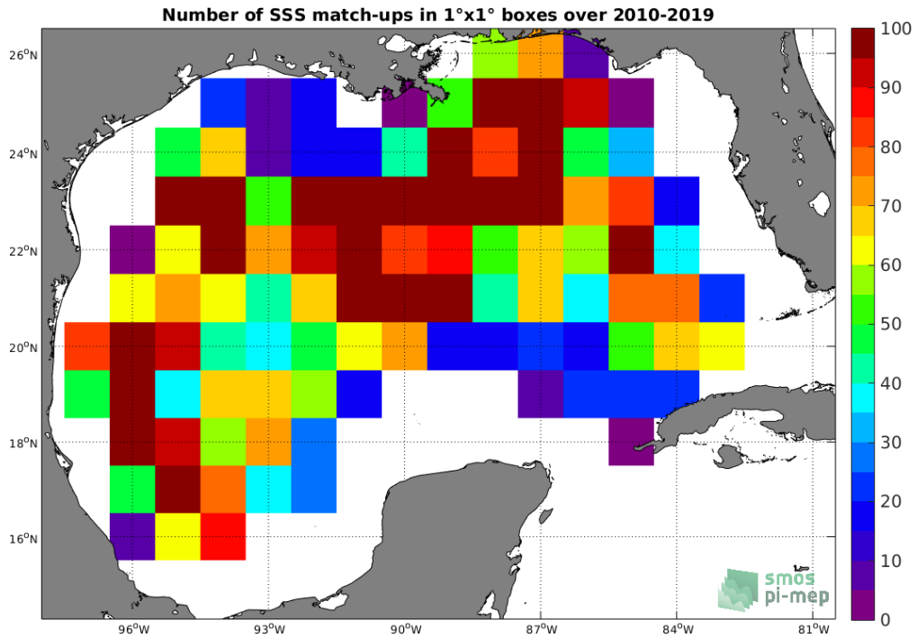
Figure 4: Number of SSS match-ups between Argo SSS and the SMOS SSS L3 v4 - 9 Days (CATDS-CECOS-LOCEAN) SSS product for the Gulf of Mexico Pi-MEP region over 1°x1° boxes and for the full satellite product period.
