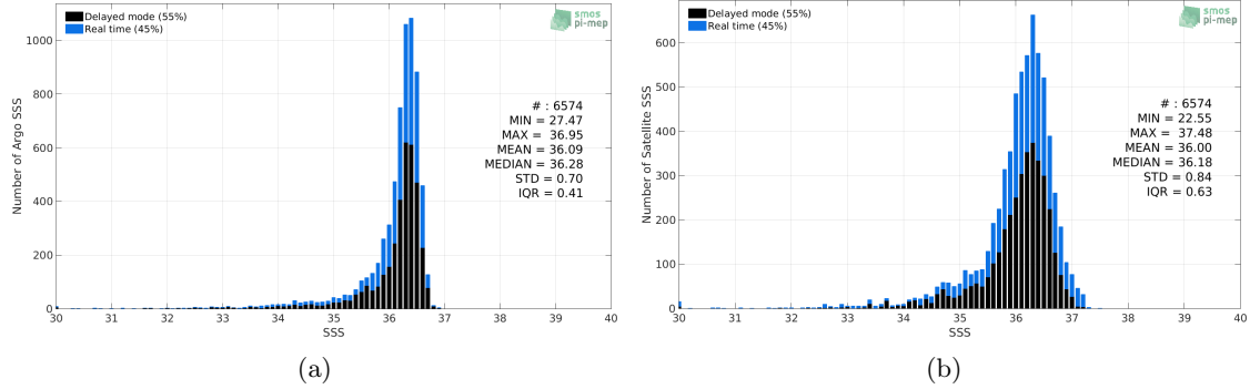
Figure 2: Histograms of SSS from Argo (a) and SMOS SSS L3 v4 - 9 Days (CATDS-CECOS-LOCEAN) (b) considering all match-up pairs per bins of 0.1 over the Gulf of Mexico Pi-MEP region and for the full satellite product period.
