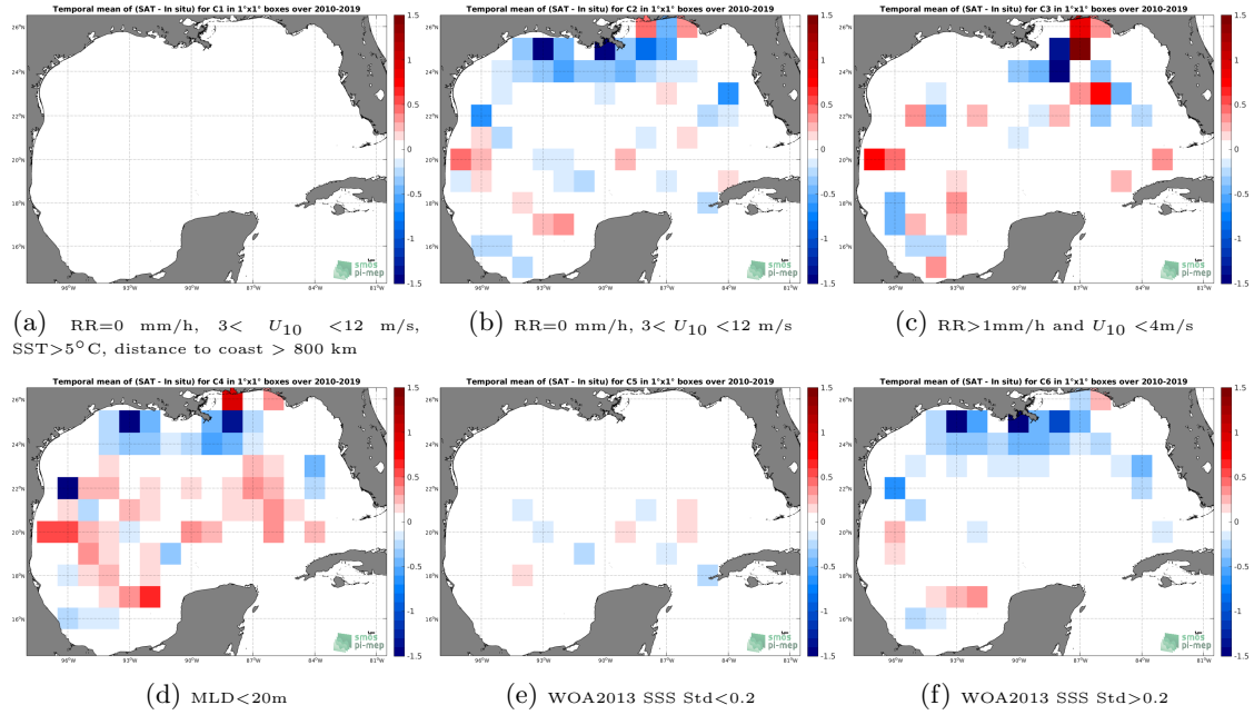
Figure 12: Temporal mean gridded over spatial boxes of size 1^\circ \times 1^\circ of \Delta SSS (SMOS SSS L3 v4 - 9 Days (CATDS-CECOS-LOCEAN) - Argo) for 6 different subdatasets corresponding to: RR=0 mm/h, 3 < U_{10} < 12 m/s, SST >5^\circ\text{C} , distance to coast > 800 km (a), RR=0 mm/h, 3 < U_{10} < 12 m/s (b), RR >1 mm/h and U_{10} < 4 m/s (c),MLD <20 m (d),WOA2013 SSS Std <0.2 (e),WOA2013 SSS Std >0.2 (f).
