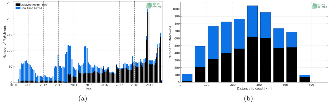
Figure 1: Number of match-ups between Argo and SMOS SSS L3 v4 - 9 Days (CATDS-CECOS-LOCEAN) SSS as a function of time (a) and as function of the distance to coast (b) over the Gulf of Mexico Pi-MEP region and for the full satellite product period.
