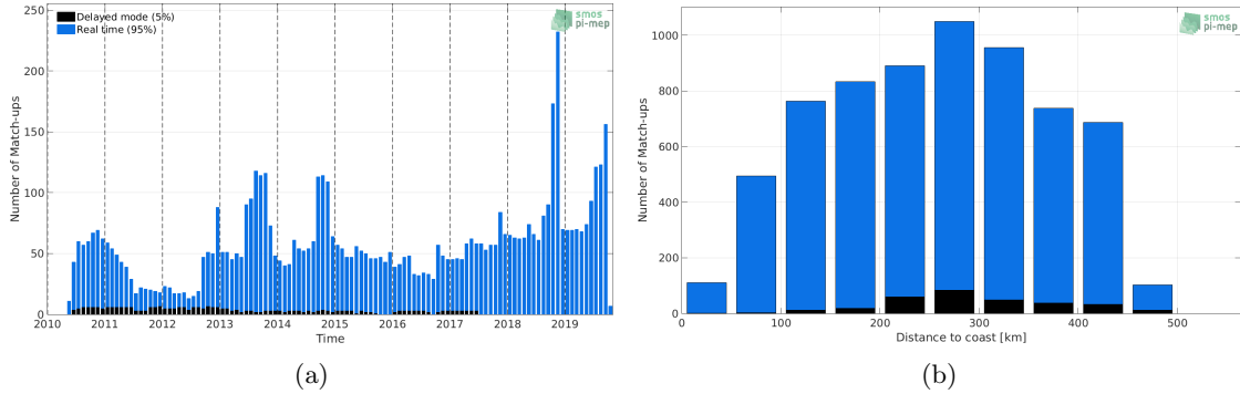
Figure 1: Number of match-ups between Argo and SMOS-L3-CATDS-CECOS-LOCEAN-V4-9DAYS-25KM SSS as a function of time (a) and as function of the distance to coast (b) over the Gulf of Mexico Pi-MEP region and for the full satellite product period.
