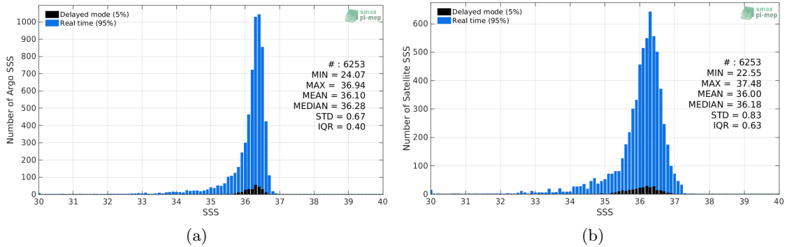
Figure 2: Histograms of SSS from Argo (a) and SMOS-L3-CATDS-CECOS-LOCEAN-V4-9DAYS-25KM (b) considering all match-up pairs per bins of 0.1 over the Gulf of Mexico Pi-MEP region and for the full satellite product period.
