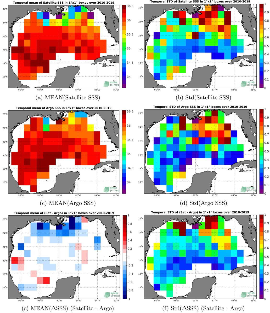
Figure 6: Temporal mean (left) and Std (right) of SSS from SMOS-L3-CATDS-CECOS-LOCEAN-V4-9DAYS-25KM (top), Argo (middle), and of \Delta SSS (Satellite - Argo). Only match-up pairs are used to generate these maps.
