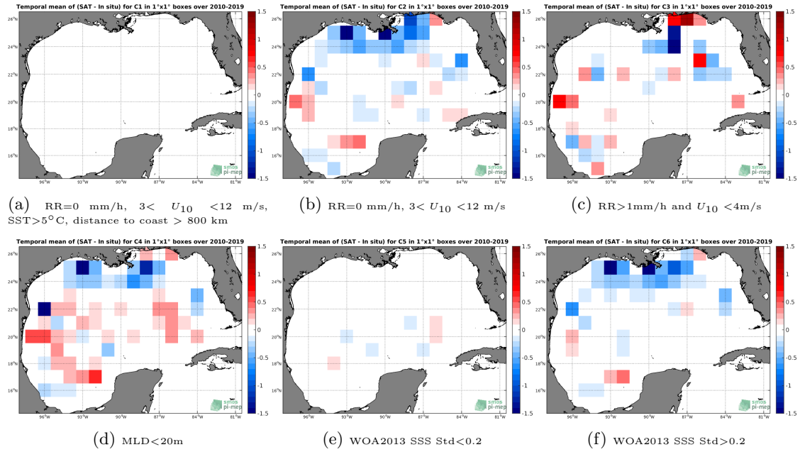
Figure 12: Temporal mean gridded over spatial boxes of size 1^\circ \times 1^\circ of \Delta SSS (SMOS-L3-CATDS-CECOS-LOCEAN-V4-9DAYS-25KM - Argo) for 6 different subdatasets corresponding to:RR=0 mm/h, 3 < U_{10} < 12 m/s, SST >5^\circ C, distance to coast > 800 km (a), RR=0 mm/h, 3 < U_{10} < 12 m/s (b), RR >1 mm/h and U_{10} < 4 m/s (c),MLD <20 m (d),WOA2013 SSS Std <0.2 (e),WOA2013 SSS Std >0.2 (f).
