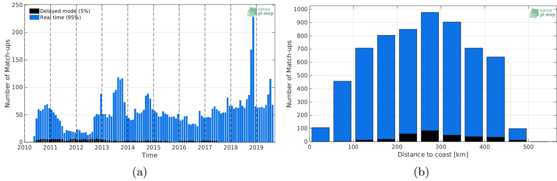
Figure 1: Number of match-ups between Argo and SMOS-L3-CATDS-CECOS-LOCEAN-V4-9DAYS-25KM SSS as a function of time (a) and as function of the distance to coast (b) over the Gulf of Mexico Pi-MEP region and for the full satellite product period.
