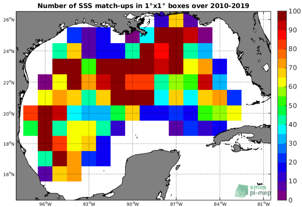
Figure 4: Number of SSS match-ups between Argo SSS and the SMOS-L3-CATDS-CECOS-LOCEAN-V4-9DAYS-25KM SSS product for the Gulf of Mexico Pi-MEP region over 1°x1° boxes and for the full satellite product period.
