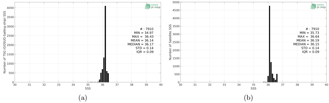
Figure 2: Histograms of SSS from TSG (GOSUD-Sailing-ship) (a) and SMOS SSS L3 v4 - 18 Days (CATDS-CECOS-LOCEAN) (b) considering all match-up pairs per bins of 0.1 over the Gulf of Mexico Pi-MEP region and for the full satellite product period.
