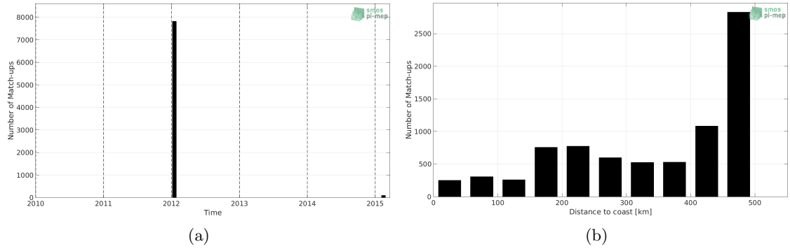
Figure 1: Number of match-ups between TSG (GOSUD-Sailing-ship) and SMOS SSS L3 v4 - 18 Days (CATDS-CECOS-LOCEAN) SSS as a function of time (a) and as function of the distance to coast (b) over the Gulf of Mexico Pi-MEP region and for the full satellite product period.
