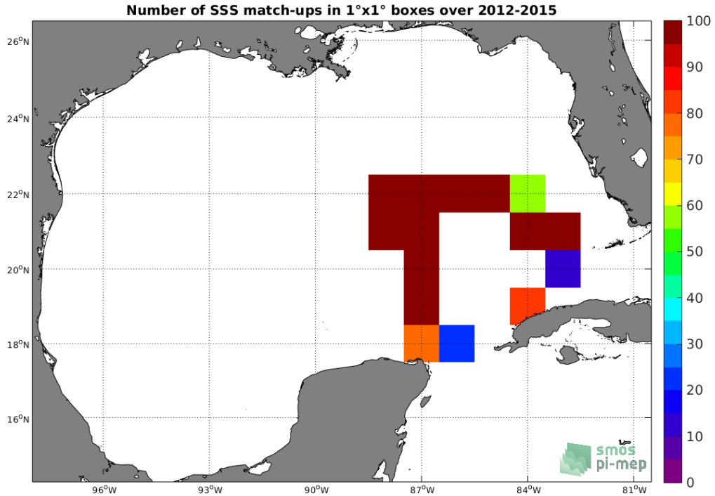
Figure 4: Number of SSS match-ups between TSG (GOSUD-Sailing-ship) SSS and the SMOS SSS L3 v4 - 18 Days (CATDS-CECOS-LOCEAN) SSS product for the Gulf of Mexico Pi-MEP region over 1°x1° boxes and for the full satellite product period.
