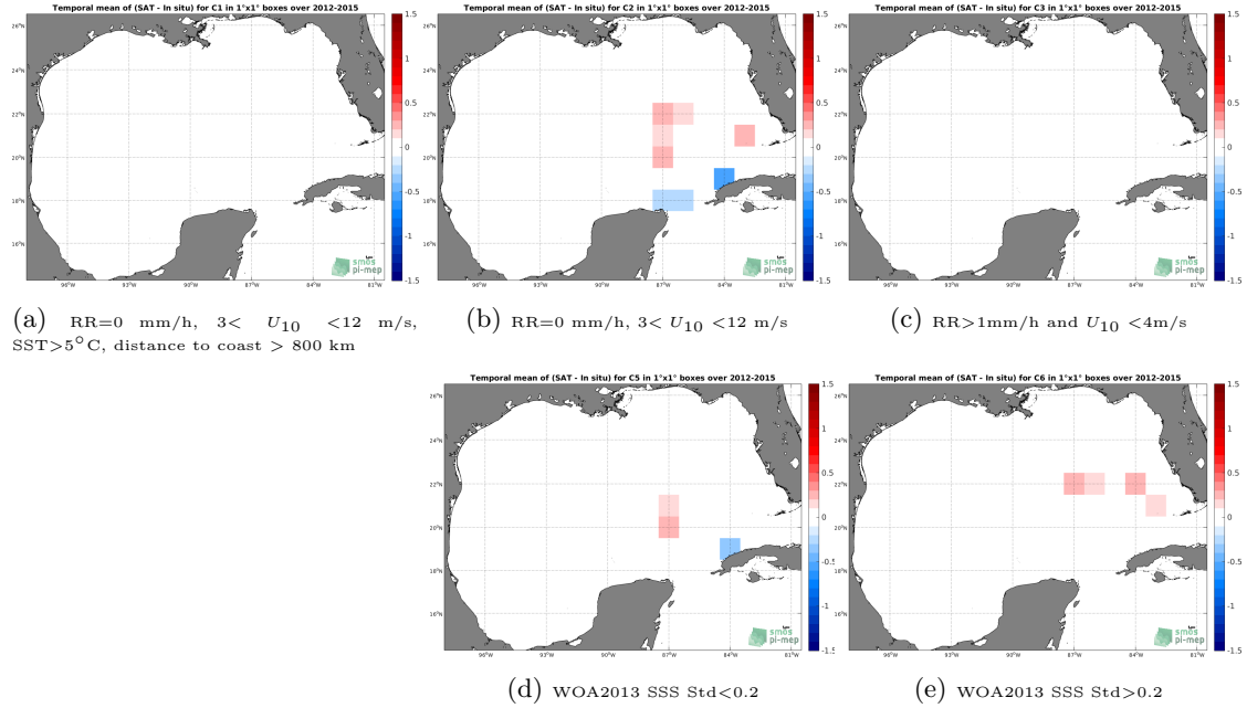
Figure 12: Temporal mean gridded over spatial boxes of size 1^\circ \times 1^\circ of \Delta SSS (SMOS SSS L3 v4 - 18 Days (CATDS-CECOS-LOCEAN) - TSG (GOSUD-Sailing-ship)) for 5 different subdatasets corresponding to: RR=0 mm/h, 3 < U_{10} < 12 m/s, SST >5^\circ\text{C} , distance to coast > 800 km (a), RR=0 mm/h, 3 < U_{10} < 12 m/s (b), RR >1 mm/h and U_{10} < 4 m/s (c), WOA2013 SSS Std <0.2 (d), WOA2013 SSS Std >0.2 (e).
