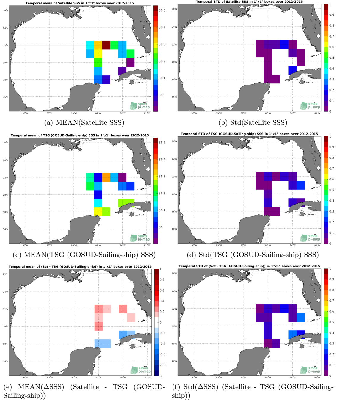
Figure 6: Temporal mean (left) and Std (right) of SSS from SMOS SSS L3 v4 - 18 Days (CATDS-CECOS-LOCEAN) (top), TSG (GOSUD-Sailing-ship) (middle), and of \Delta SSS (Satellite - TSG (GOSUD-Sailing-ship)). Only match-up pairs are used to generate these maps.
