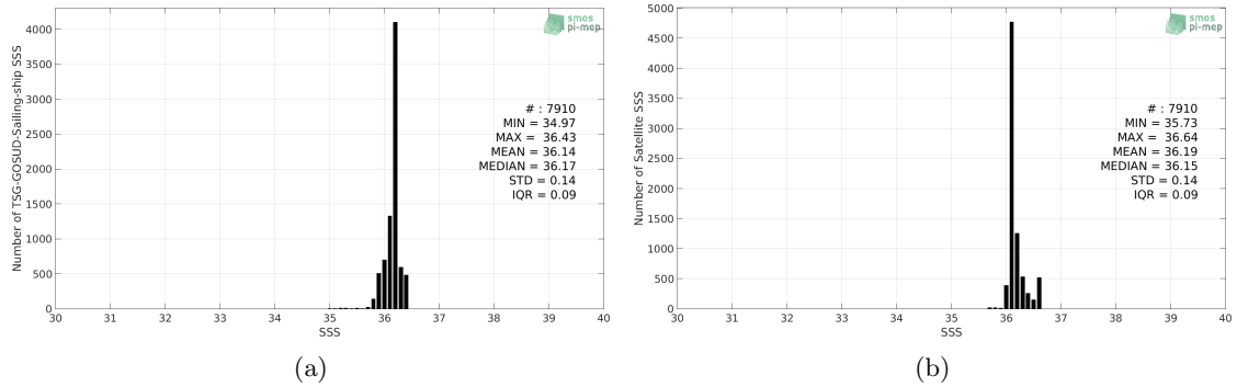
Figure 2: Histograms of SSS from TSG-GOSUD-Sailing-ship (a) and SMOS-L3-CATDS-CECOS-LOCEAN-V4-18DAYS-25KM (b) considering all match-up pairs per bins of 0.1 over the Gulf of Mexico Pi-MEP region and for the full satellite product period.
