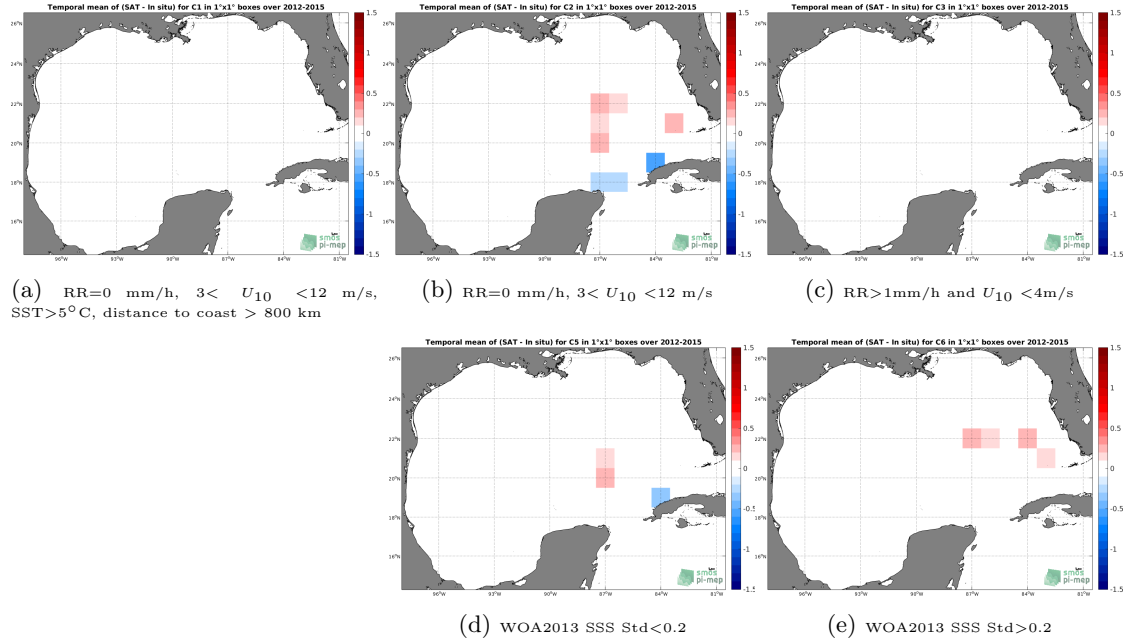
Figure 12: Temporal mean gridded over spatial boxes of size 1^\circ \times 1^\circ of \Delta SSS (SMOS-L3-CATDS-CECOS-LOCEAN-V4-18DAYS-25KM - TSG-GOSUD-Sailing-ship) for 5 different subdatasets corresponding to: RR=0 mm/h, 3 < U_{10} < 12 m/s, SST >5^\circ\text{C} , distance to coast > 800 km (a), RR=0 mm/h, 3 < U_{10} < 12 m/s (b), RR >1 mm/h and U_{10} < 4 m/s (c), WOA2013 SSS Std <0.2 (d), WOA2013 SSS Std >0.2 (e).
