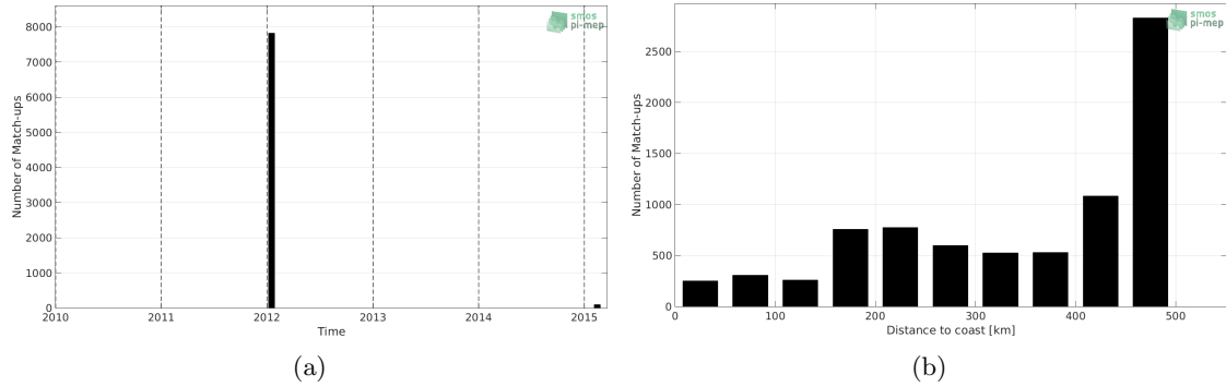
Figure 1: Number of match-ups between TSG-GOSUD-Sailing-ship and SMOS-L3-CATDS-CECOS-LOCEAN-V4-18DAYS-25KM SSS as a function of time (a) and as function of the distance to coast (b) over the Gulf of Mexico Pi-MEP region and for the full satellite product period.
