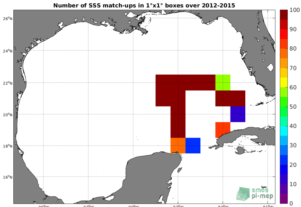
Figure 4: Number of SSS match-ups between TSG-GOSUD-Sailing-ship SSS and the SMOS-L3-CATDS-CECOS-LOCEAN-V4-18DAYS-25KM SSS product for the Gulf of Mexico Pi-MEP region over 1°x1° boxes and for the full satellite product period.
