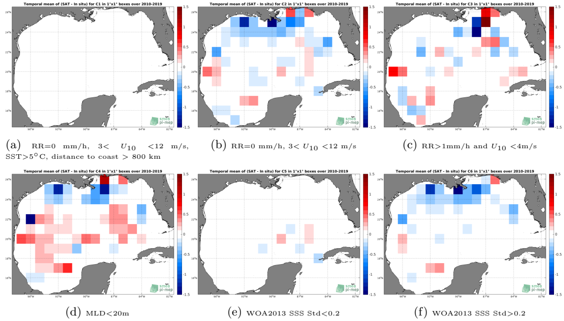
Figure 12: Temporal mean gridded over spatial boxes of size 1^\circ \times 1^\circ of \Delta SSS (SMOS SSS L3 v4 - 18 Days (CATDS-CECOS-LOCEAN) - Argo) for 6 different subdatasets corresponding to: RR=0 mm/h, 3 < U_{10} < 12 m/s, SST > 5^\circ C , distance to coast > 800 km (a), RR=0 mm/h, 3 < U_{10} < 12 m/s (b), RR > 1 mm/h and U_{10} < 4 m/s (c), MLD < 20 m (d), WOA2013 SSS Std < 0.2 (e), WOA2013 SSS Std > 0.2 (f).
