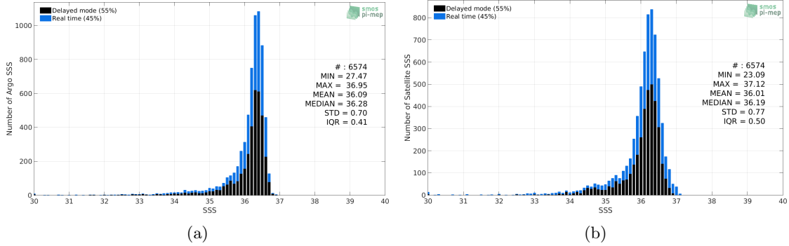
Figure 2: Histograms of SSS from Argo (a) and SMOS SSS L3 v4 - 18 Days (CATDS-CECOS-LOCEAN) (b) considering all match-up pairs per bins of 0.1 over the Gulf of Mexico Pi-MEP region and for the full satellite product period.
