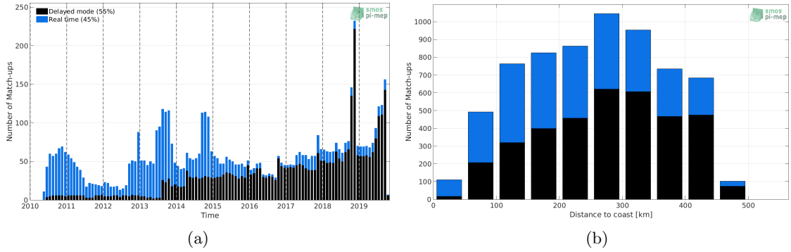
Figure 1: Number of match-ups between Argo and SMOS SSS L3 v4 - 18 Days (CATDS-CECOS-LOCEAN) SSS as a function of time (a) and as function of the distance to coast (b) over the Gulf of Mexico Pi-MEP region and for the full satellite product period.
