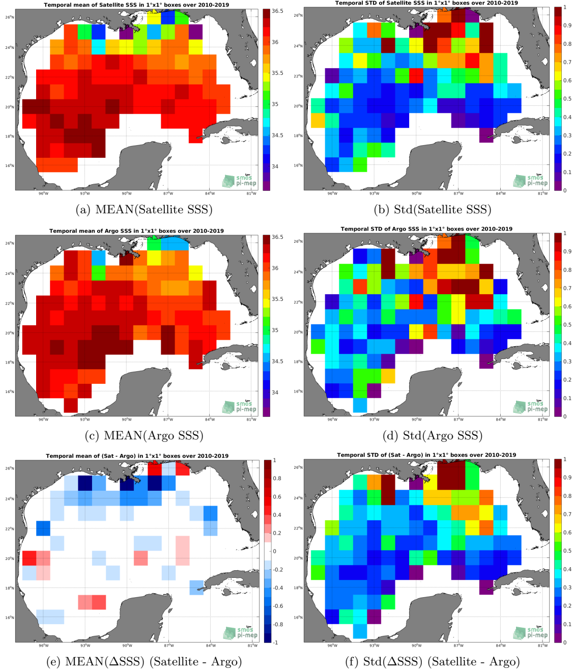
Figure 6: Temporal mean (left) and Std (right) of SSS from SMOS SSS L3 v4 - 18 Days (CATDS-CECOS-LOCEAN) (top), Argo (middle), and of \Delta SSS (Satellite - Argo). Only match-up pairs are used to generate these maps.
