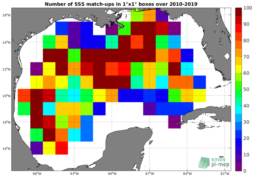
Figure 4: Number of SSS match-ups between Argo SSS and the SMOS SSS L3 v4 - 18 Days (CATDS-CECOS-LOCEAN) SSS product for the Gulf of Mexico Pi-MEP region over 1^\circ \times 1^\circ boxes and for the full satellite product period.
