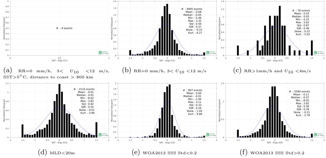
Figure 13: Normalized histogram of \Delta\text{SSS} (SMOS-L3-CATDS-CECOS-LOCEAN-V4-18DAYS-25KM - Argo) for 6 different subdatasets corresponding to: RR=0 mm/h, 3 < U_{10} < 12 m/s, SST > 5^\circ\text{C} , distance to coast > 800 km (a), RR=0 mm/h, 3 < U_{10} < 12 m/s (b), RR > 1\text{mm/h} and U_{10} < 4\text{m/s} (c), MLD < 20\text{m} (d), WOA2013 SSS Std < 0.2 (e), WOA2013 SSS Std > 0.2 (f).
