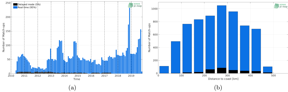
Figure 1: Number of match-ups between Argo and SMOS-L3-CATDS-CECOS-LOCEAN-V4-18DAYS-25KM SSS as a function of time (a) and as function of the distance to coast (b) over the Gulf of Mexico Pi-MEP region and for the full satellite product period.
