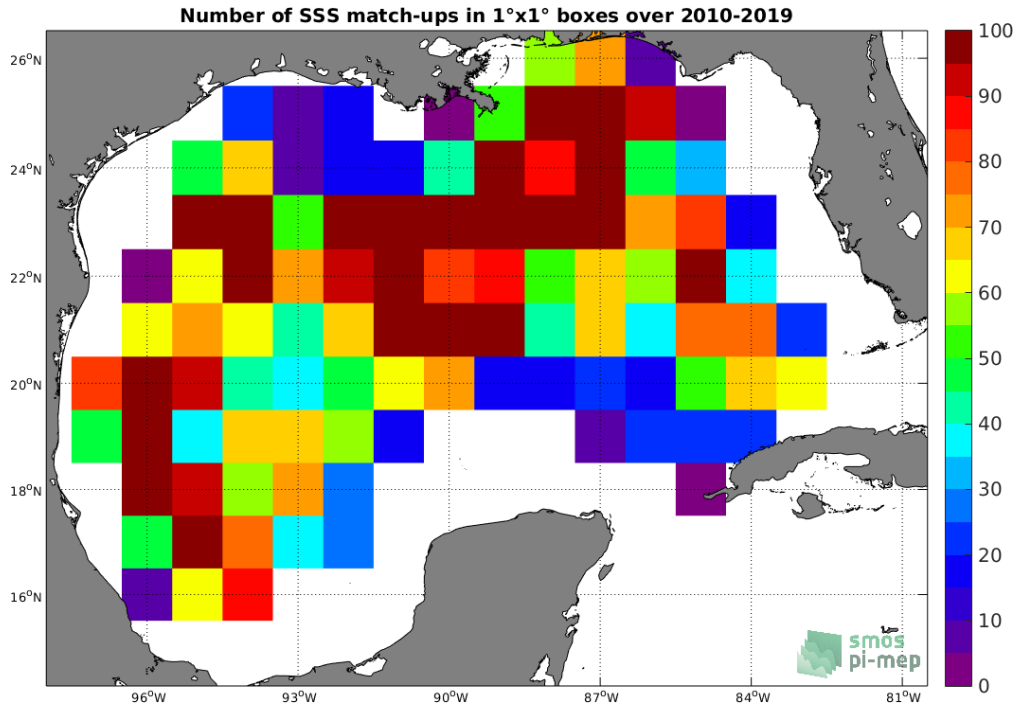
Figure 4: Number of SSS match-ups between Argo SSS and the SMOS-L3-CATDS-CECOS-LOCEAN-V4-18DAYS-25KM SSS product for the Gulf of Mexico Pi-MEP region over 1^\circ \times 1^\circ boxes and for the full satellite product period.
