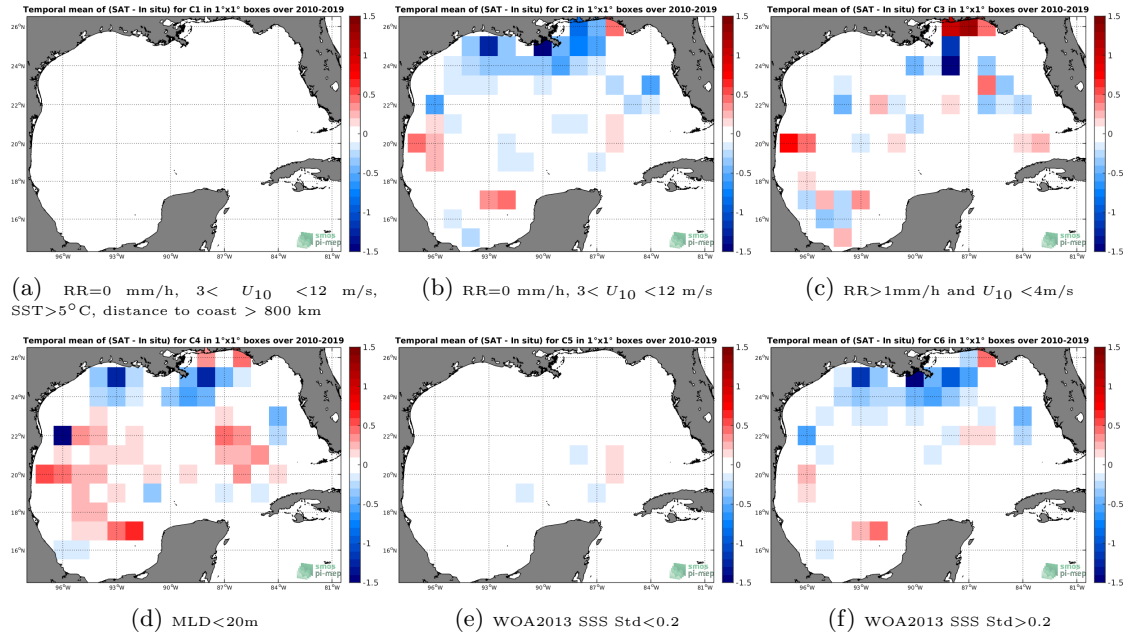
Figure 12: Temporal mean gridded over spatial boxes of size 1^\circ \times 1^\circ of \Delta SSS (SMOS-L3-CATDS-CECOS-LOCEAN-V4-18DAYS-25KM - Argo) for 6 different subdatasets corresponding to:RR=0 mm/h, 3 < U_{10} < 12 m/s, SST >5^\circ C, distance to coast > 800 km (a), RR=0 mm/h, 3 < U_{10} < 12 m/s (b), RR >1 mm/h and U_{10} < 4 m/s (c),MLD <20 m (d),WOA2013 SSS Std <0.2 (e),WOA2013 SSS Std >0.2 (f).
