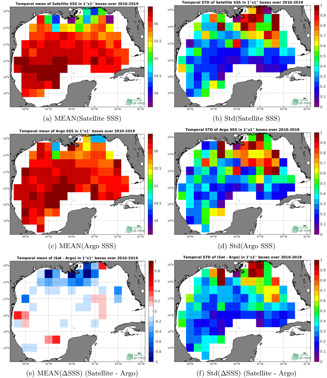
Figure 6: Temporal mean (left) and Std (right) of SSS from SMOS-L3-CATDS-CECOS-LOCEAN-V4-18DAYS-25KM (top), Argo (middle), and of \Delta SSS (Satellite - Argo). Only match-up pairs are used to generate these maps.
