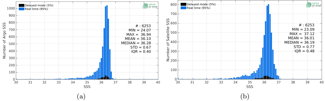
Figure 2: Histograms of SSS from Argo (a) and SMOS-L3-CATDS-CECOS-LOCEAN-V4-18DAYS-25KM (b) considering all match-up pairs per bins of 0.1 over the Gulf of Mexico Pi-MEP region and for the full satellite product period.
