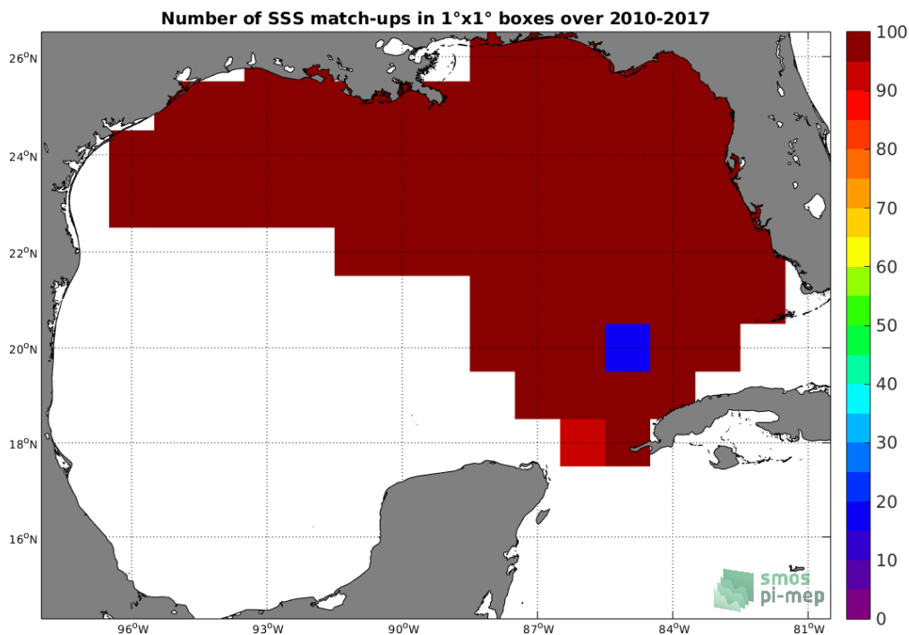
Figure 4: Number of SSS match-ups between TSG-SAMOS SSS and the SMOS-L3-CATDS-CECOS-LOCEAN-V3-9DAYS-25KM SSS product for the Gulf of Mexico Pi-MEP region over 1^\circ \times 1^\circ boxes and for the full satellite product period.
