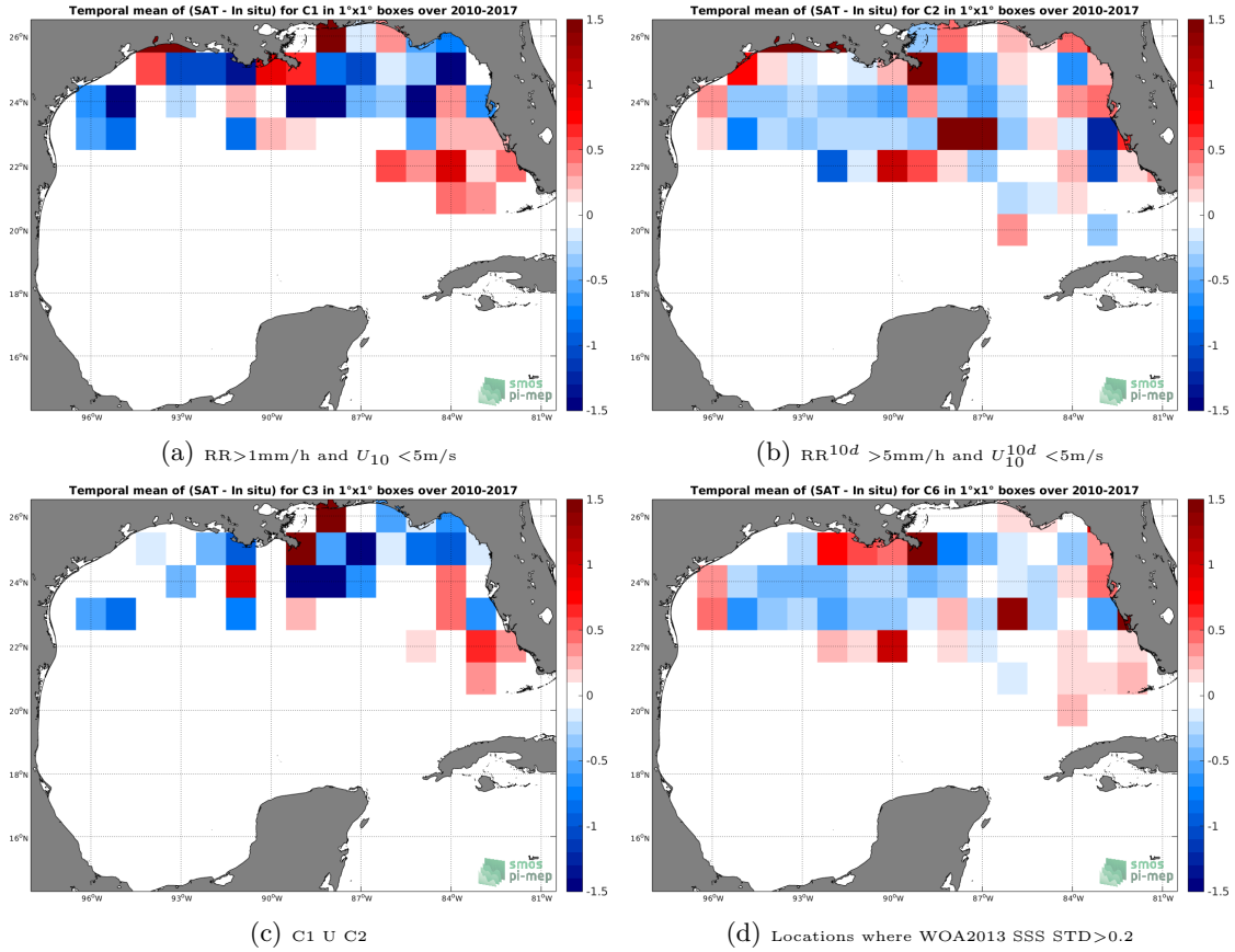
Figure 12: Temporal mean gridded over spatial boxes of size 1^\circ \times 1^\circ of \Delta SSS (SMOS-L3-CATDS-CECOS-LOCEAN-V3-9DAYS-25KM - TSG-SAMOS) for 4 different subdatasets corresponding to: RR > 1\text{mm/h} and U_{10} < 5\text{m/s} (a), RR^{10d} > 5\text{mm/h} and U_{10}^{10d} < 5\text{m/s} (b), C1 U C2 (c), Locations where WOA2013 SSS STD > 0.2 (d).
