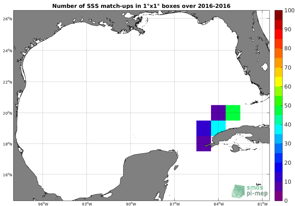
Figure 4: Number of SSS match-ups between TSG-LEGOS-DM SSS and the SMOS-L3-CATDS-CECOS-LOCEAN-V3-9DAYS-25KM SSS product for the Gulf of Mexico Pi-MEP region over 1^\circ \times 1^\circ boxes and for the full satellite product period.
