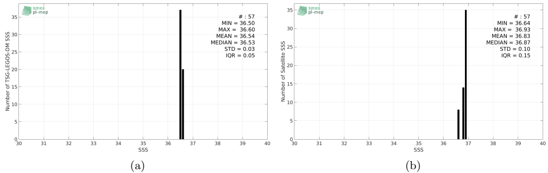
Figure 2: Histograms of SSS from TSG-LEGOS-DM (a) and SMOS-L3-CATDS-CECOS-LOCEAN-V3-9DAYS-25KM (b) considering all match-up pairs per bins of 0.1 over the Gulf of Mexico Pi-MEP region and for the full satellite product period.
