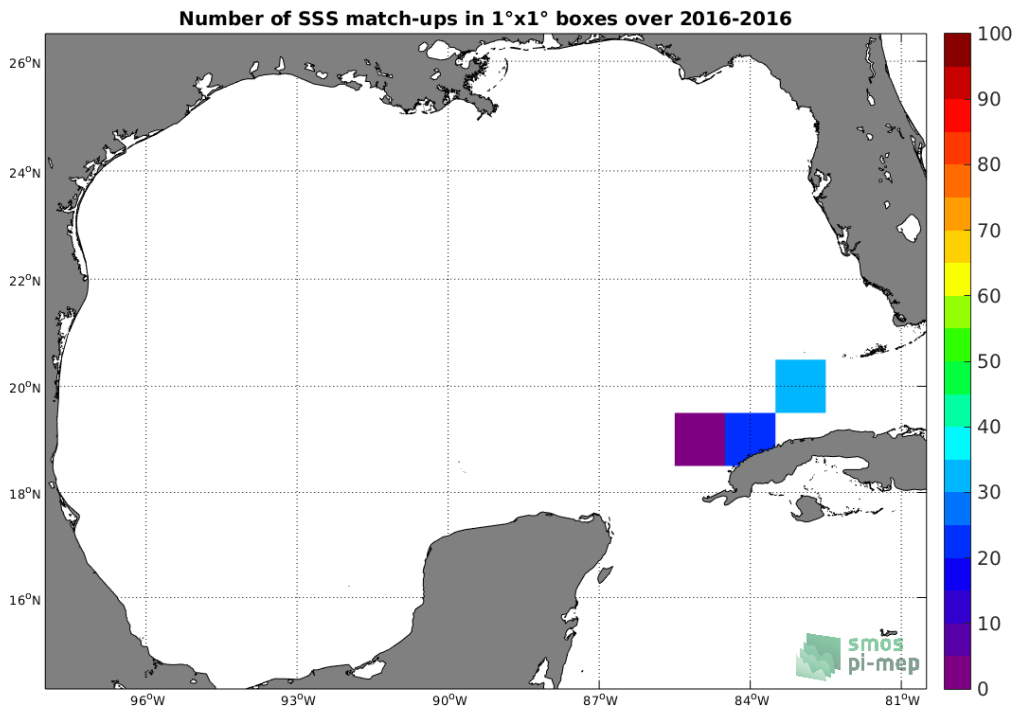
Figure 4: Number of SSS match-ups between TSG-LEGOS-DM SSS and the SMOS-L3-CATDS-CECOS-LOCEAN-V3-9DAYS-25KM SSS product for the Gulf of Mexico Pi-MEP region over 1°x1° boxes and for the full satellite product period.
