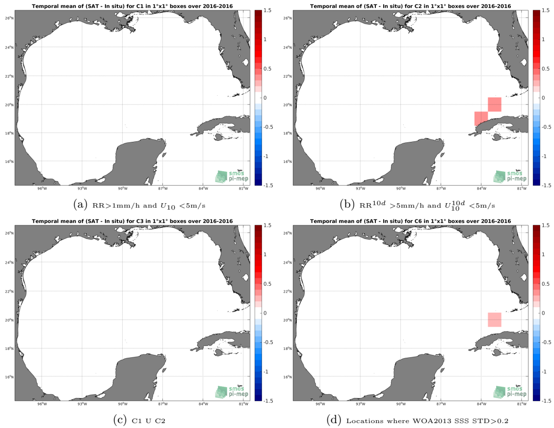
Figure 12: Temporal mean gridded over spatial boxes of size 1^\circ \times 1^\circ of \Delta SSS (SMOS-L3-CATDS-CECOS-LOCEAN-V3-9DAYS-25KM - TSG-LEGOS-DM) for 4 different subdatasets corresponding to: RR > 1mm/h and U_{10} < 5\text{m/s} (a), RR^{10d} > 5\text{mm/h} and U_{10}^{10d} < 5\text{m/s} (b), C1 U C2 (c), Locations where WOA2013 SSS STD > 0.2 (d).
