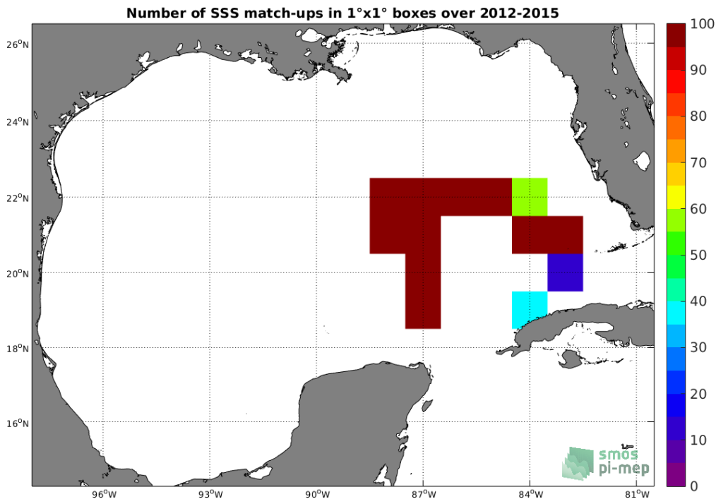
Figure 4: Number of SSS match-ups between TSG-GOSUD-Sailing-ship SSS and the SMOS-L3-CATDS-CECOS-LOCEAN-V3-9DAYS-25KM SSS product for the Gulf of Mexico Pi-MEP region over 1°x1° boxes and for the full satellite product period.
