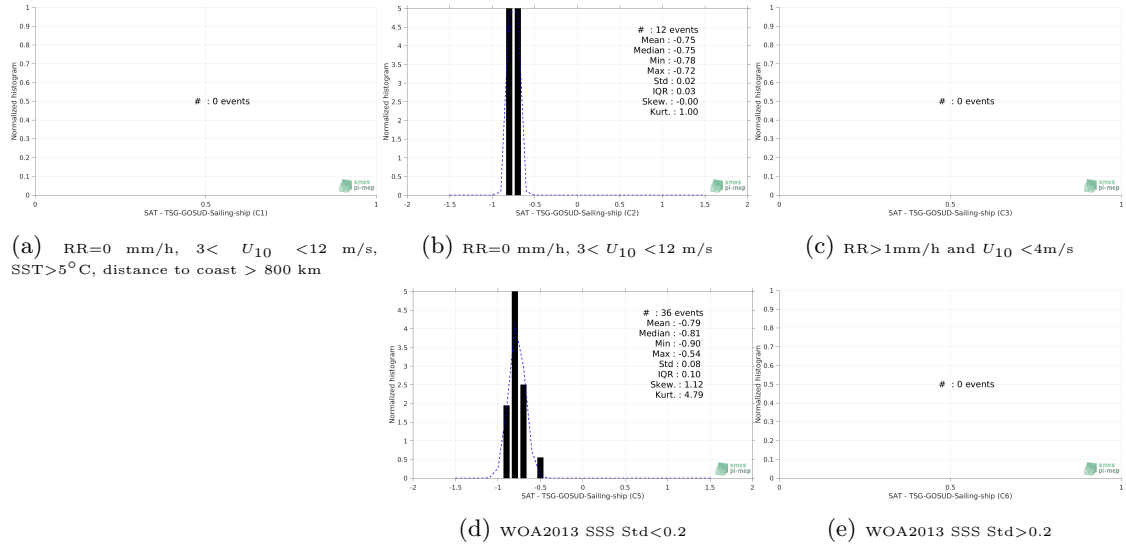
Figure 13: Normalized histogram of \Delta\text{SSS} (SMOS-L3-CATDS-CECOS-LOCEAN-V3-9DAYS-25KM - TSG-GOSUD-Sailing-ship) for 5 different subdatasets corresponding to: RR=0 mm/h, 3 < U_{10} < 12 m/s, SST > 5^\circ\text{C} , distance to coast > 800 km (a), RR=0 mm/h, 3 < U_{10} < 12 m/s (b), RR > 1\text{mm/h} and U_{10} < 4\text{m/s} (c), WOA2013 SSS \text{Std} < 0.2 (d), WOA2013 SSS \text{Std} > 0.2 (e).
