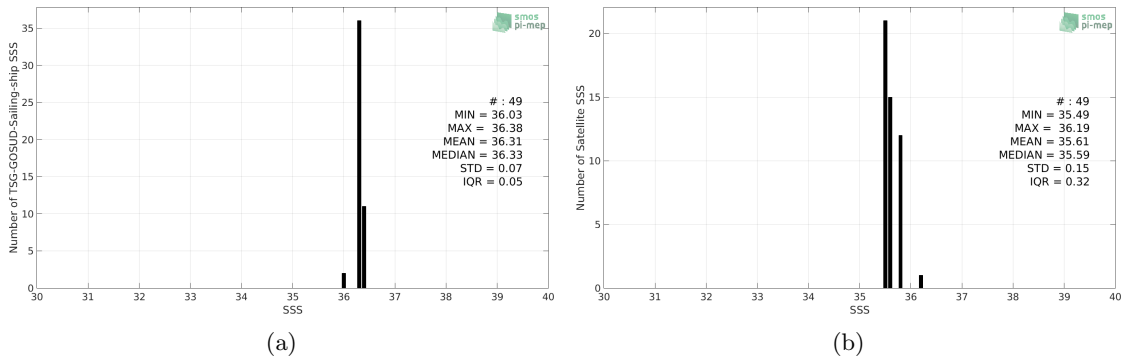
Figure 2: Histograms of SSS from TSG-GOSUD-Sailing-ship (a) and SMOS-L3-CATDS-CECOS-LOCEAN-V3-9DAYS-25KM (b) considering all match-up pairs per bins of 0.1 over the Gulf of Mexico Pi-MEP region and for the full satellite product period.
