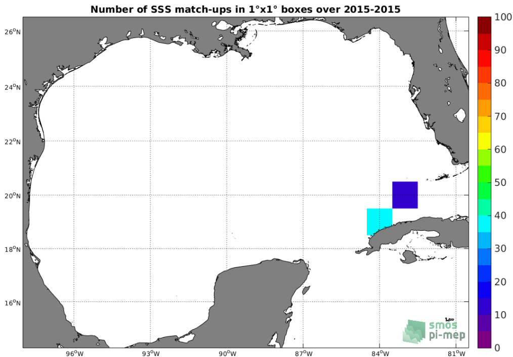
Figure 4: Number of SSS match-ups between TSG-GOSUD-Sailing-ship SSS and the SMOS-L3-CATDS-CECOS-LOCEAN-V3-9DAYS-25KM SSS product for the Gulf of Mexico Pi-MEP region over 1^\circ \times 1^\circ boxes and for the full satellite product period.
