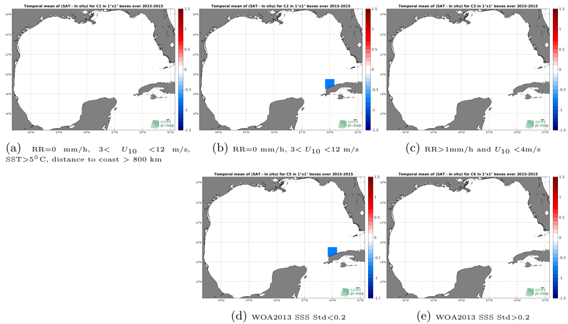
Figure 12: Temporal mean gridded over spatial boxes of size 1^\circ \times 1^\circ of \Delta SSS (SMOS-L3-CATDS-CECOS-LOCEAN-V3-9DAYS-25KM - TSG-GOSUD-Sailing-ship) for 5 different subdatasets corresponding to:RR=0 mm/h, 3 < U_{10} < 12 m/s, SST >5^\circ\text{C} , distance to coast > 800 km (a), RR=0 mm/h, 3 < U_{10} < 12 m/s (b), RR >1 mm/h and U_{10} < 4 m/s (c), WOA2013 SSS Std <0.2 (d), WOA2013 SSS Std >0.2 (e).
