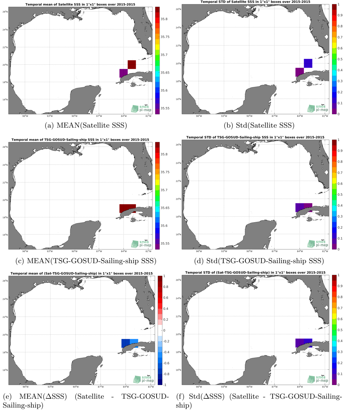
Figure 6: Temporal mean (left) and Std (right) of SSS from SMOS-L3-CATDS-CECOS-LOCEAN-V3-9DAYS-25KM (top), TSG-GOSUD-Sailing-ship (middle), and of \Delta SSS (Satellite - TSG-GOSUD-Sailing-ship). Only match-up pairs are used to generate these maps.
