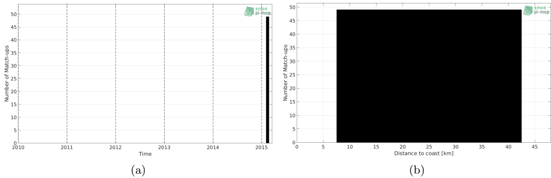
Figure 1: Number of match-ups between TSG-GOSUD-Sailing-ship and SMOS-L3-CATDS-CECOS-LOCEAN-V3-9DAYS-25KM SSS as a function of time (a) and as function of the distance to coast (b) over the Gulf of Mexico Pi-MEP region and for the full satellite product period.
