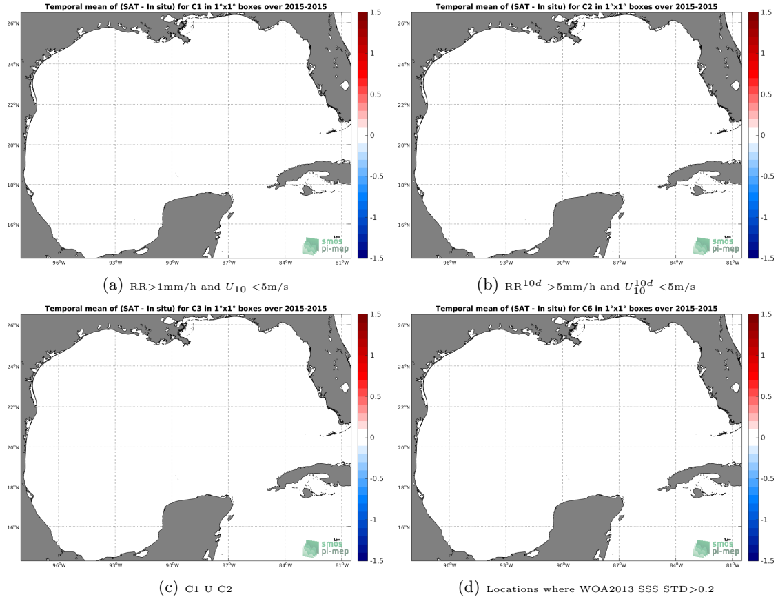
Figure 12: Temporal mean gridded over spatial boxes of size 1^\circ \times 1^\circ of \Delta\text{SSS} (SMOS-L3-CATDS-CECOS-LOCEAN-V3-9DAYS-25KM - TSG-GOSUD-Sailing-ship) for 4 different subdatasets corresponding to: RR > 1\text{mm/h} and U_{10} < 5\text{m/s} (a), RR^{10d} > 5\text{mm/h} and U_{10}^{10d} < 5\text{m/s} (b), C1 U C2 (c), Locations where WOA2013 SSS STD > 0.2 (d).
