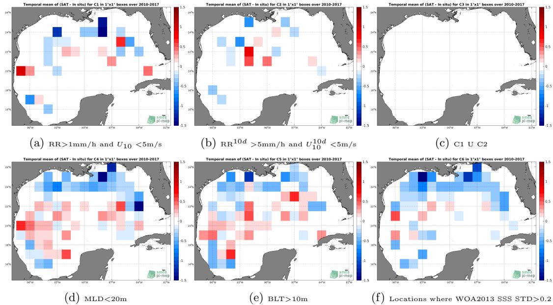
Figure 12: Temporal mean gridded over spatial boxes of size 1^\circ \times 1^\circ of \Delta\text{SSS} (SMOS-L3-CATDS-CECOS-LOCEAN-V3-9DAYS-25KM - Argo) for 6 different subdatasets corresponding to: RR > 1\text{mm/h} and U_{10} < 5\text{m/s} (a), RR^{10d} > 5\text{mm/h} and U_{10}^{10d} < 5\text{m/s} (b), C1 U C2 (c), MLD < 20\text{m} (d), BLT > 10\text{m} (e), Locations where WOA2013 SSS STD > 0.2 (f).
