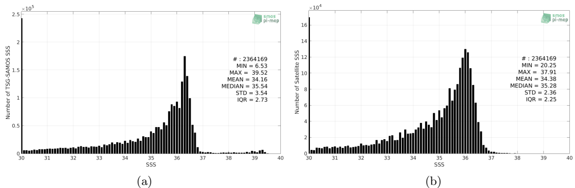
Figure 2: Histograms of SSS from TSG-SAMOS (a) and SMOS-L3-CATDS-CECOS-LOCEAN-V3-18DAYS-25KM (b) considering all match-up pairs per bins of 0.1 over the Gulf of Mexico Pi-MEP region and for the full satellite product period.
