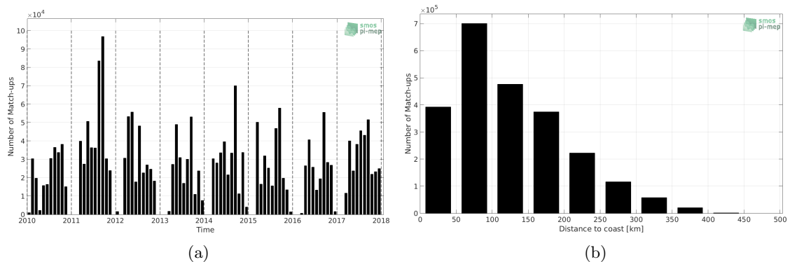
Figure 1: Number of match-ups between TSG-SAMOS and SMOS-L3-CATDS-CECOS-LOCEAN-V3-18DAYS-25KM SSS as a function of time (a) and as function of the distance to coast (b) over the Gulf of Mexico Pi-MEP region and for the full satellite product period.
