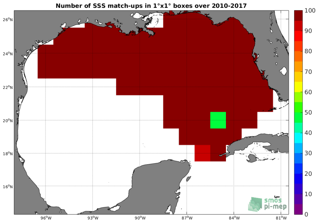
Figure 4: Number of SSS match-ups between TSG-SAMOS SSS and the SMOS-L3-CATDS-CECOS-LOCEAN-V3-18DAYS-25KM SSS product for the Gulf of Mexico Pi-MEP region over 1°x1° boxes and for the full satellite product period.
