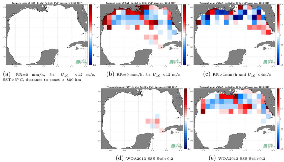
Figure 12: Temporal mean gridded over spatial boxes of size 1^\circ \times 1^\circ of \Delta SSS (SMOS-L3-CATDS-CECOS-LOCEAN-V3-18DAYS-25KM - TSG-SAMOS) for 5 different subdatasets corresponding to:RR=0 mm/h, 3 < U_{10} < 12 m/s, SST >5^\circ C, distance to coast > 800 km (a), RR=0 mm/h, 3 < U_{10} < 12 m/s (b), RR >1 mm/h and U_{10} < 4 m/s (c), WOA2013 SSS Std <0.2 (d), WOA2013 SSS Std >0.2 (e).
