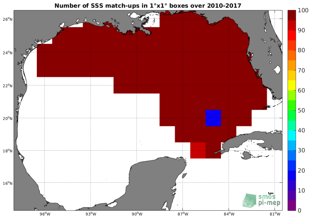
Figure 4: Number of SSS match-ups between TSG-SAMOS SSS and the SMOS-L3-CATDS-CECOS-LOCEAN-V3-18DAYS-25KM SSS product for the Gulf of Mexico Pi-MEP region over 1^\circ \times 1^\circ boxes and for the full satellite product period.
