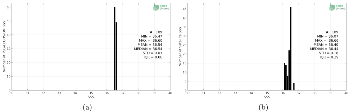
Figure 2: Histograms of SSS from TSG-LEGOS-DM (a) and SMOS-L3-CATDS-CECOS-LOCEAN-V3-18DAYS-25KM (b) considering all match-up pairs per bins of 0.1 over the Gulf of Mexico Pi-MEP region and for the full satellite product period.
