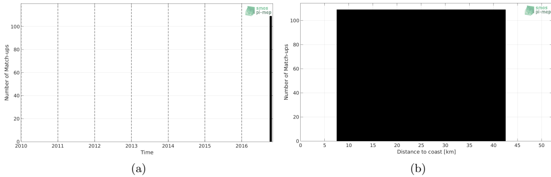
Figure 1: Number of match-ups between TSG-LEGOS-DM and SMOS-L3-CATDS-CECOS-LOCEAN-V3-18DAYS-25KM SSS as a function of time (a) and as function of the distance to coast (b) over the Gulf of Mexico Pi-MEP region and for the full satellite product period.
