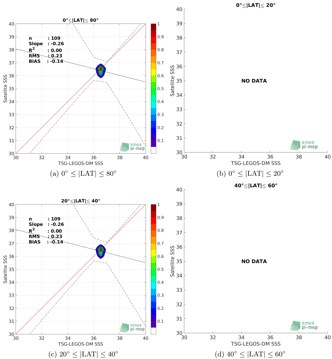
Figure 9: Contour maps of the concentration of SMOS-L3-CATDS-CECOS-LOCEAN-V3-18DAYS-25KM SSS (y-axis) versus TSG-LEGOS-DM SSS (x-axis) at match-up pairs for different latitude bands. For each plot, the red line shows x=y . The black thin and dashed lines indicate a linear fit through the data cloud and the \pm 95\% confidence levels, respectively. The number match-up pairs n , the slope and R^2 coefficient of the linear fit, the root mean square (RMS) and the mean bias between satellite and in situ data are indicated for each latitude band in each plots.
