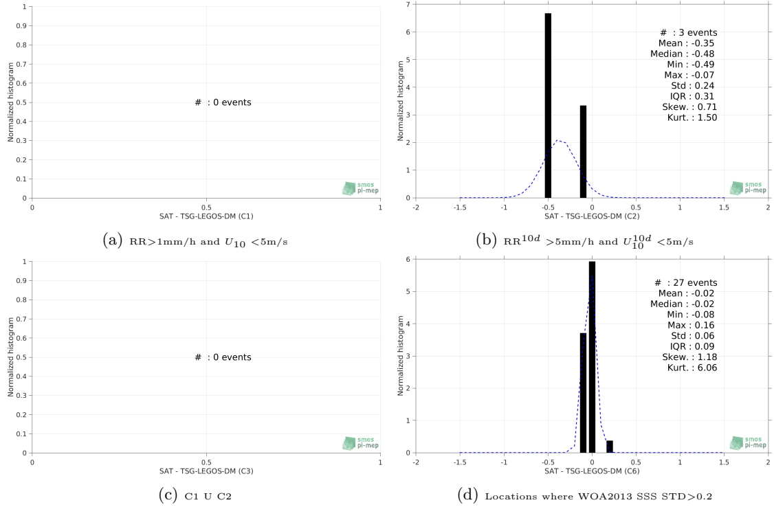
Figure 13: Normalized histogram of \Delta\text{SSS} (SMOS-L3-CATDS-CECOS-LOCEAN-V3-18DAYS-25KM - TSG-LEGOS-DM) for 6 different subdatasets corresponding to: RR > 1\text{mm/h} and U_{10} < 5\text{m/s} (a), RR^{10d} > 5\text{mm/h} and U_{10}^{10d} < 5\text{m/s} (b), C1 U C2 (c), Locations where WOA2013 SSS STD > 0.2 (d).
