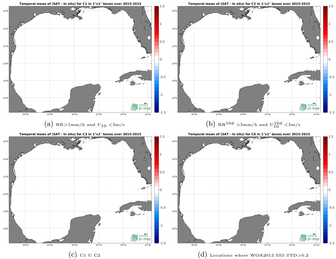
Figure 12: Temporal mean gridded over spatial boxes of size 1^\circ \times 1^\circ of \Delta SSS (SMOS-L3-CATDS-CECOS-LOCEAN-V3-18DAYS-25KM - TSG-GOSUD-Sailing-ship) for 4 different subdatasets corresponding to: RR > 1\text{mm/h} and U_{10} < 5\text{m/s} (a), RR^{10d} > 5\text{mm/h} and U_{10}^{10d} < 5\text{m/s} (b), C1 U C2 (c), Locations where WOA2013 SSS STD > 0.2 (d).
