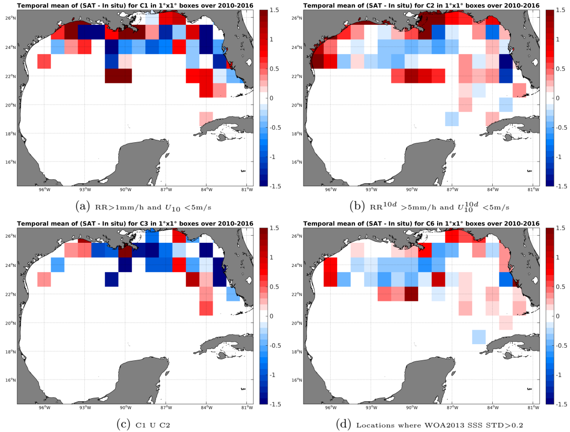
Figure 12: Temporal mean gridded over spatial boxes of size 1°x1° of \Delta SSS (SMOS-L3-CATDS-CECOS-LOCEAN-V2-9DAYS-25KM - TSG-SAMOS) for 4 different subdatasets corresponding to: RR > 1mm/h and U_{10} < 5m/s (a), RR 10d > 5mm/h and U_{10}^{10d} < 5m/s (b), C1 U C2 (c), Locations where WOA2013 SSS STD > 0.2 (d).
