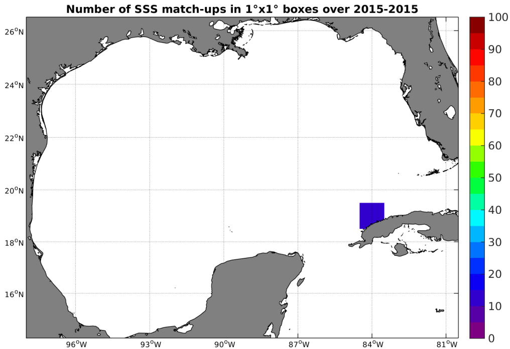
Figure 4: Number of SSS match-ups between TSG-GOSUD-Sailing-ship SSS and the SMOS-L3-CATDS-CECOS-LOCEAN-V2-9DAYS-25KM SSS product for the Gulf of Mexico Pi-MEP region over 1^\circ \times 1^\circ boxes and for the full satellite product period.
