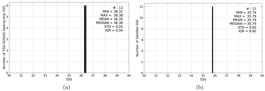
Figure 2: Histograms of SSS from TSG-GOSUD-Sailing-ship (a) and SMOS-L3-CATDS-CECOS-LOCEAN-V2-9DAYS-25KM (b) considering all match-up pairs per bins of 0.1 over the Gulf of Mexico Pi-MEP region and for the full satellite product period.
