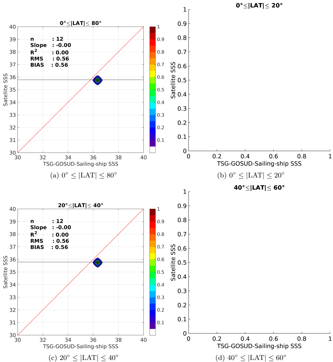
Figure 9: Contour maps of the concentration of SMOS-L3-CATDS-CECOS-LOCEAN-V2-9DAYS-25KM SSS (y-axis) versus TSG-GOSUD-Sailing-ship SSS (x-axis) at match-up pairs for different latitude bands. For each plot, the red line shows x=y . The black thin and dashed lines indicate a linear fit through the data cloud and the \pm 95\% confidence levels, respectively. The number match-up pairs n , the slope and R^2 coefficient of the linear fit, the root mean square (RMS) and the mean bias between satellite and in situ data are indicated for each latitude band in each plots.
