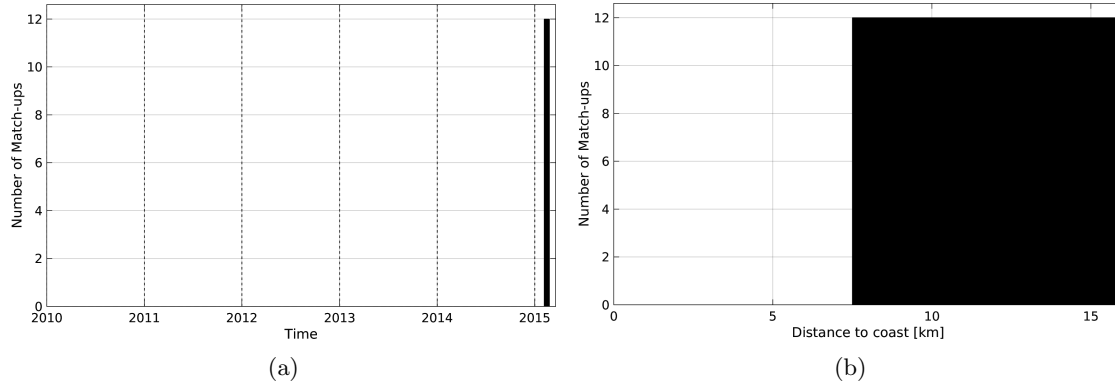
Figure 1: Number of match-ups between TSG-GOSUD-Sailing-ship and SMOS-L3-CATDS-CECOS-LOCEAN-V2-9DAYS-25KM SSS as a function of time (a) and as function of the distance to coast (b) over the Gulf of Mexico Pi-MEP region and for the full satellite product period.
