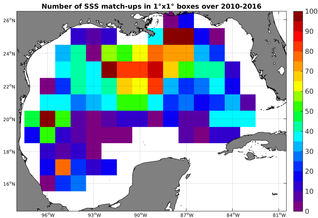
Figure 4: Number of SSS match-ups between Argo SSS and the SMOS-L3-CATDS-CECOS-LOCEAN-V2-9DAYS-25KM SSS product for the Gulf of Mexico Pi-MEP region over 1^\circ \times 1^\circ boxes and for the full satellite product period.
