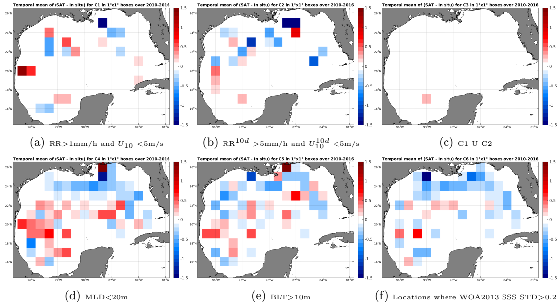
Figure 12: Temporal mean gridded over spatial boxes of size 1^\circ \times 1^\circ of \Delta SSS (SMOS-L3-CATDS-CECOS-LOCEAN-V2-9DAYS-25KM - Argo) for 6 different subdatasets corresponding to: RR > 1mm/h and U_{10} < 5\text{m/s} (a), RR^{10d} > 5\text{mm/h} and U_{10}^{10d} < 5\text{m/s} (b), C1 U C2 (c), MLD < 20m (d), BLT > 10m (e), Locations where WOA2013 SSS STD > 0.2 (f).
