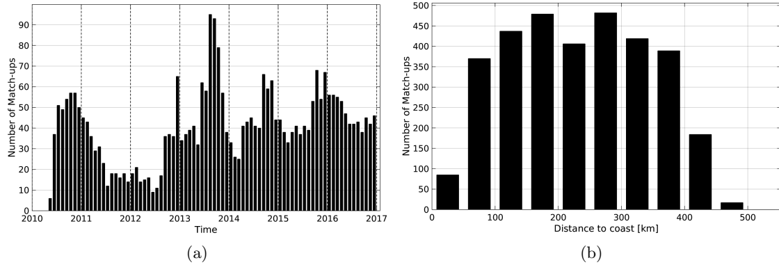
Figure 1: Number of match-ups between Argo and SMOS-L3-CATDS-CECOS-LOCEAN-V2-9DAYS-25KM SSS as a function of time (a) and as function of the distance to coast (b) over the Gulf of Mexico Pi-MEP region and for the full satellite product period.
