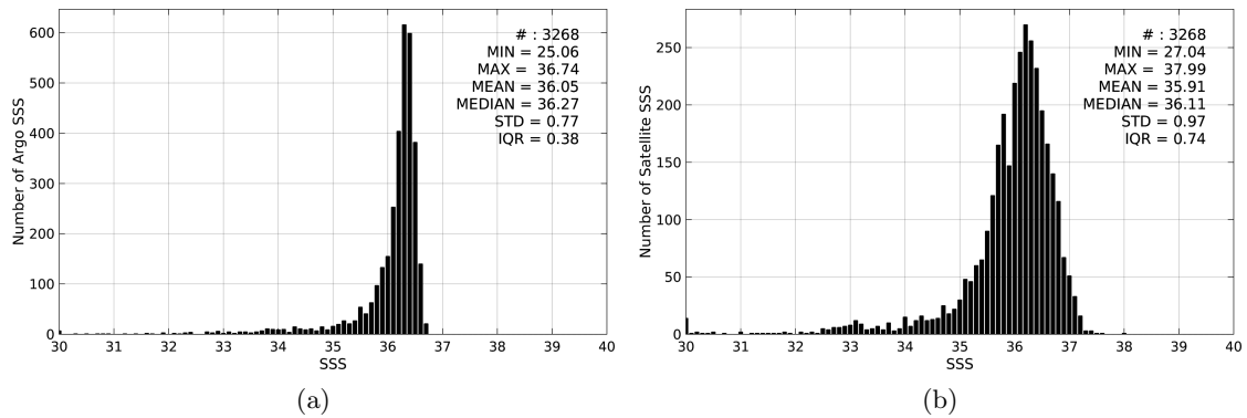
Figure 2: Histograms of SSS from Argo (a) and SMOS-L3-CATDS-CECOS-LOCEAN-V2-9DAYS-25KM (b) considering all match-up pairs per bins of 0.1 over the Gulf of Mexico Pi-MEP region and for the full satellite product period.
