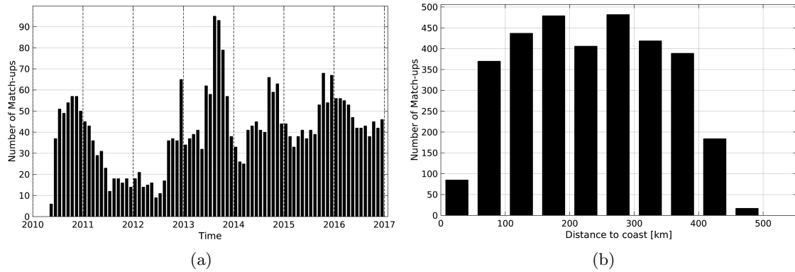
Figure 1: Number of match-ups between Argo and SMOS-L3-CATDS-CECOS-LOCEAN-V2-9DAYS-25KM SSS as a function of time (a) and as function of the distance to coast (b) over the Gulf of Mexico Pi-MEP region and for the full satellite product period.
