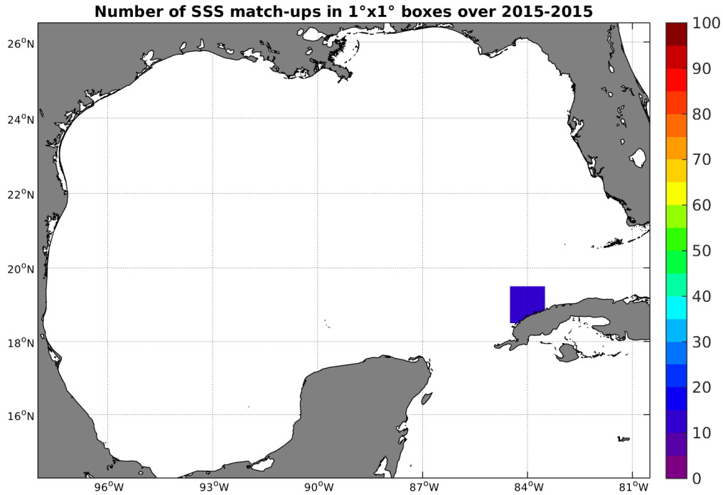
Figure 4: Number of SSS match-ups between TSG-GOSUD-Sailing-ship SSS and the SMOS-L3-CATDS-CECOS-LOCEAN-V2-18DAYS-25KM SSS product for the Gulf of Mexico Pi-MEP region over 1^\circ \times 1^\circ boxes and for the full satellite product period.
