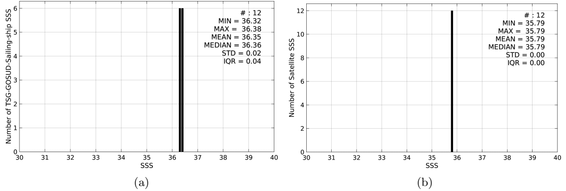
Figure 2: Histograms of SSS from TSG-GOSUD-Sailing-ship (a) and SMOS-L3-CATDS-CECOS-LOCEAN-V2-18DAYS-25KM (b) considering all match-up pairs per bins of 0.1 over the Gulf of Mexico Pi-MEP region and for the full satellite product period.
