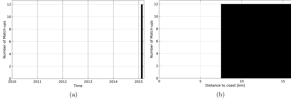
Figure 1: Number of match-ups between TSG-GOSUD-Sailing-ship and SMOS-L3-CATDS-CECOS-LOCEAN-V2-18DAYS-25KM SSS as a function of time (a) and as function of the distance to coast (b) over the Gulf of Mexico Pi-MEP region and for the full satellite product period.
