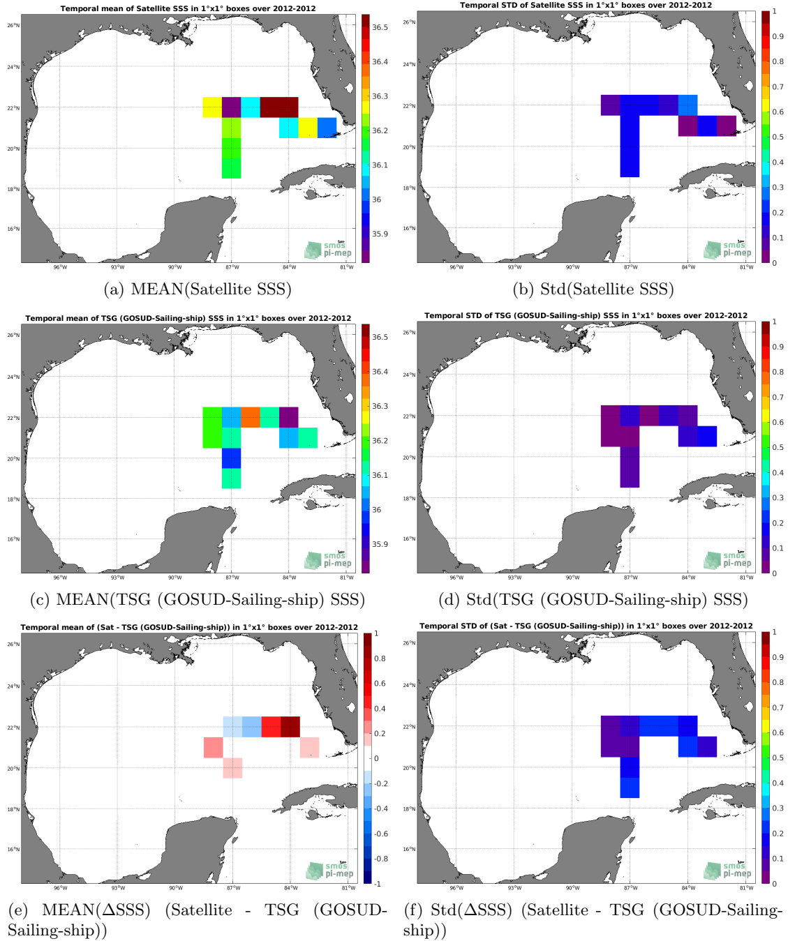
Figure 6: Temporal mean (left) and Std (right) of SSS from SMOS SSS L3 v2 - Monthly - 0.25 Deg (CATDS-CECOS-IFREMER) (top), TSG (GOSUD-Sailing-ship) (middle), and of \Delta SSS (Satellite - TSG (GOSUD-Sailing-ship)). Only match-up pairs are used to generate these maps.
