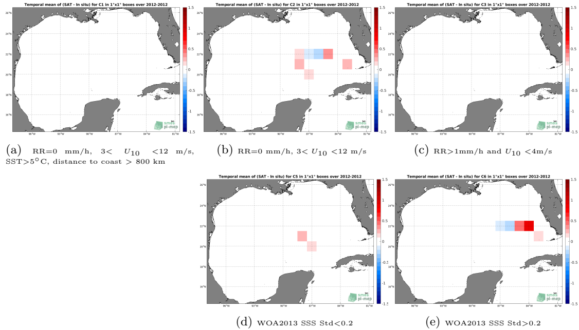
Figure 12: Temporal mean gridded over spatial boxes of size 1^\circ \times 1^\circ of \Delta SSS (SMOS SSS L3 v2 - Monthly - 0.25 Deg (CATDS-CECOS-IFREMER) - TSG (GOSUD-Sailing-ship)) for 5 different subdatasets corresponding to: RR=0 mm/h, 3 < U_{10} < 12 m/s, SST >5^\circ\text{C} , distance to coast > 800 km (a), RR=0 mm/h, 3 < U_{10} < 12 m/s (b), RR >1 mm/h and U_{10} < 4 m/s (c), WOA2013 SSS Std <0.2 (d), WOA2013 SSS Std >0.2 (e).
