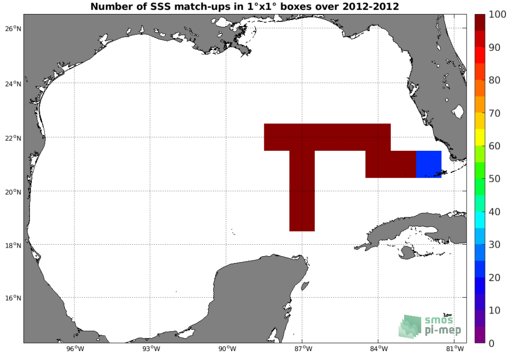
Figure 4: Number of SSS match-ups between TSG (GOSUD-Sailing-ship) SSS and the SMOS SSS L3 v2 - Monthly - 0.25 Deg (CATDS-CECOS-IFREMER) SSS product for the Gulf of Mexico Pi-MEP region over 1^\circ \times 1^\circ boxes and for the full satellite product period.
