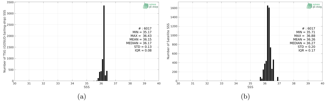
Figure 2: Histograms of SSS from TSG (GOSUD-Sailing-ship) (a) and SMOS SSS L3 v2 - Monthly - 0.25 Deg (CATDS-CECOS-IFREMER) (b) considering all match-up pairs per bins of 0.1 over the Gulf of Mexico Pi-MEP region and for the full satellite product period.
