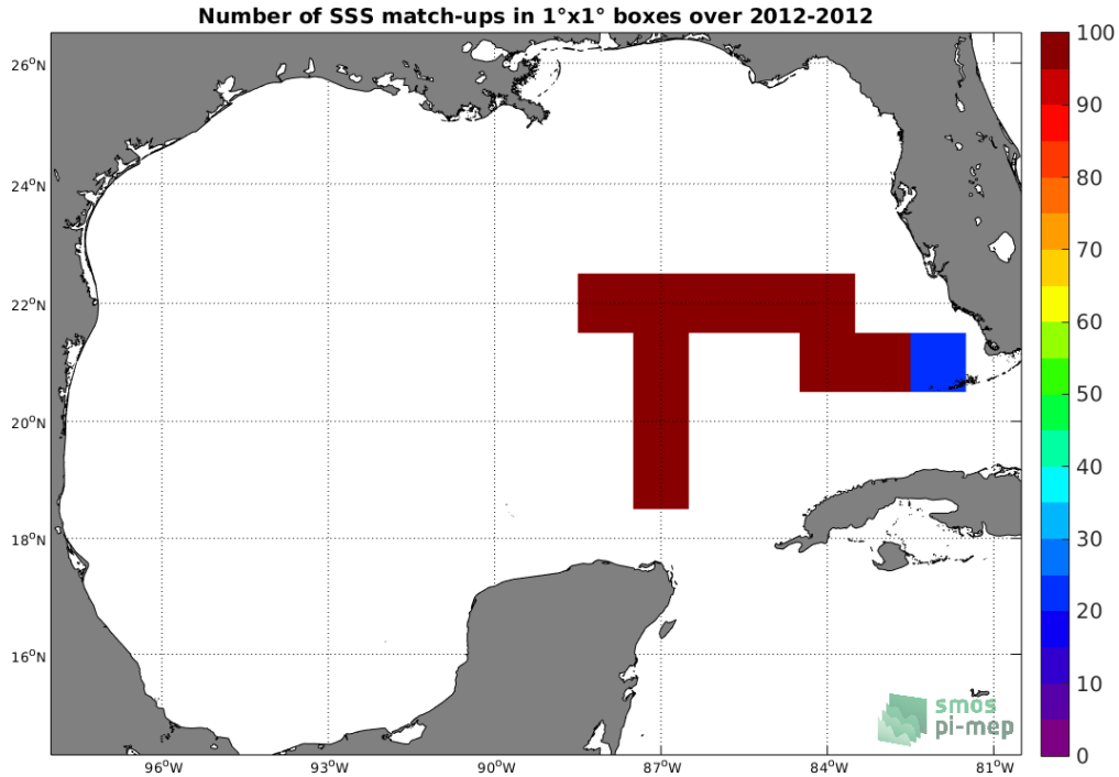
Figure 4: Number of SSS match-ups between TSG (GOSUD-Sailing-ship) SSS and the SMOS SSS L3 v2 - Monthly - 0.25 Deg (CATDS-CECOS-IFREMER) SSS product for the Gulf of Mexico Pi-MEP region over 1°x1° boxes and for the full satellite product period.
