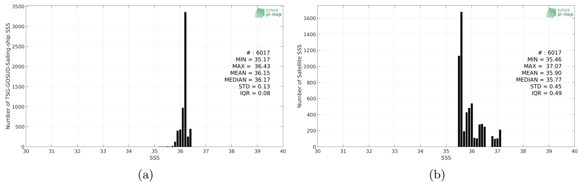
Figure 2: Histograms of SSS from TSG-GOSUD-Sailing-ship (a) and SMOS L3 v2 - Monthly - 0.25 Deg (CATDS-CECOS-IFREMER) (b) considering all match-up pairs per bins of 0.1 over the Gulf of Mexico Pi-MEP region and for the full satellite product period.
