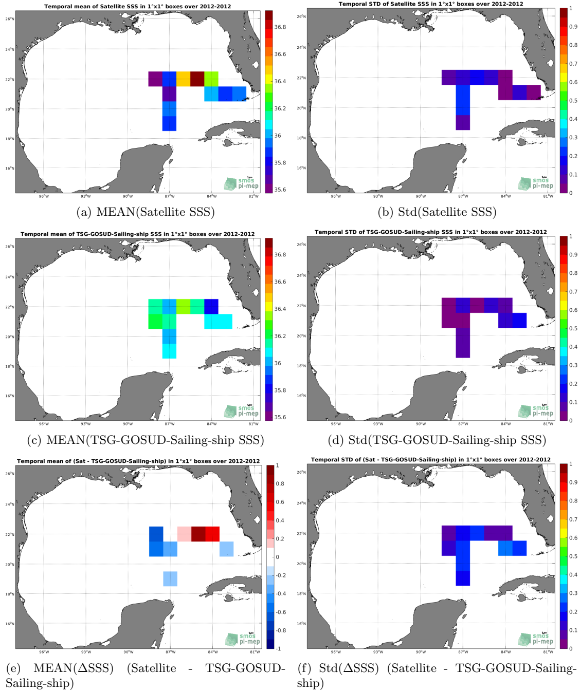
Figure 6: Temporal mean (left) and Std (right) of SSS from SMOS L3 v2 - Monthly - 0.25 Deg (CATDS-CECOS-IFREMER) (top), TSG-GOSUD-Sailing-ship (middle), and of \Delta SSS (Satellite - TSG-GOSUD-Sailing-ship). Only match-up pairs are used to generate these maps.
