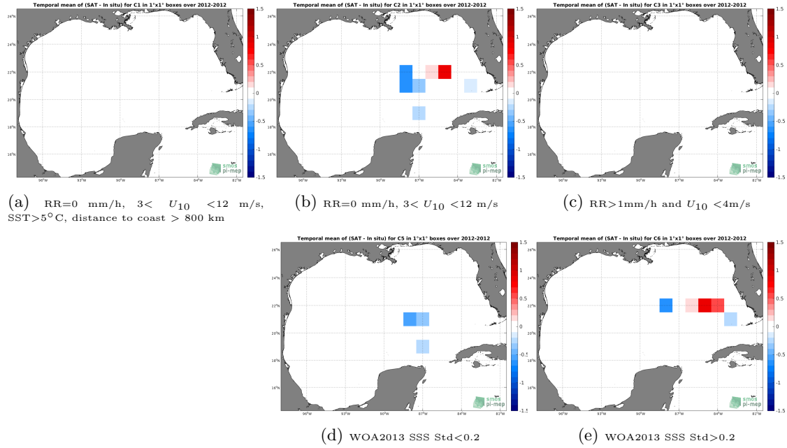
Figure 12: Temporal mean gridded over spatial boxes of size 1^{\circ}\times 1^{\circ} of \Delta SSS (SMOS L3 v2 - Monthly - 0.25 Deg (CATDS-CECOS-IFREMER) - TSG-GOSUD-Sailing-ship) for 5 different subdatasets corresponding to:RR=0 mm/h, 3 < U_{10} < 12 m/s, SST >5^{\circ}\text{C} , distance to coast > 800 km (a), RR=0 mm/h, 3 < U_{10} < 12 m/s (b), RR >1 mm/h and U_{10} < 4 m/s (c), WOA2013 SSS Std <0.2 (d), WOA2013 SSS Std >0.2 (e).
