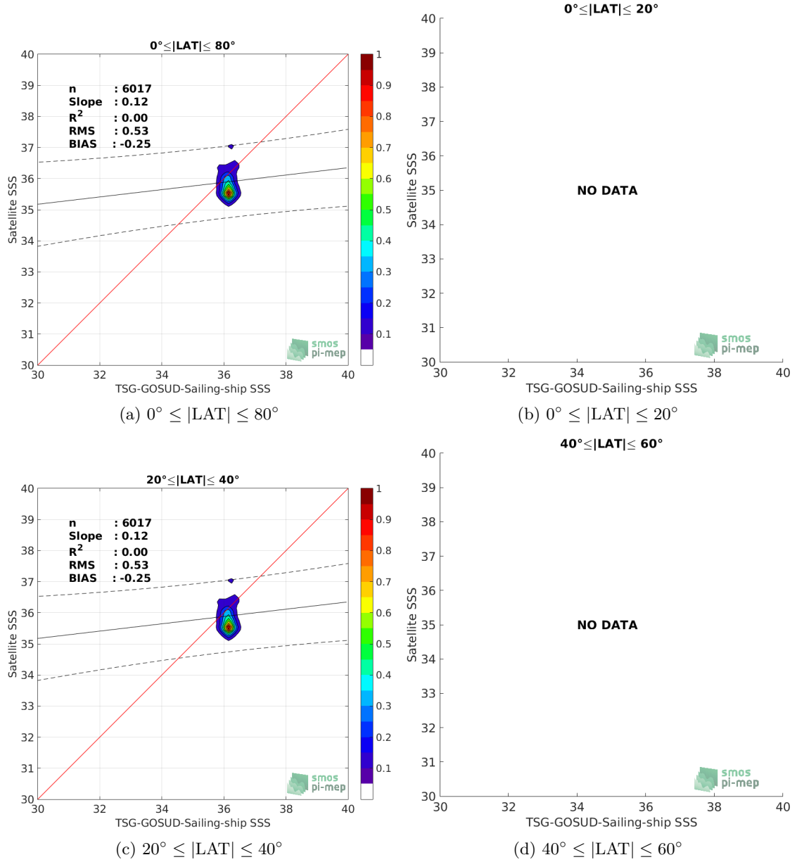
Figure 9: Contour maps of the concentration of SMOS L3 v2 - Monthly - 0.25 Deg (CATDS-CECOS-IFREMER) SSS (y-axis) versus TSG-GOSUD-Sailing-ship SSS (x-axis) at match-up pairs for different latitude bands. For each plot, the red line shows x=y . The black thin and dashed lines indicate a linear fit through the data cloud and the \pm 95\% confidence levels, respectively. The number match-up pairs n , the slope and R^2 coefficient of the linear fit, the root mean square (RMS) and the mean bias between satellite and in situ data are indicated for each latitude band in each plots.
