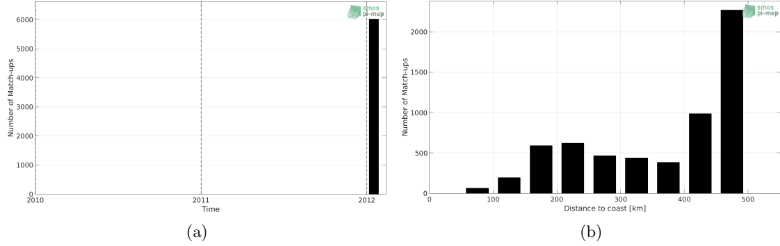
Figure 1: Number of match-ups between TSG-GOSUD-Sailing-ship and SMOS L3 v2 - Monthly - 0.25 Deg (CATDS-CECOS-IFREMER) SSS as a function of time (a) and as function of the distance to coast (b) over the Gulf of Mexico Pi-MEP region and for the full satellite product period.
