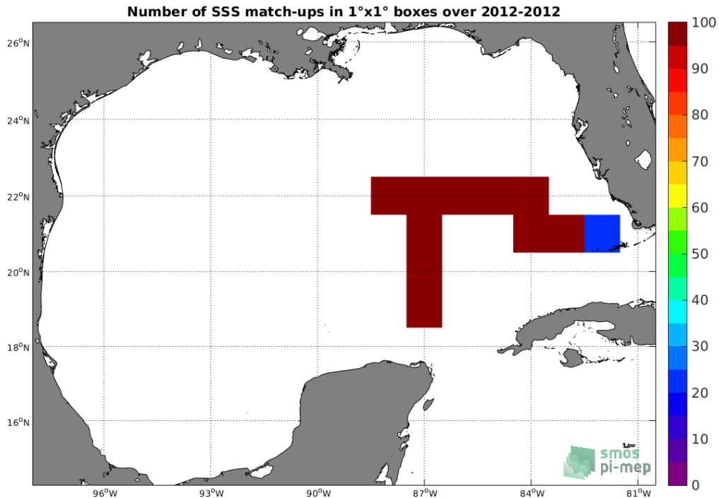
Figure 4: Number of SSS match-ups between TSG-GOSUD-Sailing-ship SSS and the SMOS L3 v2 - Monthly - 0.25 Deg (CATDS-CECOS-IFREMER) SSS product for the Gulf of Mexico Pi-MEP region over 1°x1° boxes and for the full satellite product period.
