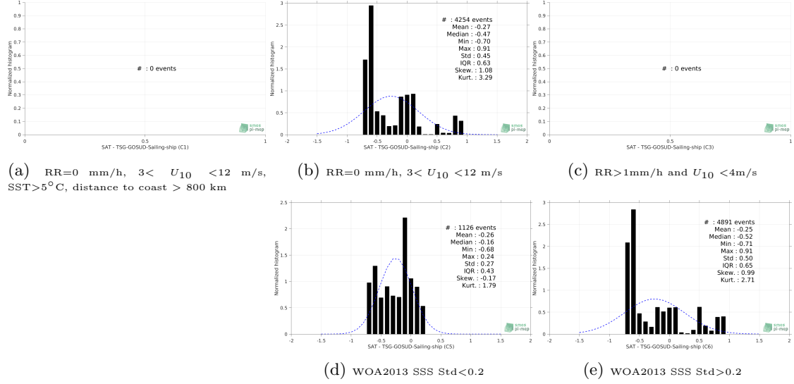
Figure 13: Normalized histogram of \Delta\text{SSS} (SMOS L3 v2 - Monthly - 0.25 Deg (CATDS-CECOS-IFREMER) - TSG-GOSUD-Sailing-ship) for 5 different subdatasets corresponding to: RR=0 mm/h, 3 < U_{10} < 12 m/s, SST > 5^\circ\text{C} , distance to coast > 800 km (a), RR=0 mm/h, 3 < U_{10} < 12 m/s (b), RR > 1\text{mm/h} and U_{10} < 4\text{m/s} (c), WOA2013 SSS Std < 0.2 (d), WOA2013 SSS Std > 0.2 (e).
