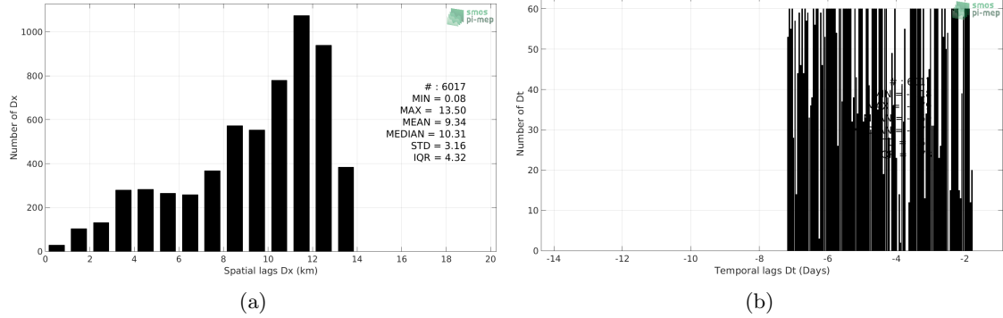
Figure 5: Histograms of the spatial (a) and temporal (b) lags between the time of the TSG-GOSUD-Sailing-ship measurements and the date of the corresponding SMOS L3 v2 - Monthly - 0.25 Deg (CATDS-CECOS-IFREMER) SSS product.
