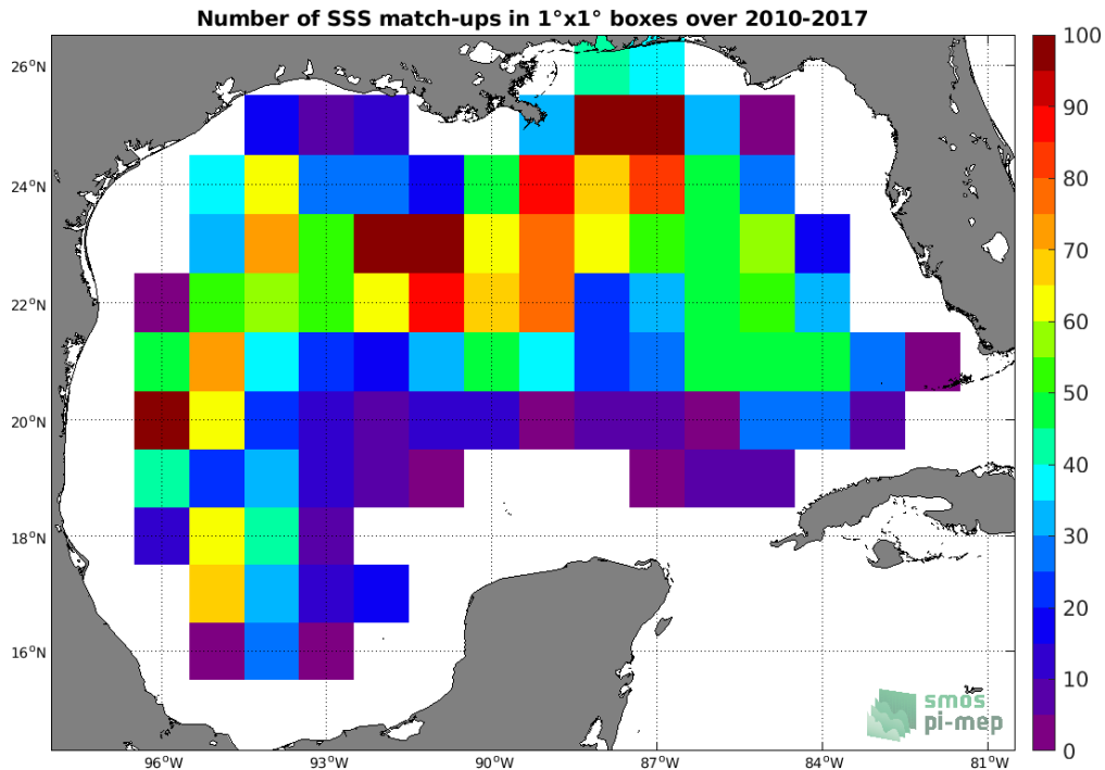
Figure 4: Number of SSS match-ups between Argo SSS and the SMOS SSS L3 v2 - Monthly - 0.25 Deg (CATDS-CECOS-IFREMER) SSS product for the Gulf of Mexico Pi-MEP region over 1°x1° boxes and for the full satellite product period.
