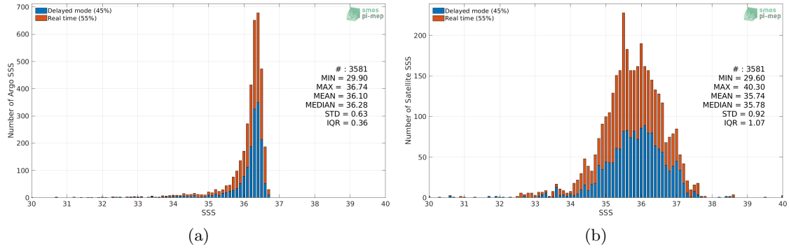
Figure 2: Histograms of SSS from Argo (a) and SMOS SSS L3 v2 - Monthly - 0.25 Deg (CATDS-CECOS-IFREMER) (b) considering all match-up pairs per bins of 0.1 over the Gulf of Mexico Pi-MEP region and for the full satellite product period.
