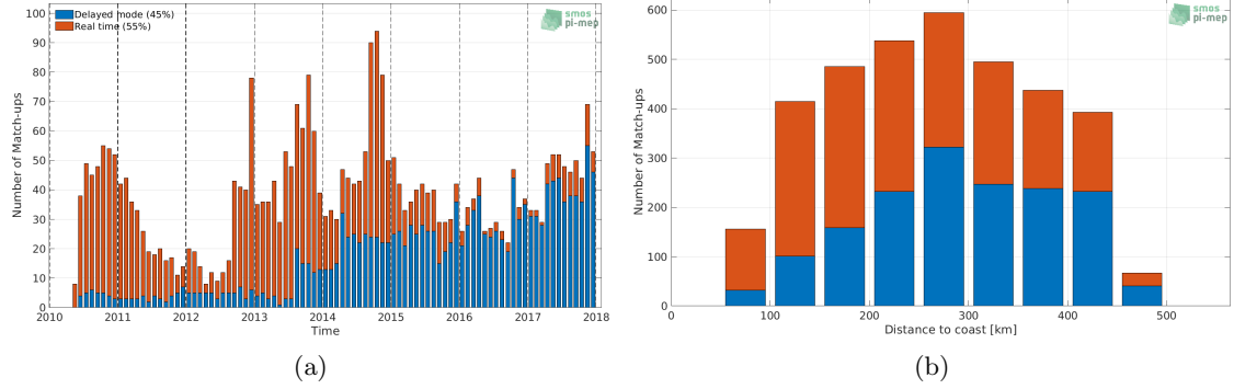
Figure 1: Number of match-ups between Argo and SMOS SSS L3 v2 - Monthly - 0.25 Deg (CATDS-CECOS-IFREMER) SSS as a function of time (a) and as function of the distance to coast (b) over the Gulf of Mexico Pi-MEP region and for the full satellite product period.
