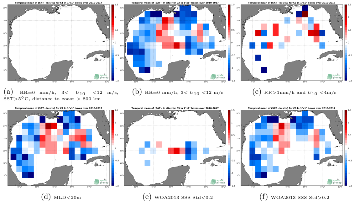
Figure 12: Temporal mean gridded over spatial boxes of size 1^\circ \times 1^\circ of \Delta SSS (SMOS SSS L3 v2 - Monthly - 0.25 Deg (CATDS-CECOS-IFREMER) - Argo) for 6 different subdatasets corresponding to:RR=0 mm/h, 3 < U_{10} < 12 m/s, SST >5^\circ C, distance to coast > 800 km (a), RR=0 mm/h, 3 < U_{10} < 12 m/s (b), RR >1 mm/h and U_{10} < 4 m/s (c),MLD <20 m (d),WOA2013 SSS Std <0.2 (e),WOA2013 SSS Std >0.2 (f).
