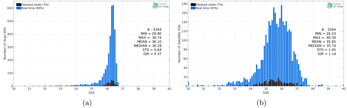
Figure 2: Histograms of SSS from Argo (a) and SMOS L3 v2 - Monthly - 0.25 Deg (CATDS-CECOS-IFREMER) (b) considering all match-up pairs per bins of 0.1 over the Gulf of Mexico Pi-MEP region and for the full satellite product period.
