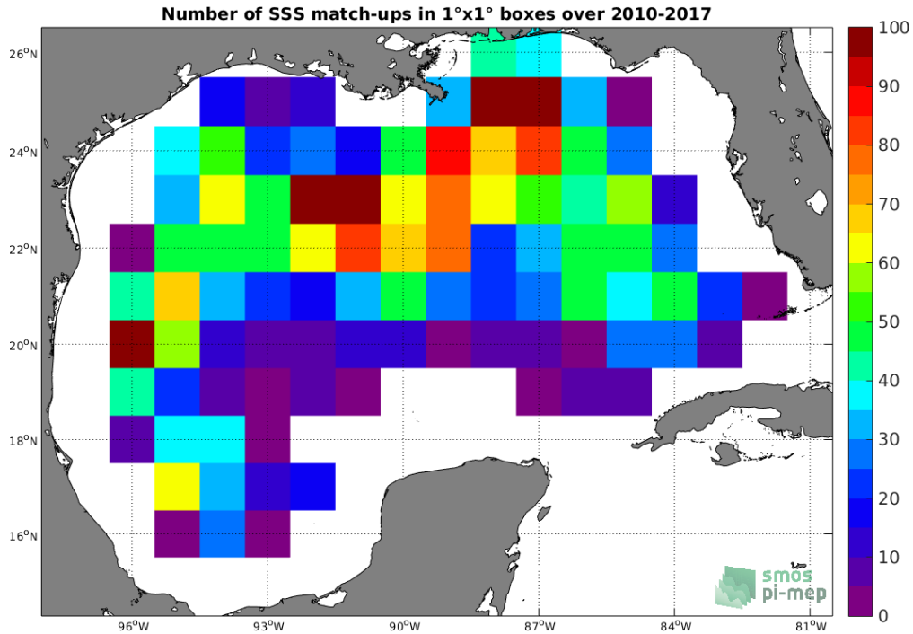
Figure 4: Number of SSS match-ups between Argo SSS and the SMOS L3 v2 - Monthly - 0.25 Deg (CATDS-CECOS-IFREMER) SSS product for the Gulf of Mexico Pi-MEP region over 1°x1° boxes and for the full satellite product period.
