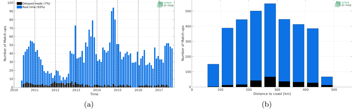
Figure 1: Number of match-ups between Argo and SMOS L3 v2 - Monthly - 0.25 Deg (CATDS-CECOS-IFREMER) SSS as a function of time (a) and as function of the distance to coast (b) over the Gulf of Mexico Pi-MEP region and for the full satellite product period.
