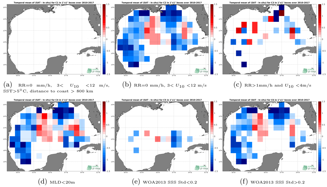
Figure 12: Temporal mean gridded over spatial boxes of size 1^\circ \times 1^\circ of \Delta SSS (SMOS L3 v2 - Monthly - 0.25^\circ Deg (CATDS-CECOS-IFREMER) - Argo) for 6 different subdatasets corresponding to: RR=0 mm/h, 3 < U_{10} < 12 m/s, SST >5^\circ C, distance to coast > 800 km (a), RR=0 mm/h, 3 < U_{10} < 12 m/s (b), RR >1 mm/h and U_{10} < 4 m/s (c),MLD <20 m (d),WOA2013 SSS Std <0.2 (e),WOA2013 SSS Std >0.2 (f).
