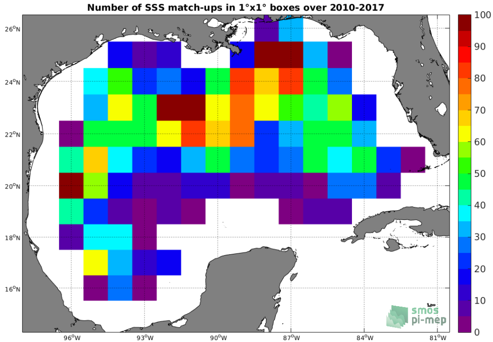
Figure 4: Number of SSS match-ups between Argo SSS and the SMOS-L3-CATDS-IFREMER-CECOS-V2-MONTHLY-0.25DEG SSS product for the Gulf of Mexico Pi-MEP region over 1^\circ \times 1^\circ boxes and for the full satellite product period.
