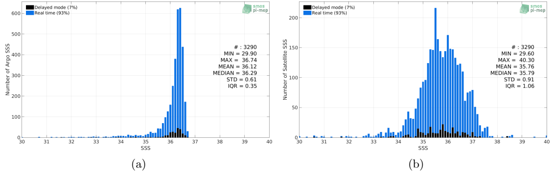
Figure 2: Histograms of SSS from Argo (a) and SMOS-L3-CATDS-IFREMER-CECOS-V2-MONTHLY-0.25DEG (b) considering all match-up pairs per bins of 0.1 over the Gulf of Mexico Pi-MEP region and for the full satellite product period.
