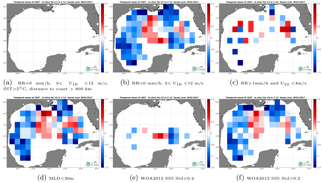
Figure 12: Temporal mean gridded over spatial boxes of size 1^\circ \times 1^\circ of \Delta SSS (SMOS-L3-CATDS-IFREMER-CECOS-V2-MONTHLY-0.25DEG - Argo) for 6 different subdatasets corresponding to:RR=0 mm/h, 3 < U_{10} < 12 m/s, SST >5^\circ C, distance to coast > 800 km (a), RR=0 mm/h, 3 < U_{10} < 12 m/s (b), RR >1 mm/h and U_{10} < 4 m/s (c),MLD <20 m (d),WOA2013 SSS Std <0.2 (e),WOA2013 SSS Std >0.2 (f).
