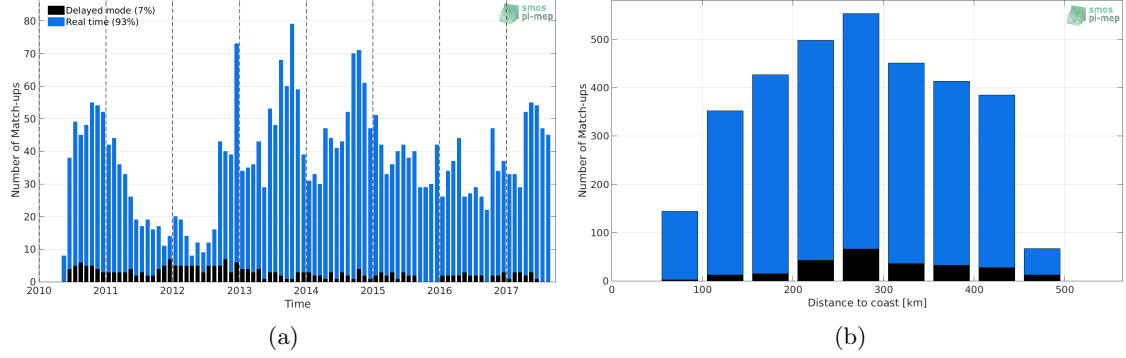
Figure 1: Number of match-ups between Argo and SMOS-L3-CATDS-IFREMER-CECOS-V2-MONTHLY-0.25DEG SSS as a function of time (a) and as function of the distance to coast (b) over the Gulf of Mexico Pi-MEP region and for the full satellite product period.
