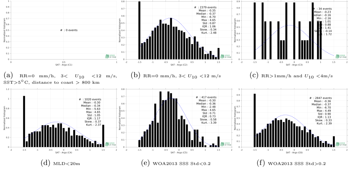
Figure 13: Normalized histogram of \Delta\text{SSS} (SMOS-L3-CATDS-IFREMER-CECOS-V2-MONTHLY-0.25DEG - Argo) for 6 different subdatasets corresponding to: RR=0 mm/h, 3 < U_{10} < 12 m/s, SST > 5^\circ\text{C} , distance to coast > 800 km (a), RR=0 mm/h, 3 < U_{10} < 12 m/s (b), RR > 1 mm/h and U_{10} < 4 m/s (c), MLD < 20 m (d), WOA2013 SSS Std < 0.2 (e), WOA2013 SSS Std > 0.2 (f).
