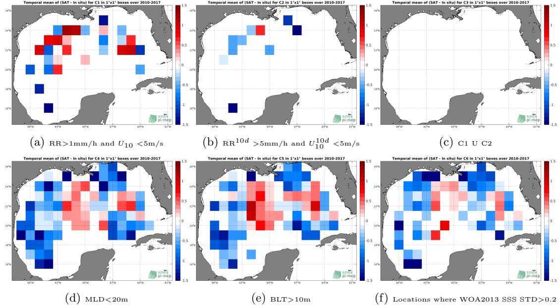
Figure 12: Temporal mean gridded over spatial boxes of size 1^\circ \times 1^\circ of \Delta\text{SSS} (SMOS-L3-CATDS-IFREMER-CECOS-V2-MONTHLY-0.25DEG - Argo) for 6 different subdatasets corresponding to: RR > 1\text{mm/h} and U_{10} < 5\text{m/s} (a), RR^{10d} > 5\text{mm/h} and U_{10}^{10d} < 5\text{m/s} (b), C1 U C2 (c), MLD < 20\text{m} (d), BLT > 10\text{m} (e), Locations where WOA2013 SSS STD > 0.2 (f).
