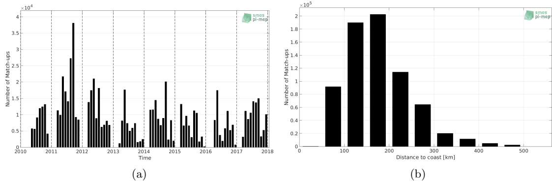
Figure 1: Number of match-ups between TSG (SAMOS) and SMOS SSS L3 v2 - Daily - 0.5 Deg (CATDS-CECOS-IFREMER) SSS as a function of time (a) and as function of the distance to coast (b) over the Gulf of Mexico Pi-MEP region and for the full satellite product period.
