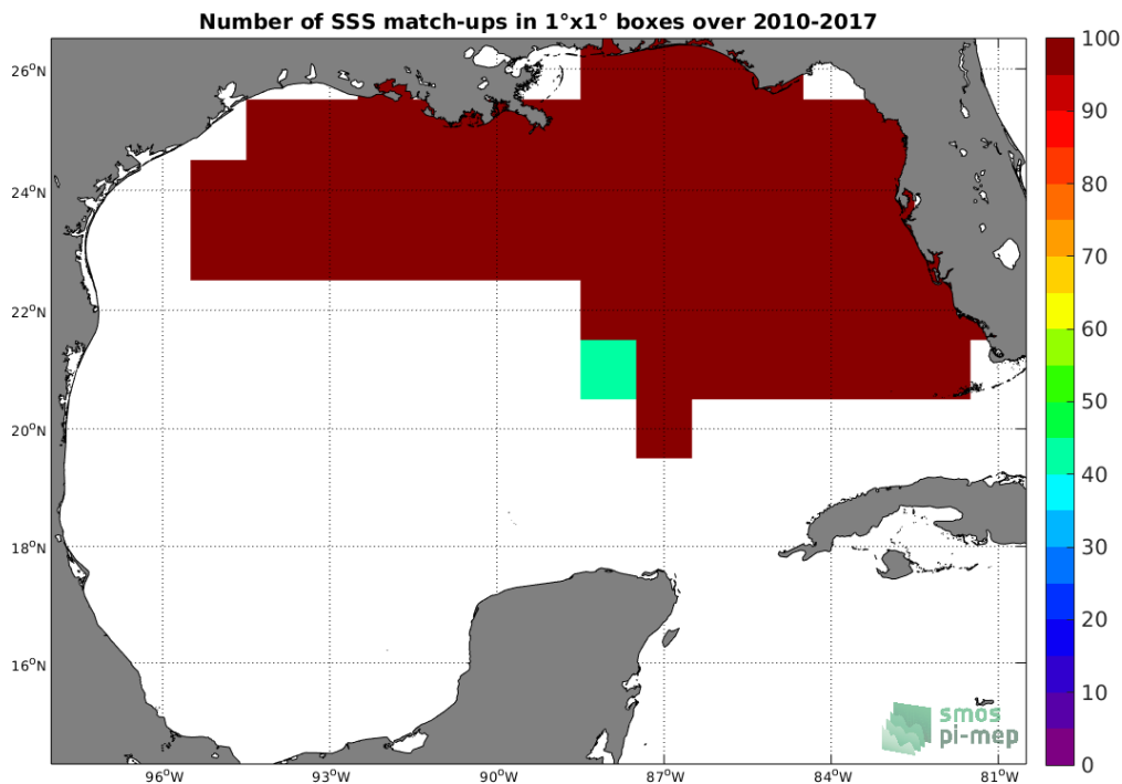
Figure 4: Number of SSS match-ups between TSG (SAMOS) SSS and the SMOS SSS L3 v2 - Daily - 0.5 Deg (CATDS-CECOS-IFREMER) SSS product for the Gulf of Mexico Pi-MEP region over 1^\circ \times 1^\circ boxes and for the full satellite product period.
