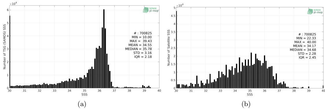
Figure 2: Histograms of SSS from TSG (SAMOS) (a) and SMOS SSS L3 v2 - Daily - 0.5 Deg (CATDS-CECOS-IFREMER) (b) considering all match-up pairs per bins of 0.1 over the Gulf of Mexico Pi-MEP region and for the full satellite product period.
