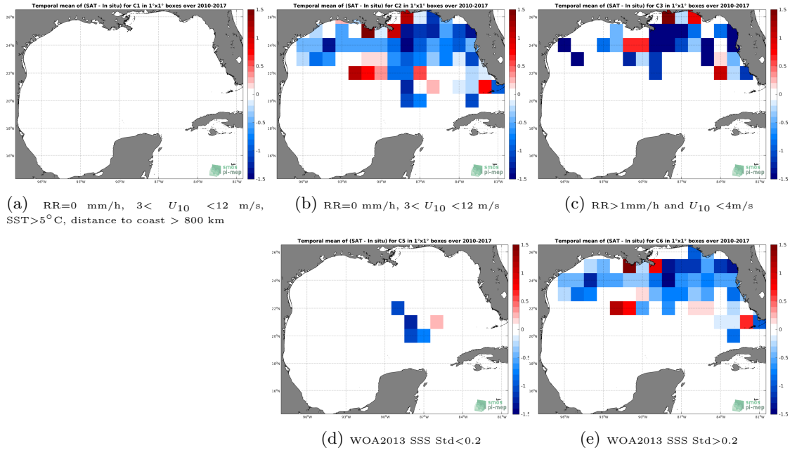
Figure 12: Temporal mean gridded over spatial boxes of size 1^{\circ}\times 1^{\circ} of \Delta\text{SSS} (SMOS SSS L3 v2 - Daily - 0.5 Deg (CATDS-CECOS-IFREMER) - TSG (SAMOS)) for 5 different subdatasets corresponding to:RR=0 mm/h, 3 < U_{10} < 12 m/s, SST >5^{\circ}\text{C} , distance to coast > 800 km (a), RR=0 mm/h, 3 < U_{10} < 12 m/s (b), RR >1 mm/h and U_{10} < 4 m/s (c), WOA2013 SSS Std <0.2 (d), WOA2013 SSS Std >0.2 (e).
