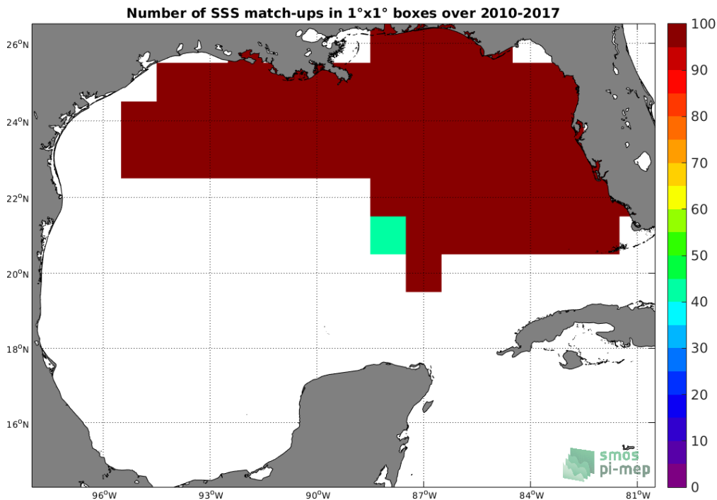
Figure 4: Number of SSS match-ups between TSG-SAMOS SSS and the SMOS L3 v2 - Daily - 0.5 Deg (CATDS-CECOS-IFREMER) SSS product for the Gulf of Mexico Pi-MEP region over 1°x1° boxes and for the full satellite product period.
