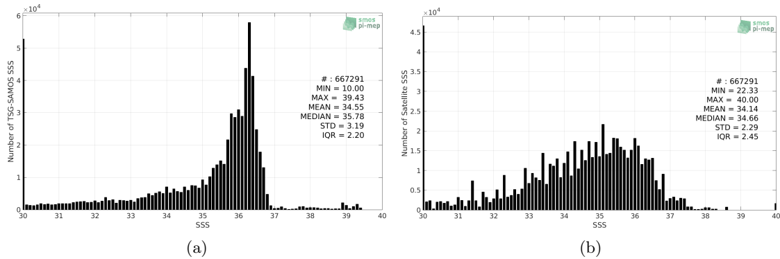
Figure 2: Histograms of SSS from TSG-SAMOS (a) and SMOS L3 v2 - Daily - 0.5 Deg (CATDS-CECOS-IFREMER) (b) considering all match-up pairs per bins of 0.1 over the Gulf of Mexico Pi-MEP region and for the full satellite product period.
