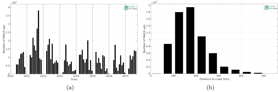
Figure 1: Number of match-ups between TSG-SAMOS and SMOS L3 v2 - Daily - 0.5 Deg (CATDS-CECOS-IFREMER) SSS as a function of time (a) and as function of the distance to coast (b) over the Gulf of Mexico Pi-MEP region and for the full satellite product period.
