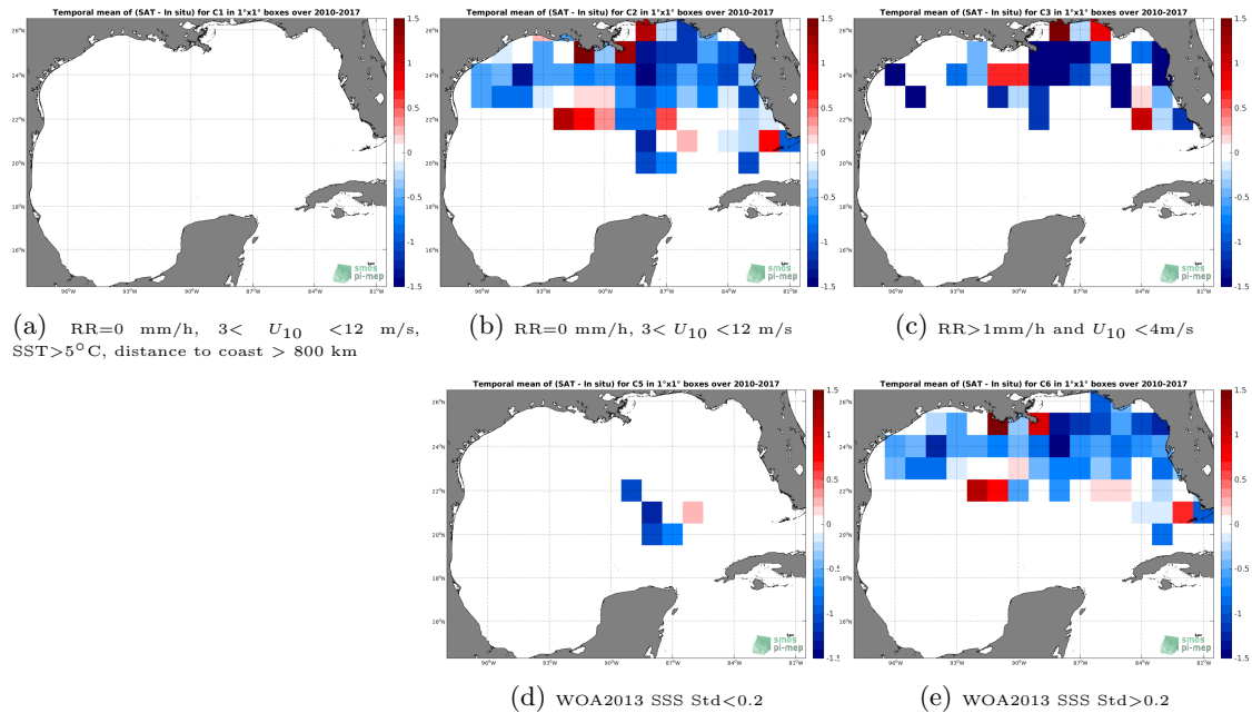
Figure 12: Temporal mean gridded over spatial boxes of size 1^{\circ}\times 1^{\circ} of \Delta\text{SSS} (SMOS L3 v2 - Daily - 0.5 Deg (CATDS-CECOS-IFREMER) - TSG-SAMOS) for 5 different subdatasets corresponding to:RR=0 mm/h, 3 < U_{10} < 12 m/s, SST >5^{\circ}\text{C} , distance to coast > 800 km (a), RR=0 mm/h, 3 < U_{10} < 12 m/s (b), RR >1 mm/h and U_{10} < 4 m/s (c), WOA2013 SSS Std <0.2 (d), WOA2013 SSS Std >0.2 (e).
