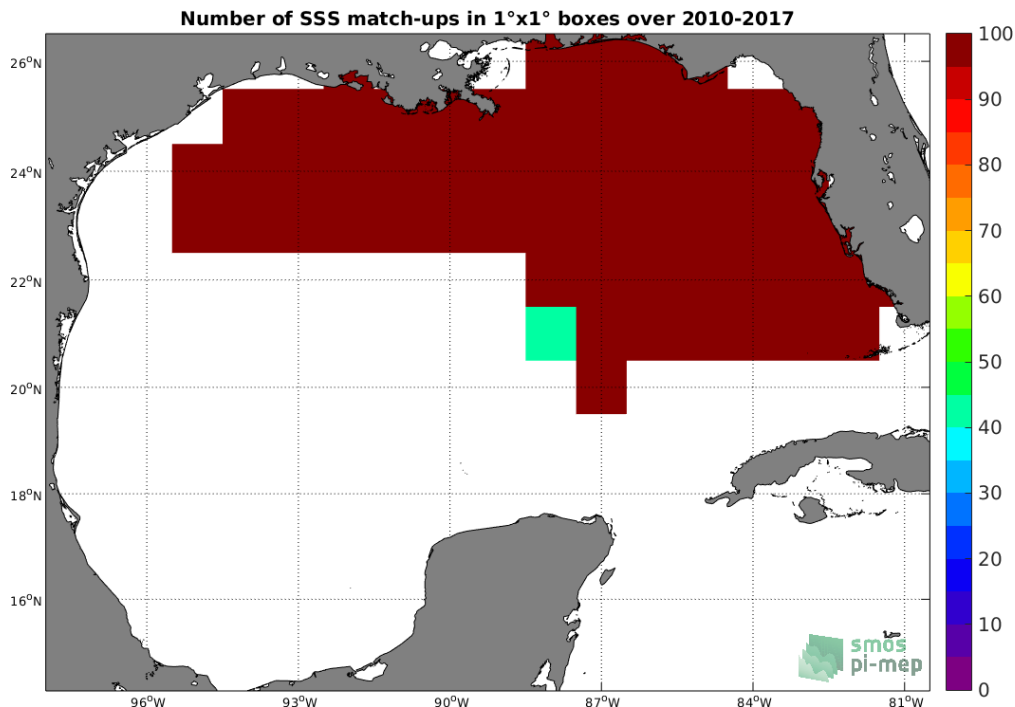
Figure 4: Number of SSS match-ups between TSG-SAMOS SSS and the SMOS-L3-CATDS-CECOS-IFREMER-V2-1DAY-0.5DEG SSS product for the Gulf of Mexico Pi-MEP region over 1°x1° boxes and for the full satellite product period.
