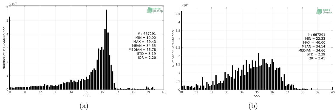
Figure 2: Histograms of SSS from TSG-SAMOS (a) and SMOS-L3-CATDS-CECOS-IFREMER-V2-1DAY-0.5DEG (b) considering all match-up pairs per bins of 0.1 over the Gulf of Mexico Pi-MEP region and for the full satellite product period.
