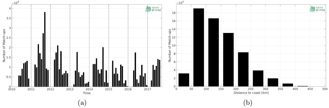
Figure 1: Number of match-ups between TSG-SAMOS and SMOS-L3-CATDS-CECOS-IFREMER-V2-1DAY-0.5DEG SSS as a function of time (a) and as function of the distance to coast (b) over the Gulf of Mexico Pi-MEP region and for the full satellite product period.
