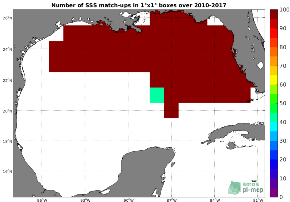
Figure 4: Number of SSS match-ups between TSG-SAMOS SSS and the SMOS-L3-CATDS-CECOS-IFREMER-V2-1DAY-0.5DEG SSS product for the Gulf of Mexico Pi-MEP region over 1^\circ \times 1^\circ boxes and for the full satellite product period.
