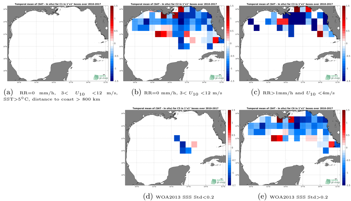
Figure 12: Temporal mean gridded over spatial boxes of size 1^\circ \times 1^\circ of \Delta SSS (SMOS-L3-CATDS-CECOS-IFREMER-V2-1DAY-0.5DEG - TSG-SAMOS) for 5 different subdatasets corresponding to:RR=0 mm/h, 3 < U_{10} < 12 m/s, SST >5^\circ C, distance to coast > 800 km (a), RR=0 mm/h, 3 < U_{10} < 12 m/s (b), RR >1 mm/h and U_{10} < 4 m/s (c), WOA2013 SSS Std <0.2 (d), WOA2013 SSS Std >0.2 (e).
