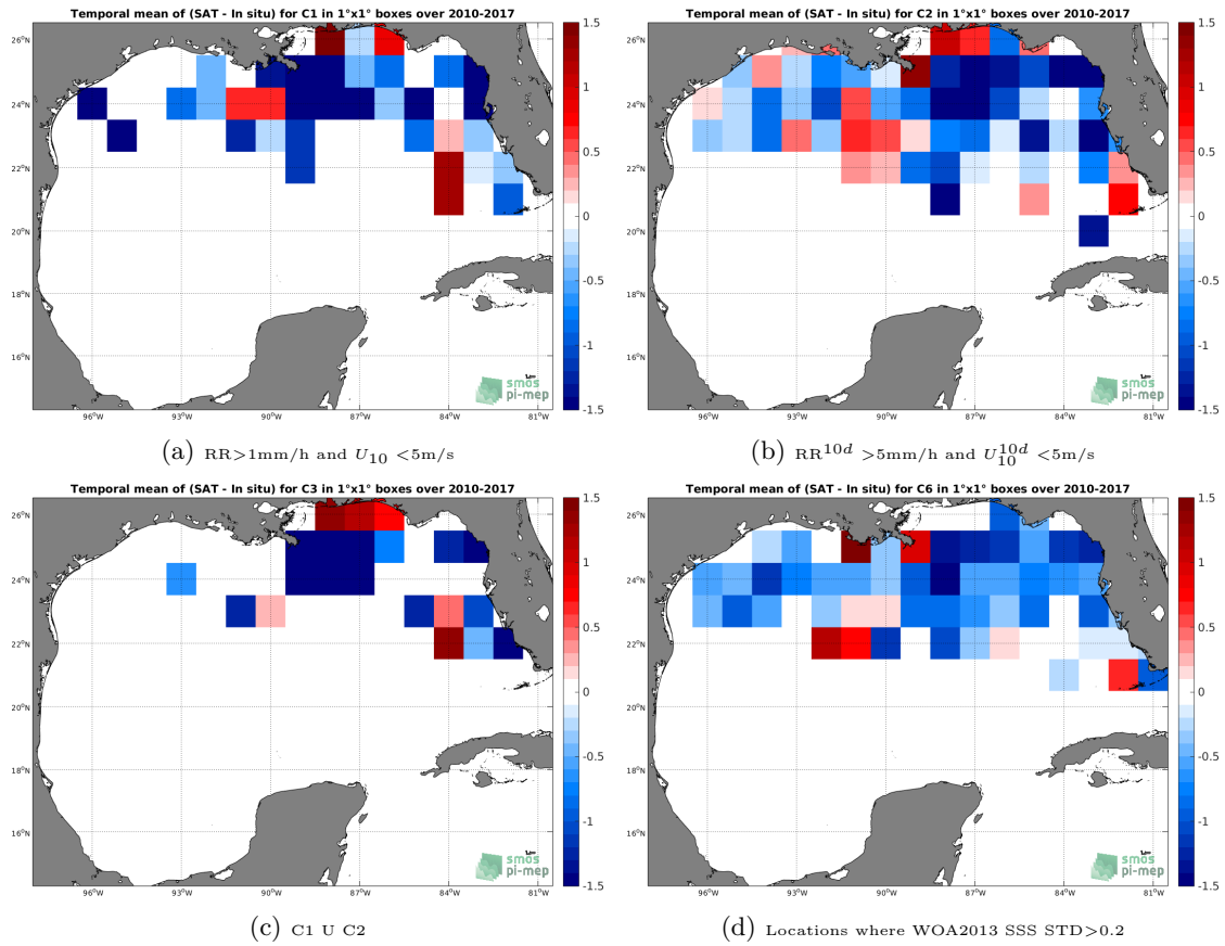
Figure 12: Temporal mean gridded over spatial boxes of size 1^\circ \times 1^\circ of \Delta SSS (SMOS-L3-CATDS-CECOS-IFREMER-V2-1DAY-0.5DEG - TSG-SAMOS) for 4 different subdatasets corresponding to: RR > 1\text{mm/h} and U_{10} < 5\text{m/s} (a), RR^{10d} > 5\text{mm/h} and U_{10}^{10d} < 5\text{m/s} (b), C1 U C2 (c), Locations where WOA2013 SSS STD > 0.2 (d).
