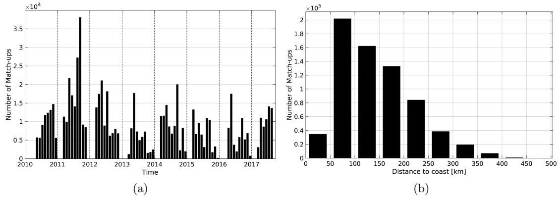
Figure 1: Number of match-ups between TSG-SAMOS and SMOS-L3-CATDS-CECOS-IFREMER-V2-1DAY-0.5DEG SSS as a function of time (a) and as function of the distance to coast (b) over the Gulf of Mexico Pi-MEP region and for the full satellite product period.
