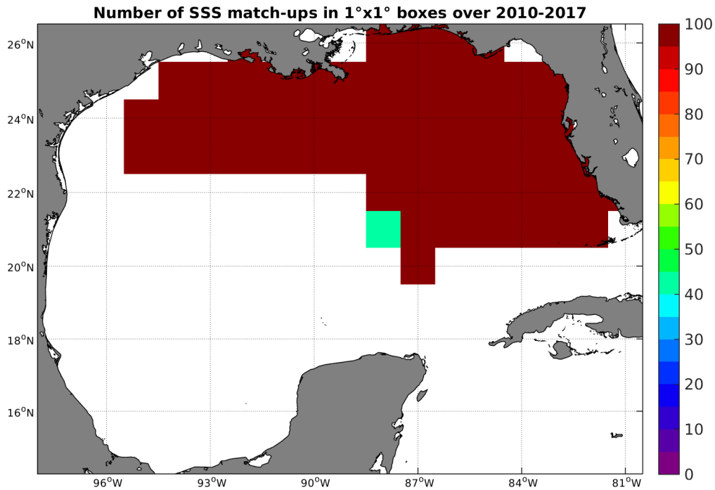
Figure 4: Number of SSS match-ups between TSG-SAMOS SSS and the SMOS-L3-CATDS-CECOS-IFREMER-V2-1DAY-0.5DEG SSS product for the Gulf of Mexico Pi-MEP region over 1^\circ \times 1^\circ boxes and for the full satellite product period.
