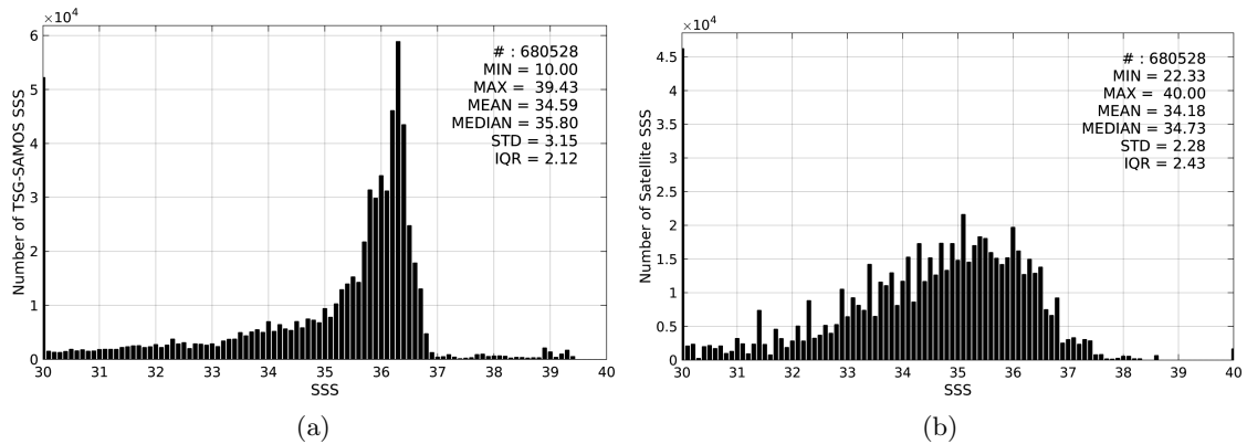
Figure 2: Histograms of SSS from TSG-SAMOS (a) and SMOS-L3-CATDS-CECOS-IFREMER-V2-1DAY-0.5DEG (b) considering all match-up pairs per bins of 0.1 over the Gulf of Mexico Pi-MEP region and for the full satellite product period.
