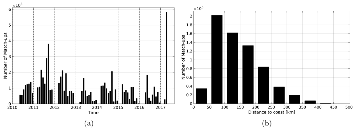
Figure 1: Number of match-ups between TSG-SAMOS and SMOS-L3-CATDS-CECOS-IFREMER-V2-1DAY-0.5deg SSS as a function of time (a) and as function of the distance to coast (b) over the Gulf of Mexico Pi-MEP region and for the full satellite product period.
