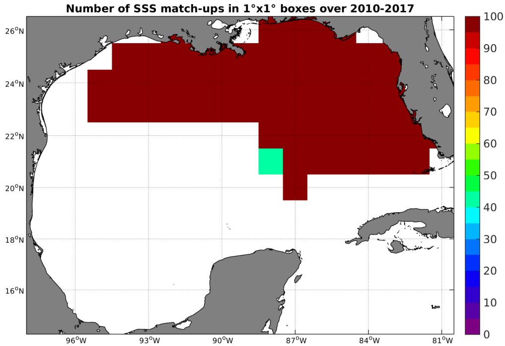
Figure 4: Number of SSS match-ups between TSG-SAMOS SSS and the SMOS-L3-CATDS-CECOS-IFREMER-V2-1DAY-0.5deg SSS product for the Gulf of Mexico Pi-MEP region over 1°x1° boxes and for the full satellite product period.
