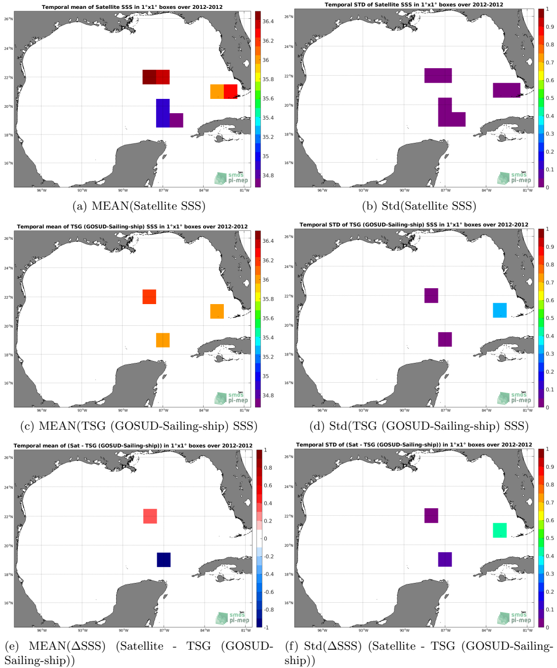
Figure 6: Temporal mean (left) and Std (right) of SSS from SMOS SSS L3 v2 - Daily - 0.5 Deg (CATDS-CECOS-IFREMER) (top), TSG (GOSUD-Sailing-ship) (middle), and of \Delta SSS (Satellite - TSG (GOSUD-Sailing-ship)). Only match-up pairs are used to generate these maps.
