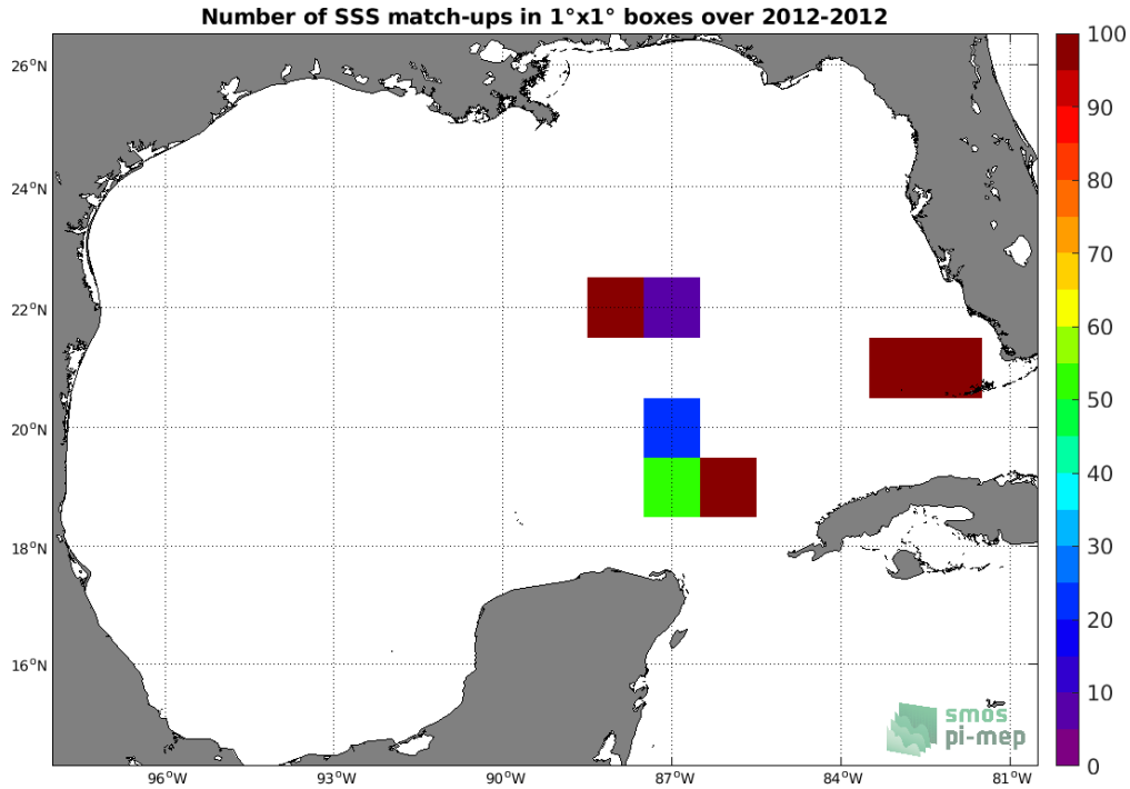
Figure 4: Number of SSS match-ups between TSG (GOSUD-Sailing-ship) SSS and the SMOS SSS L3 v2 - Daily - 0.5 Deg (CATDS-CECOS-IFREMER) SSS product for the Gulf of Mexico Pi-MEP region over 1°x1° boxes and for the full satellite product period.
