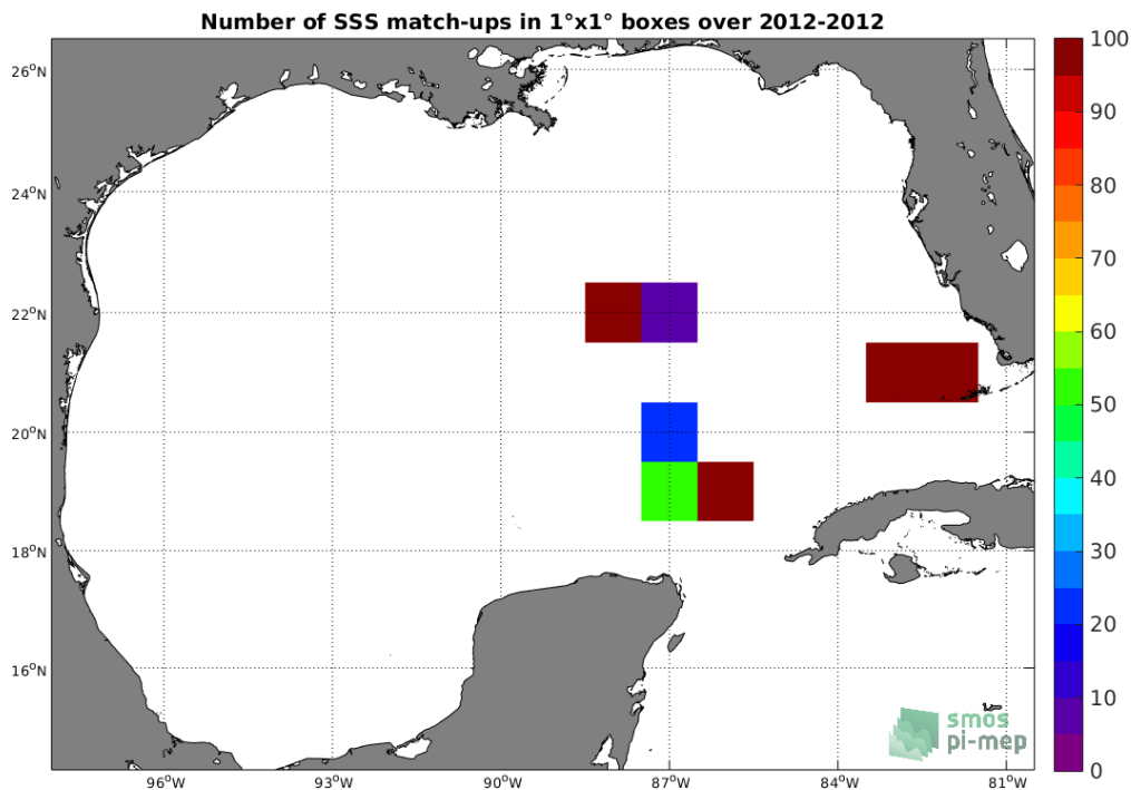
Figure 4: Number of SSS match-ups between TSG (GOSUD-Sailing-ship) SSS and the SMOS SSS L3 v2 - Daily - 0.5 Deg (CATDS-CECOS-IFREMER) SSS product for the Gulf of Mexico Pi-MEP region over 1^\circ \times 1^\circ boxes and for the full satellite product period.
