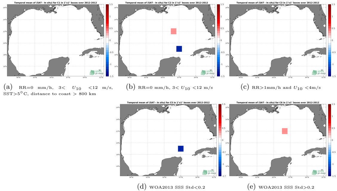
Figure 12: Temporal mean gridded over spatial boxes of size 1^\circ \times 1^\circ of \Delta SSS (SMOS SSS L3 v2 - Daily - 0.5 Deg (CATDS-CECOS-IFREMER) - TSG (GOSUD-Sailing-ship)) for 5 different subdatasets corresponding to:RR=0 mm/h, 3 < U_{10} < 12 m/s, SST >5^\circ\text{C} , distance to coast > 800 km (a), RR=0 mm/h, 3 < U_{10} < 12 m/s (b), RR >1 mm/h and U_{10} < 4 m/s (c), WOA2013 SSS Std <0.2 (d), WOA2013 SSS Std >0.2 (e).
