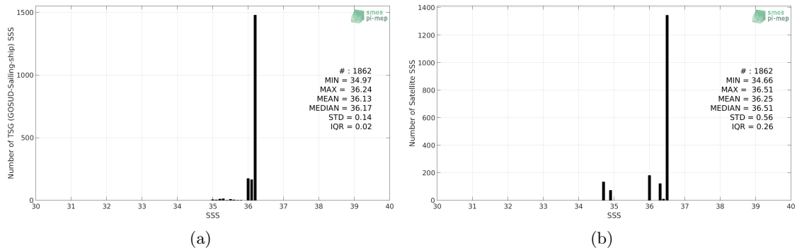
Figure 2: Histograms of SSS from TSG (GOSUD-Sailing-ship) (a) and SMOS SSS L3 v2 - Daily - 0.5 Deg (CATDS-CECOS-IFREMER) (b) considering all match-up pairs per bins of 0.1 over the Gulf of Mexico Pi-MEP region and for the full satellite product period.
