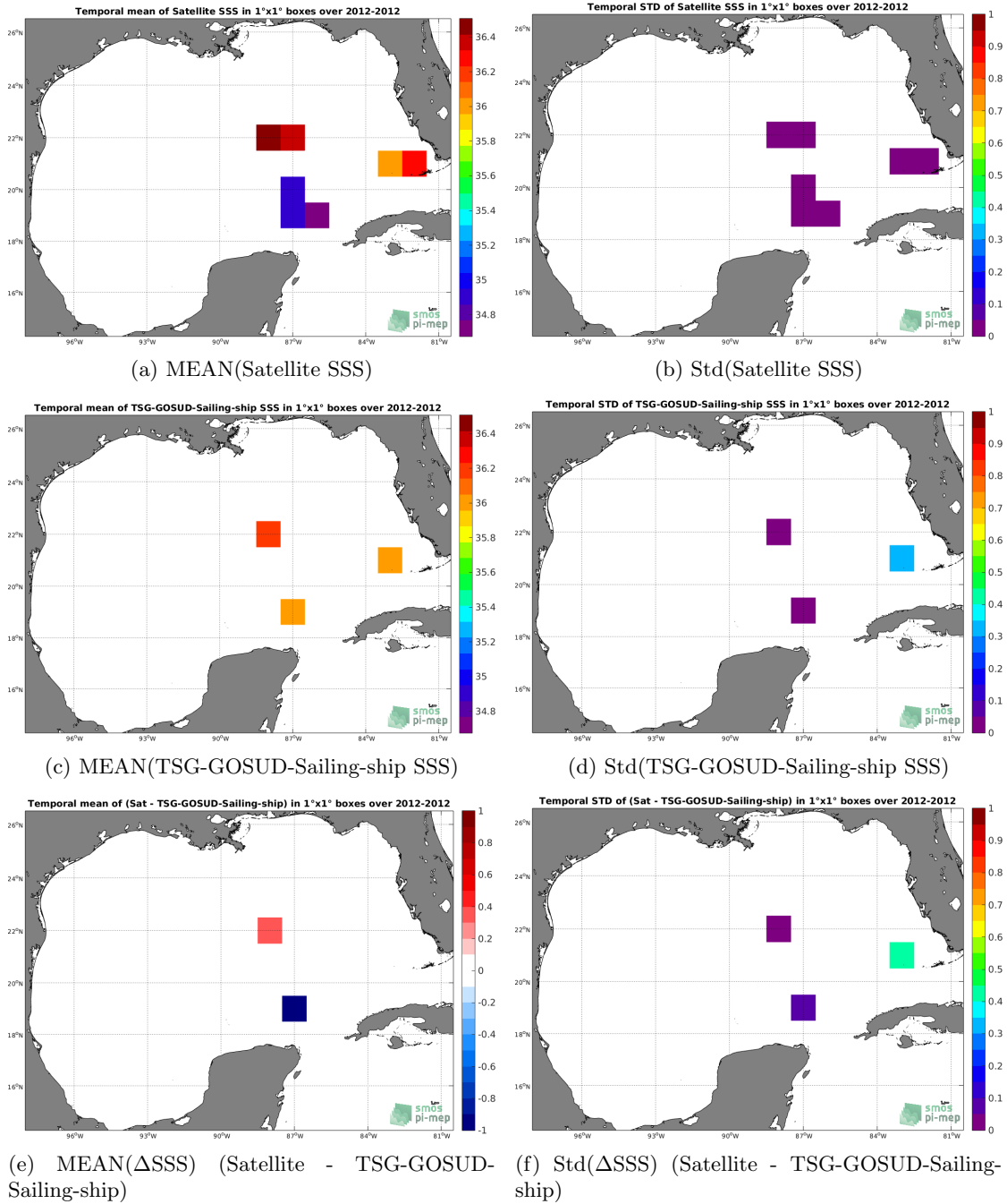
Figure 6: Temporal mean (left) and Std (right) of SSS from SMOS L3 v2 - Daily - 0.5 Deg (CATDS-CECOS-IFREMER) (top), TSG-GOSUD-Sailing-ship (middle), and of \Delta SSS (Satellite - TSG-GOSUD-Sailing-ship). Only match-up pairs are used to generate these maps.
