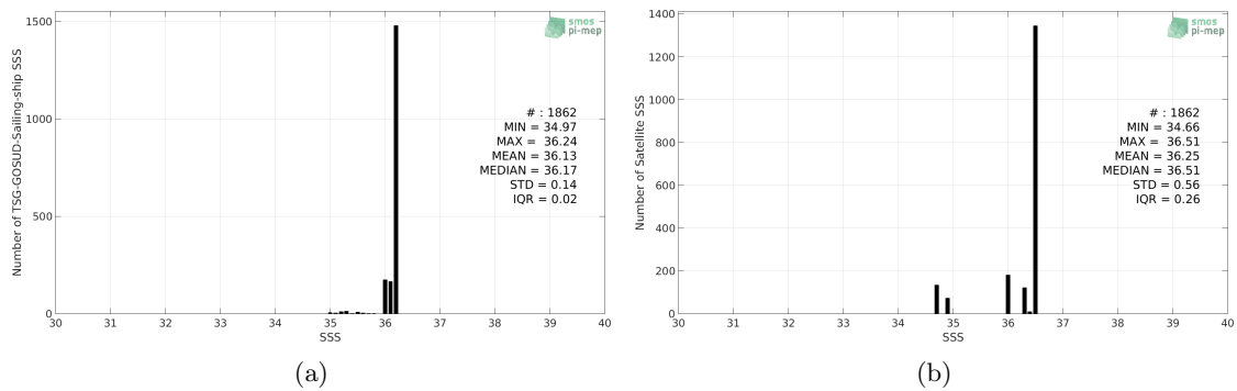
Figure 2: Histograms of SSS from TSG-GOSUD-Sailing-ship (a) and SMOS L3 v2 - Daily - 0.5 Deg (CATDS-CECOS-IFREMER) (b) considering all match-up pairs per bins of 0.1 over the Gulf of Mexico Pi-MEP region and for the full satellite product period.
