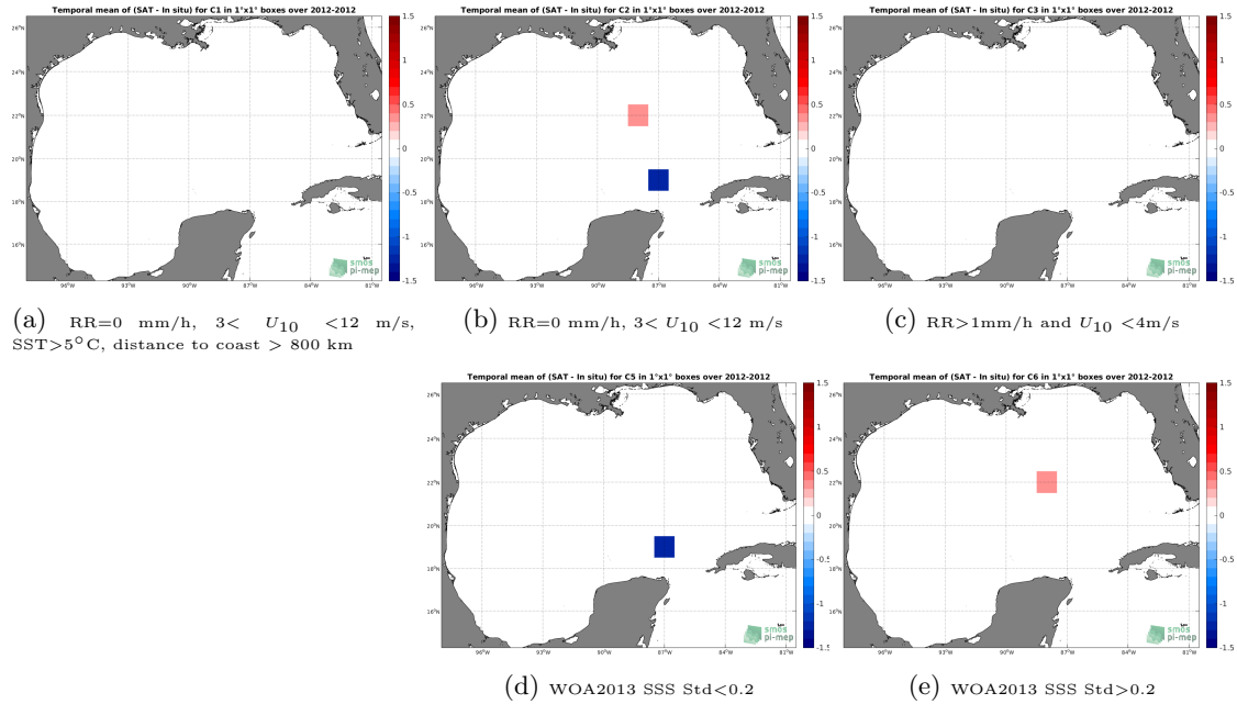
Figure 12: Temporal mean gridded over spatial boxes of size 1^{\circ}\times 1^{\circ} of \Delta SSS (SMOS L3 v2 - Daily - 0.5 Deg (CATDS-CECOS-IFREMER) - TSG-GOSUD-Sailing-ship) for 5 different subdatasets corresponding to:RR=0 mm/h, 3 < U_{10} < 12 m/s, SST >5^{\circ}\text{C} , distance to coast > 800 km (a), RR=0 mm/h, 3 < U_{10} < 12 m/s (b), RR >1 mm/h and U_{10} < 4 m/s (c), WOA2013 SSS Std <0.2 (d), WOA2013 SSS Std >0.2 (e).
