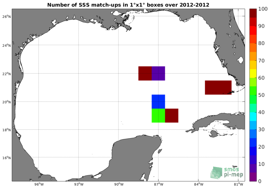
Figure 4: Number of SSS match-ups between TSG-GOSUD-Sailing-ship SSS and the SMOS L3 v2 - Daily - 0.5 Deg (CATDS-CECOS-IFREMER) SSS product for the Gulf of Mexico Pi-MEP region over 1^\circ \times 1^\circ boxes and for the full satellite product period.
