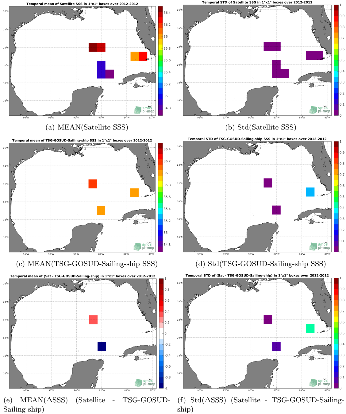
Figure 6: Temporal mean (left) and Std (right) of SSS from SMOS-L3-CATDS-CECOS-IFREMER-V2-1DAY-0.5DEG (top), TSG-GOSUD-Sailing-ship (middle), and of \Delta SSS (Satellite - TSG-GOSUD-Sailing-ship). Only match-up pairs are used to generate these maps.
