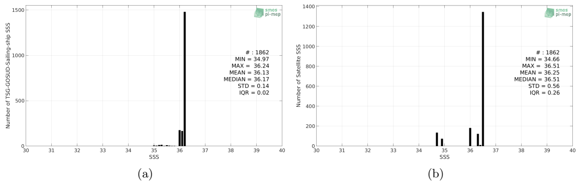
Figure 2: Histograms of SSS from TSG-GOSUD-Sailing-ship (a) and SMOS-L3-CATDS-CECOS-IFREMER-V2-1DAY-0.5DEG (b) considering all match-up pairs per bins of 0.1 over the Gulf of Mexico Pi-MEP region and for the full satellite product period.
