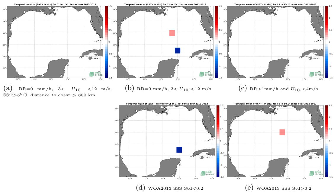
Figure 12: Temporal mean gridded over spatial boxes of size 1^\circ \times 1^\circ of \Delta SSS (SMOS-L3-CATDS-CECOS-IFREMER-V2-1DAY-0.5DEG - TSG-GOSUD-Sailing-ship) for 5 different subdatasets corresponding to:RR=0 mm/h, 3 < U_{10} < 12 m/s, SST >5^\circ\text{C} , distance to coast > 800 km (a), RR=0 mm/h, 3 < U_{10} < 12 m/s (b), RR >1 mm/h and U_{10} < 4 m/s (c), WOA2013 SSS Std <0.2 (d), WOA2013 SSS Std >0.2 (e).
