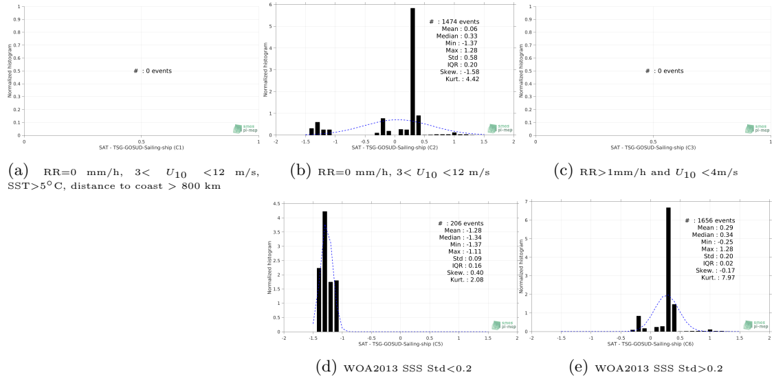
Figure 13: Normalized histogram of \Delta\text{SSS} (SMOS-L3-CATDS-CECOS-IFREMER-V2-1DAY-0.5DEG - TSG-GOSUD-Sailing-ship) for 5 different subdatasets corresponding to: RR=0 mm/h, 3 < U_{10} < 12 m/s, SST > 5^\circ\text{C} , distance to coast > 800 km (a), RR=0 mm/h, 3 < U_{10} < 12 m/s (b), RR > 1\text{mm/h} and U_{10} < 4\text{m/s} (c), WOA2013 SSS Std < 0.2 (d), WOA2013 SSS Std > 0.2 (e).
