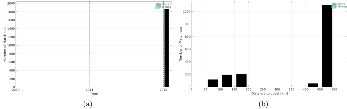
Figure 1: Number of match-ups between TSG-GOSUD-Sailing-ship and SMOS-L3-CATDS-CECOS-IFREMER-V2-1DAY-0.5DEG SSS as a function of time (a) and as function of the distance to coast (b) over the Gulf of Mexico Pi-MEP region and for the full satellite product period.
