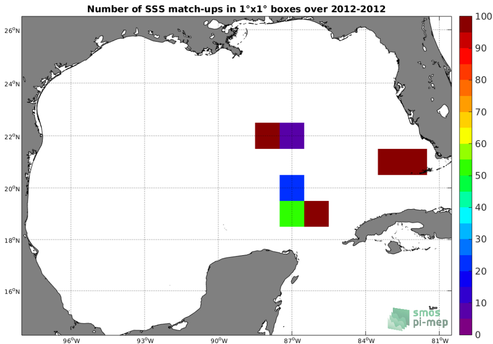
Figure 4: Number of SSS match-ups between TSG-GOSUD-Sailing-ship SSS and the SMOS-L3-CATDS-CECOS-IFREMER-V2-1DAY-0.5DEG SSS product for the Gulf of Mexico Pi-MEP region over 1°x1° boxes and for the full satellite product period.
