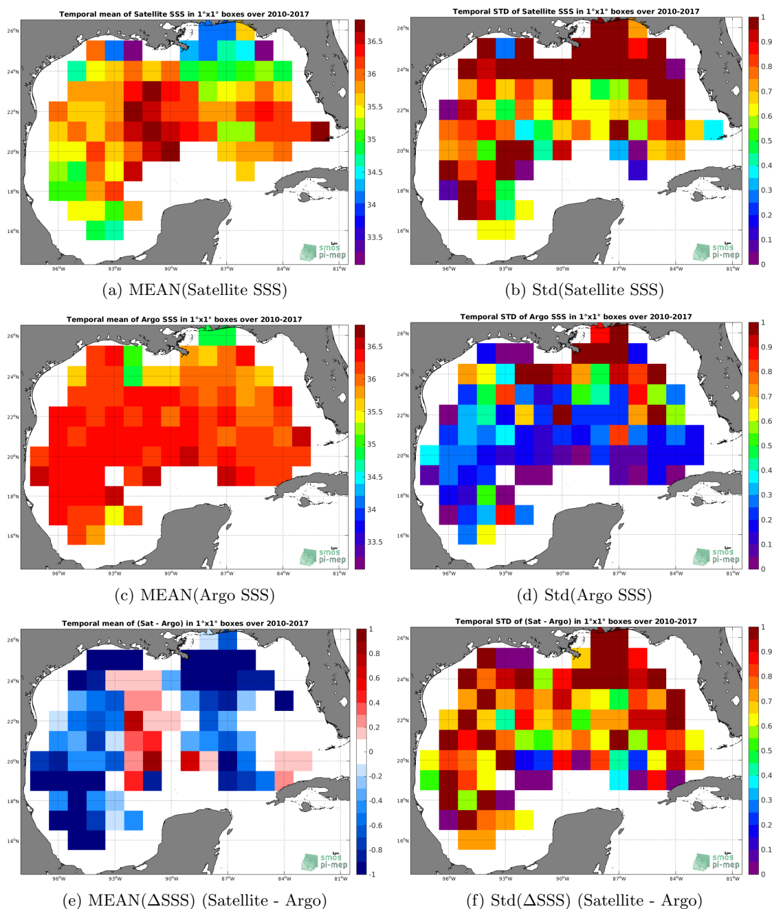
Figure 6: Temporal mean (left) and Std (right) of SSS from SMOS L3 v2 - Daily - 0.5 Deg (CATDS-CECOS-IFREMER) (top), Argo (middle), and of \Delta SSS (Satellite - Argo). Only match-up pairs are used to generate these maps.
