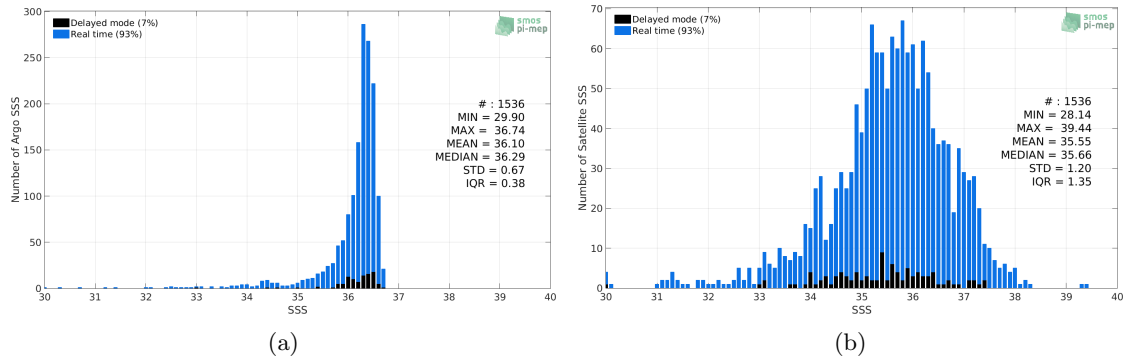
Figure 2: Histograms of SSS from Argo (a) and SMOS L3 v2 - Daily - 0.5 Deg (CATDS-CECOS-IFREMER) (b) considering all match-up pairs per bins of 0.1 over the Gulf of Mexico Pi-MEP region and for the full satellite product period.
