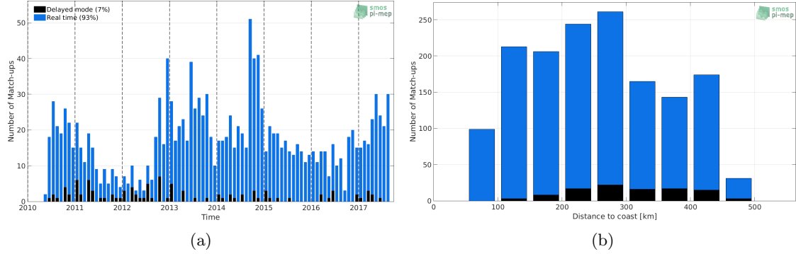
Figure 1: Number of match-ups between Argo and SMOS L3 v2 - Daily - 0.5 Deg (CATDS-CECOS-IFREMER) SSS as a function of time (a) and as function of the distance to coast (b) over the Gulf of Mexico Pi-MEP region and for the full satellite product period.
