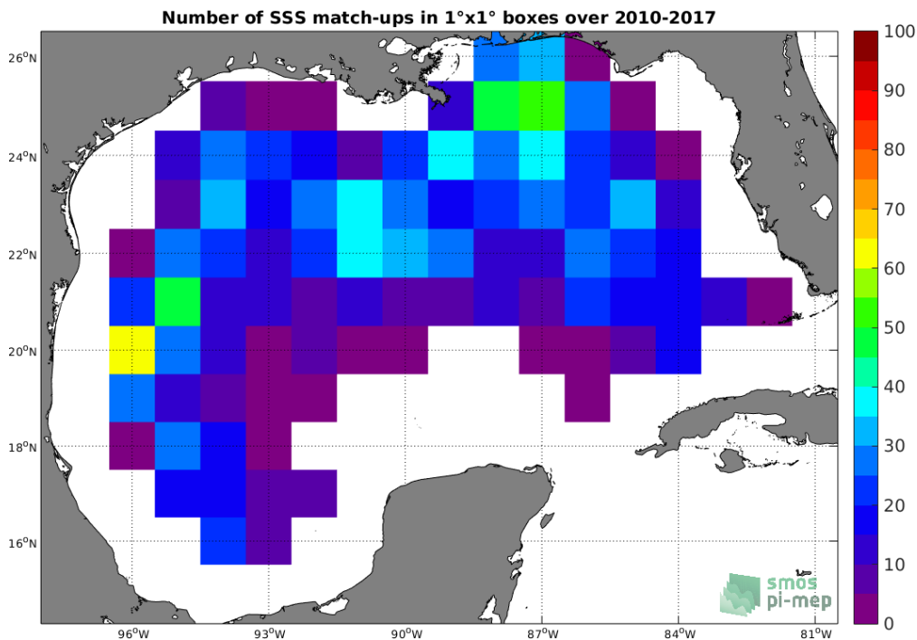
Figure 4: Number of SSS match-ups between Argo SSS and the SMOS L3 v2 - Daily - 0.5 Deg (CATDS-CECOS-IFREMER) SSS product for the Gulf of Mexico Pi-MEP region over 1°x1° boxes and for the full satellite product period.
