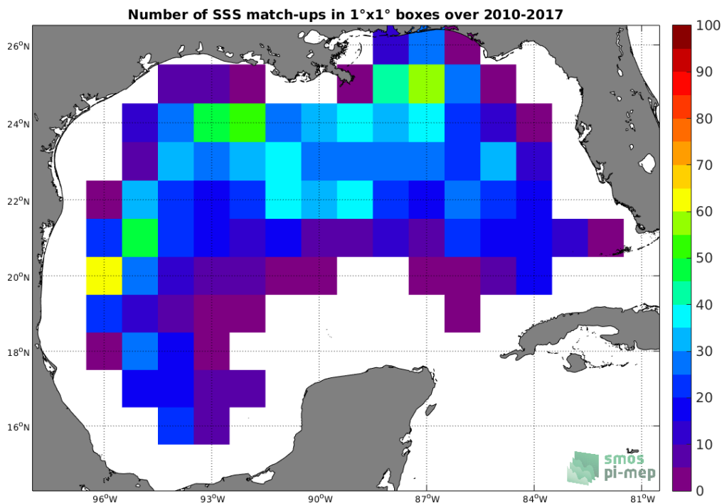
Figure 4: Number of SSS match-ups between Argo SSS and the SMOS-L3-CATDS-CECOS-IFREMER-V2-1DAY-0.5DEG SSS product for the Gulf of Mexico Pi-MEP region over 1^\circ \times 1^\circ boxes and for the full satellite product period.
