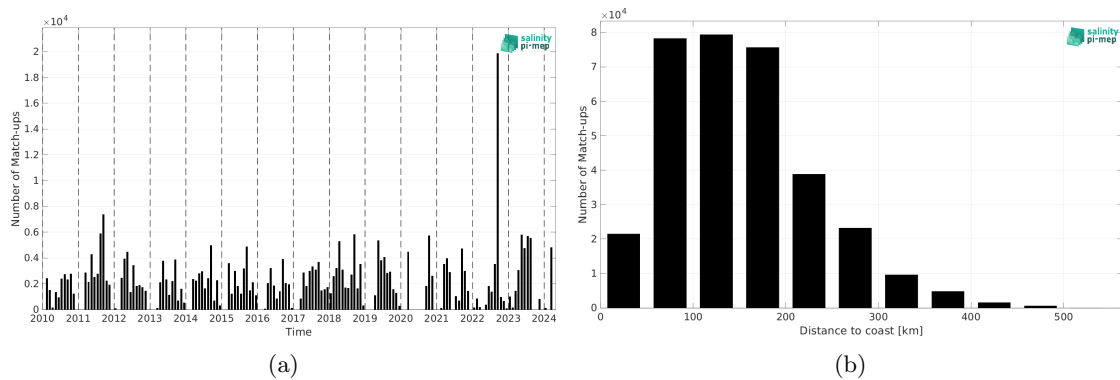
Figure 2: Number of match-ups between TSG (SAMOS) and SMOS SSS L3 v335 - Monthly - 25 km (CATDS-CPDC) SSS as a function of time (a) and as function of the distance to coast (b) over the Gulf of Mexico Pi-MEP region and for the full satellite product period.
