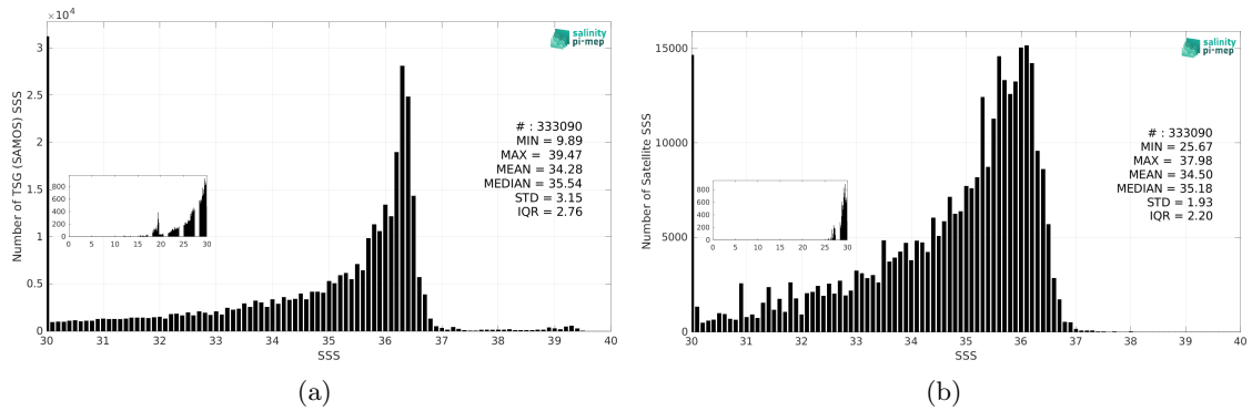
Figure 3: Histograms of SSS from TSG (SAMOS) (a) and SMOS SSS L3 v335 - Monthly - 25 km (CATDS-CPDC) (b) considering all match-up pairs per bins of 0.1 over the Gulf of Mexico Pi-MEP region and for the full satellite product period.
