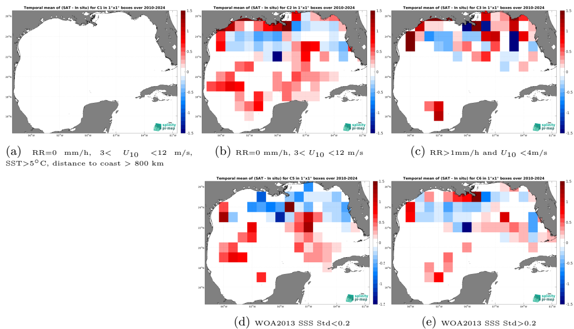
Figure 14: Temporal mean gridded over spatial boxes of size 1^\circ \times 1^\circ of \Delta\text{SSS} (SMOS SSS L3 v335 - Monthly - 25 km (CATDS-CPDC) - TSG (SAMOS)) for 5 different subdatasets corresponding to:RR=0 mm/h, 3 < U_{10} < 12 m/s, SST >5^\circ\text{C} , distance to coast > 800 km (a), RR=0 mm/h, 3 < U_{10} < 12 m/s (b), RR >1 mm/h and U_{10} < 4 m/s (c), WOA2013 SSS Std <0.2 (d), WOA2013 SSS Std >0.2 (e).
