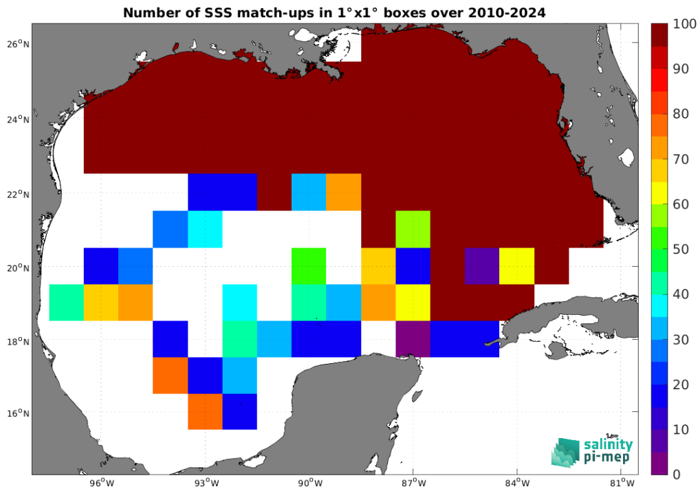
Figure 5: Number of SSS match-ups between TSG (SAMOS) SSS and the SMOS SSS L3 v335 - Monthly - 25 km (CATDS-CPDC) SSS product for the Gulf of Mexico Pi-MEP region over 1^\circ \times 1^\circ boxes and for the full satellite product period.
